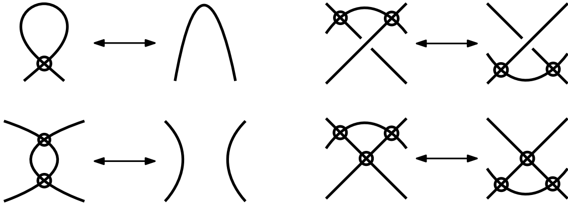
Figure 3.2: The non-classical moves making up the virtual Reidemeister moves. Anti-clockwise from the top left: virtual Reidemeister 1, virtual Reidemeister 2, virtual Reidemeister 3, and the mixed move.
