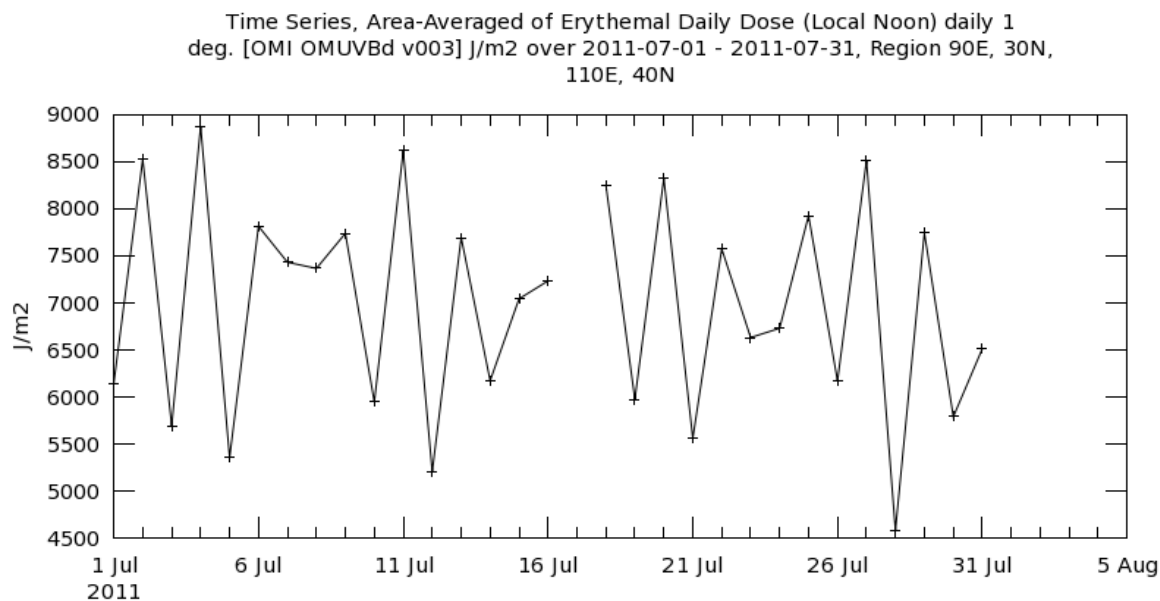
Supplementary Figure 1. Time series of area-averaged source region erythemal daily dose date through July 2011 illustrating peak surface UV-B radiation on July 4 th . Produced using Nasa Giovanni environment (Data source, Hovila et al., 2013 108 ).
