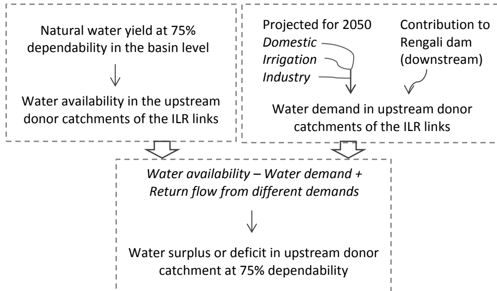
Figure 7.9: Water balance assessment process followed by (NWDA 2009a; 2009b)
