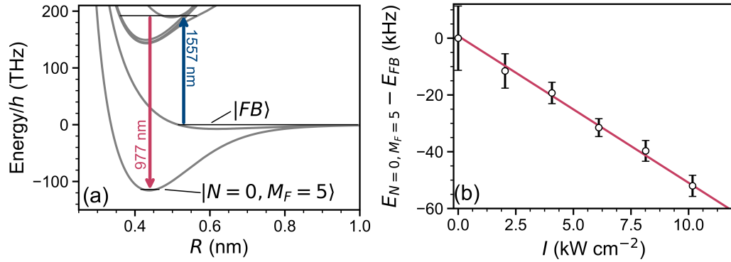
Figure 6.5: Measurement of the isotropic component \alpha^{(0)} with spectroscopy. (a) Transitions used in STIRAP of molecules to the lowest hyperfine sublevel of the rovibronic ground state. (b) AC Stark shift of the STIRAP dark-state resonance.
