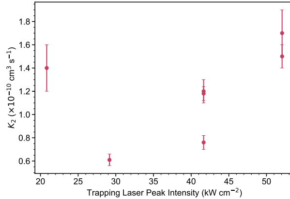
Figure 7.3: Dependence of two-body molecule loss rate K_2 on the intensity of the trapping laser. Error bars shown are those found during the fitting of the results. The real uncertainty in loss rate is likely significantly higher.
