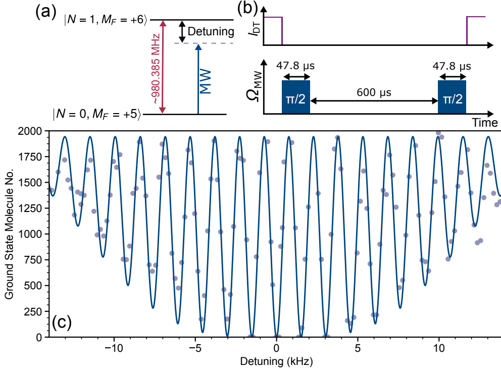
Figure 5.12: Ramsey interferometry between the two lowest hyperfine states of the N=0 and N=1 rotational levels of ^{87}\text{Rb}^{133}\text{Cs} in free-space. (a) The relevant hyperfine levels in ^{87}\text{Rb}^{133}\text{Cs} . We vary the detuning of the microwaves from the on-resonance transition frequency. (b) The relevant timings for the observation of kHz separated Ramsey fringes. The two microwave pulses are set such that they each drive a \pi/2 pulse when on resonance. The duration of 47.8 \mu\text{s} corresponds to a Rabi frequency of \Omega/2\pi = 5.2(1) kHz. The pulses are separated by a free-space evolution time of 600 \mu\text{s} . (c) By varying the frequency of both microwave pulses, Ramsey fringes separated by \sim 1.5 kHz are observed. Each point is the result of a single run of the experiment, the solid blue line is a least-squares fit to the data using Eq. 5.1 with two free parameters: the centre frequency and the peak number of molecules.
