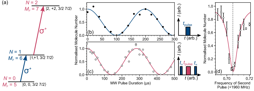
Figure 5.7: Two-step transfer between the spin-stretched and lowest energy hyperfine levels of N = 0, 1 and 2 . (a) Transfer scheme followed in this work. All molecules start in the lowest hyperfine state ( M_F = 5 ) of N = 0 . States are described in the uncoupled basis set |N, M_N, m_I^{\text{Rb}}, m_I^{\text{Cs}}\rangle . (b) Rabi oscillations in one-photon transfer of molecules to the spin-stretched M_F = 6 state of N = 1 shown in (a). (c) Rabi oscillations in two-photon transfer, using a \pi -pulse on the first transition and a second microwave pulse with different frequency to drive a second transition to the M_F = 7 hyperfine level of N = 2 shown in (a). (d) Effect of scanning the frequency of the second microwave pulse with duration < t_\pi . The dashed grey line shows the expected transition frequency given the molecular constants fitted to the N = 1 spectroscopy.
