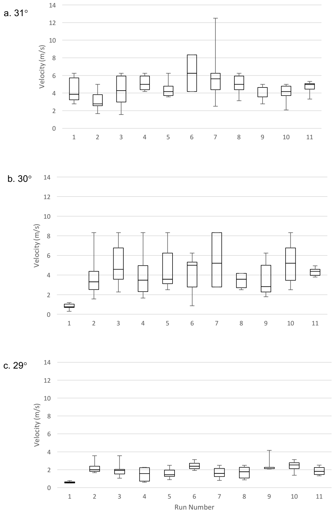
Figure 3.6. Boxplots of debris-flow velocity (between 6 and 8 m downslope) for different slope angles: (a) 31^\circ , (b) 30^\circ , and (c) 29^\circ , with 11 replicate experiments.
