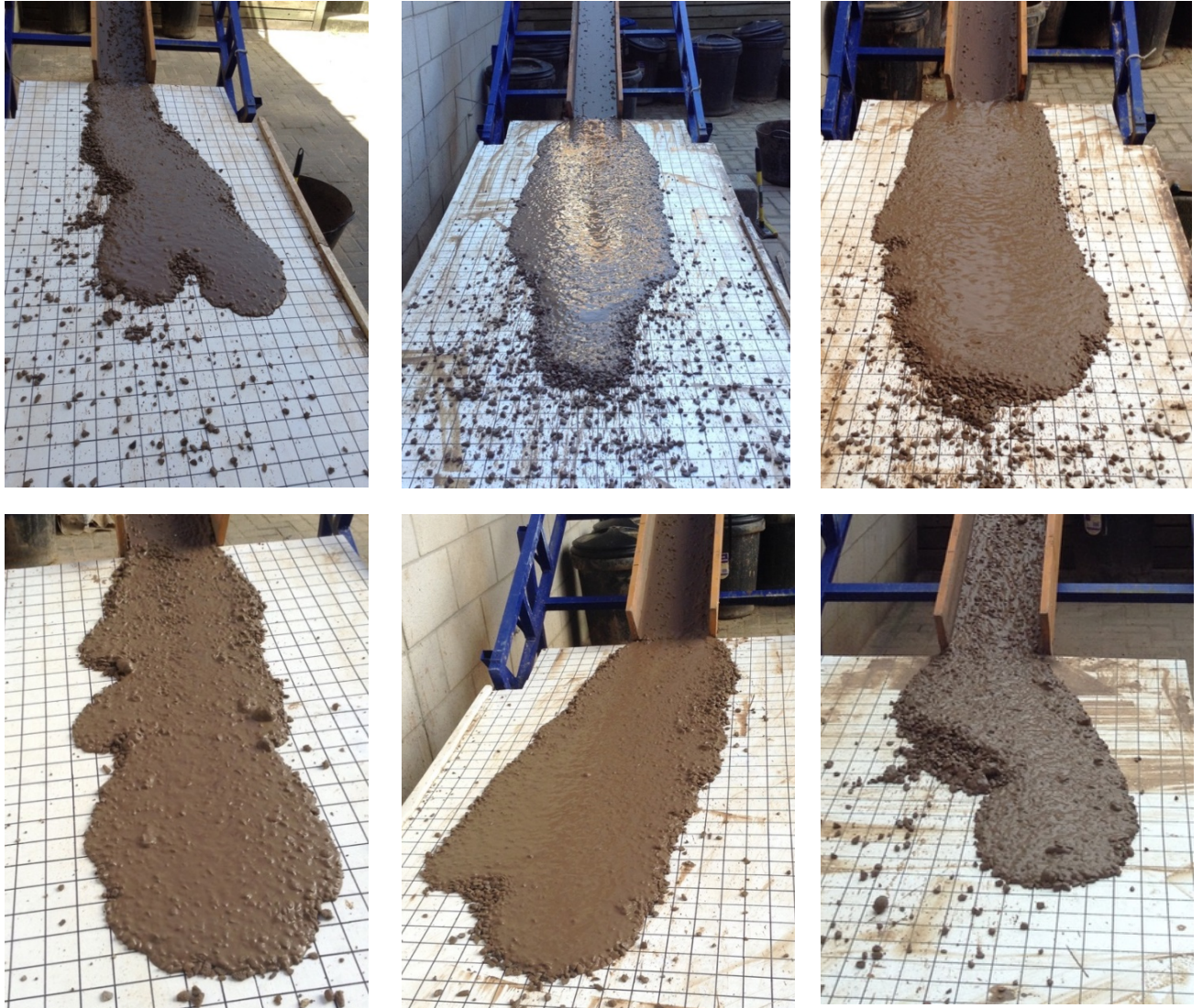
Figure 3.10. Examples of debris flow deposits, showing the varied deposit shapes produced.
