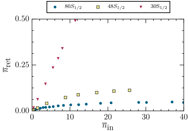
Figure 4.21.: Saturation of photon storage/retrieval due to dipole interactions. Photon retrieval rate \bar{n}_{ret} as a function of incoming photon number \bar{n}_{in} for three Rydberg states.
