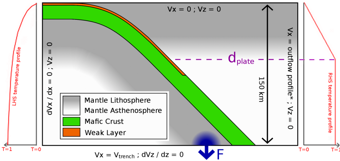
Figure 5.1 Schematic representation of the model setup with thermal and mechanical boundary conditions. Green area marks the position of crustal material and is given a thickness d_{crust} , the location of the weak zone (see main text for further details) is depicted in orange, and the overriding plate is defined to extend down to d_{plate} . The artificial slab pull force F is applied over an area within the slab mantle which is free to move laterally (indicated in blue). V_{trench} is applied to the bottom boundary to mimic the effect trench migration has on the subduction geometry
