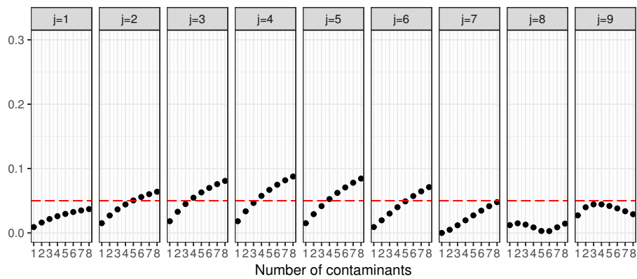
Figure 5.7: SC_{P(X_{(2)} \in I_i)}(\underline{x}, y_1, \dots, y_l) for n = 8 and m = 3 .
