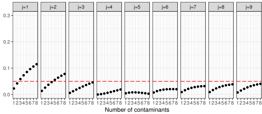
Figure 5.6: SC_{P(X_{(1)} \in I_i)}(\underline{x}, y_1, \dots, y_l) for n = 8 and m = 3 .
