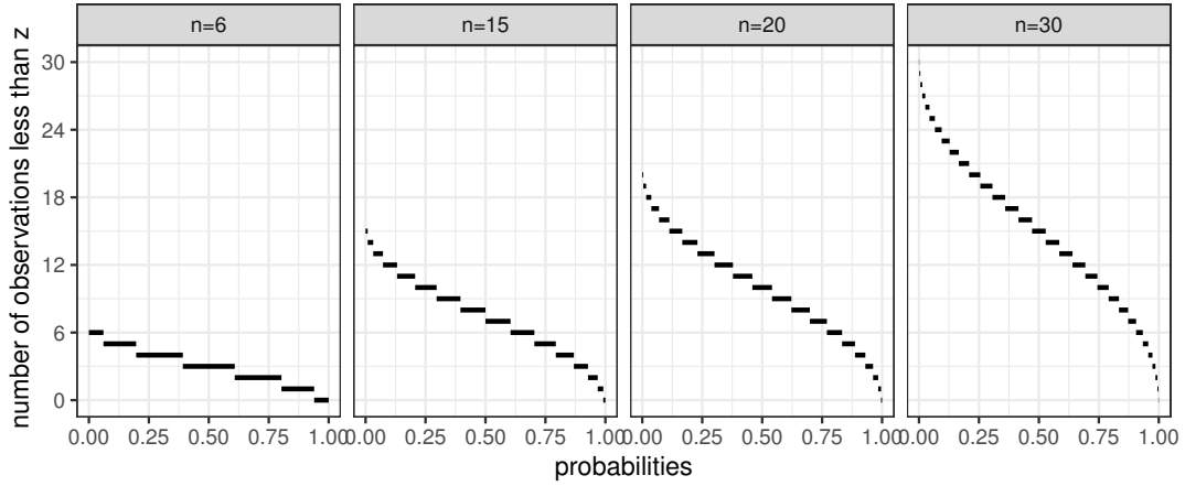
Figure 2.5: [\underline{P}, \overline{P}](M_m > z) for m = 5 and n = 6, 15, 20, 30 .
