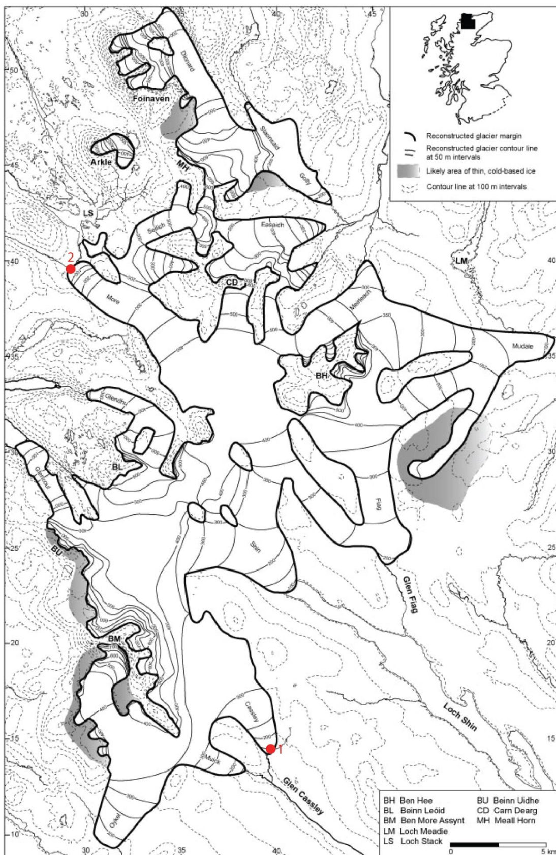
Figure 3.9 Three-dimensional reconstruction of the mountain icefield in the Ben Hee area. Chronological sites discussed in the text are indicated by the red dots. Adapted from Journal of Quaternary Science, Vol. 25(4), Lukas, S. and Bradwell, T., Reconstruction of a Lateglacial (Younger Dryas) mountain ice field in Sutherland, northwestern Scotland, and its palaeoclimatic implications, 567-580, Copyright (2010), with permission from John Wiley and Sons.
