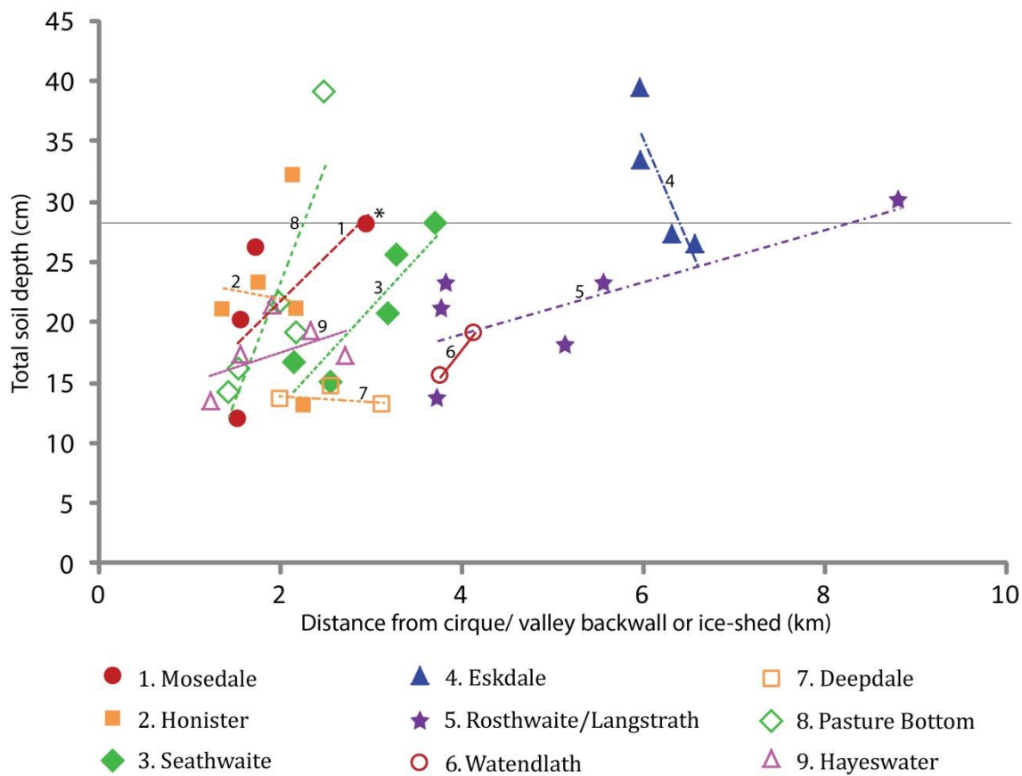
Figure 5.13 Total soil depth against distance from the cirque backwall or ice-shed. Linear trendlines show that total soil depth generally increases with distance from the backwall but there are some exceptions where the pits sampled are closely spaced along the former glacier flowline. The horizontal grey line represents the total soil thickness at site MD1, which has been assigned a pre-LLS age based on its location down-valley of a Lateglacial coring site.
