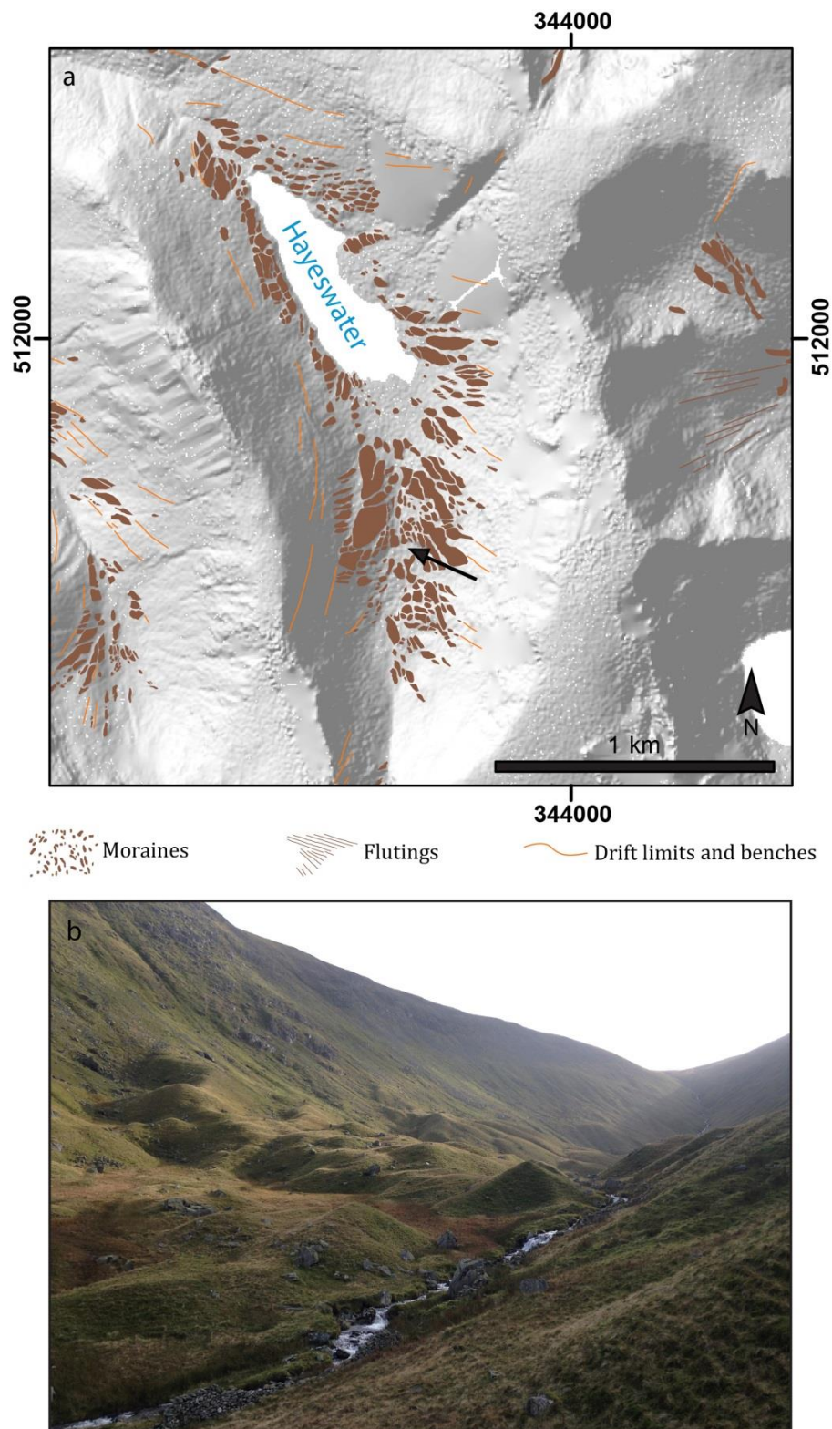
Figure 3.25 a) Sharp-crested recessional moraines at Hayeswater (after McDougall, 2013). At the valley head the moraines show glacier retreat back onto the plateau, refuting the alpine style of glaciation Sissons (1980a) proposed for this site. Figure 3.25b was taken looking south from the point indicated by the arrow. The hill-shaded image derived from NEXTMap DSM from Intermap Technologies Inc. provided by the NERC Earth Observation Data Centre. b) Hummocky moraines at the head of Hayeswater valley looking north. Photograph from H.L. Bickerdike.
