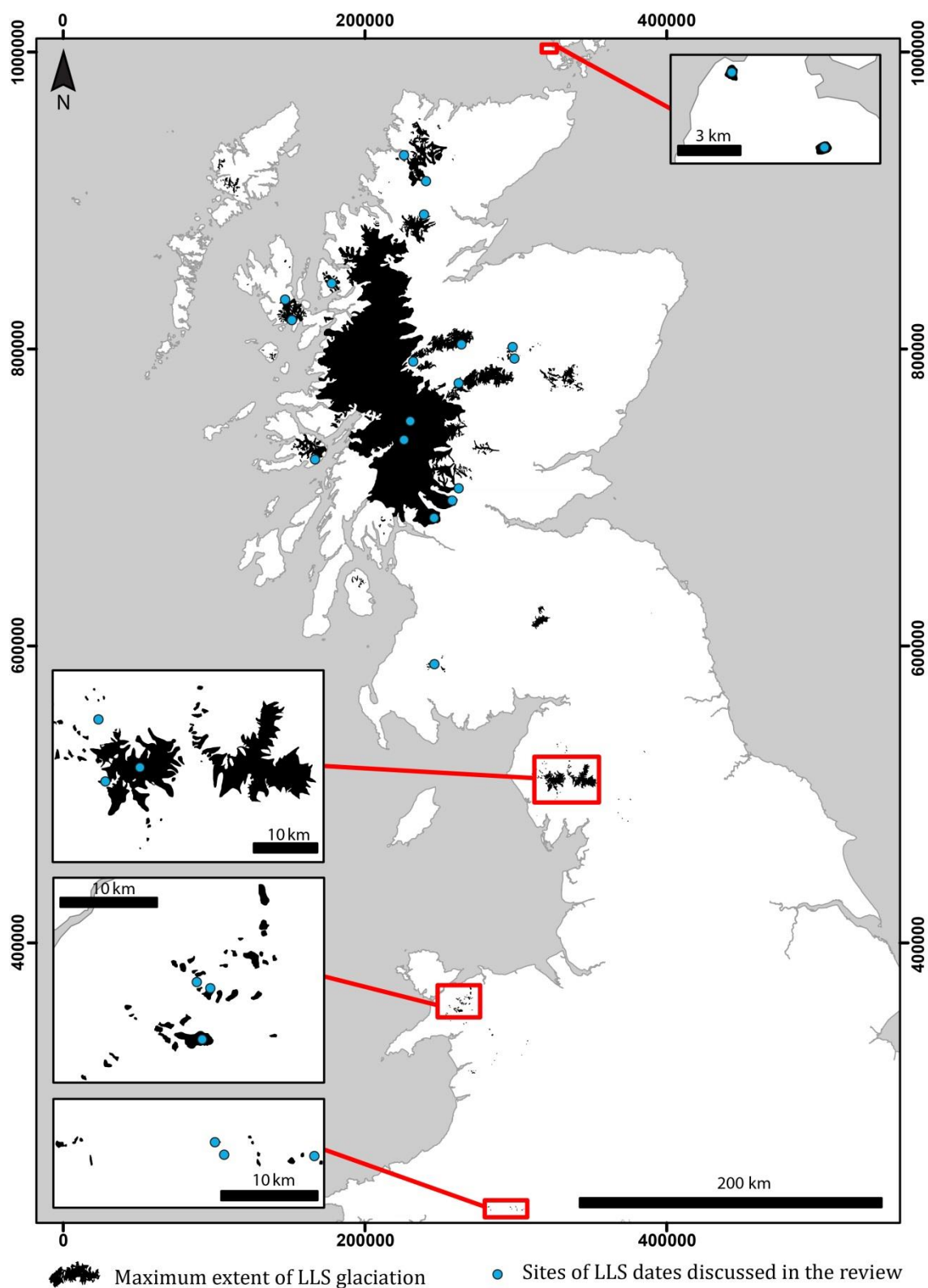
Figure 3.29 Approximate reconstruction of the maximum extent of LLS glaciation in Britain. The West Highland Glacier Complex is shown flanked by satellite icefields, while in marginal areas, glaciation is limited to topographically favourable valleys and cirques. Britain coastline reproduced from Ordnance Survey © Crown Copyright and Database Right 2015. Ordnance Survey (Digimap Licence).
