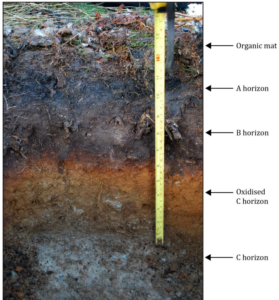
Figure 5.2 Example of a soil profile from Deepdale, Lake District. The top of the profile displays an organic mat, below which the black layer represents the organic rich A horizon. Below this is a B horizon which transitions from a more grey-brown colour to darker shades at its base. At the bottom of the profile there is an orange oxidised C horizon and the more olive-grey unchanged parent material (C horizon).
