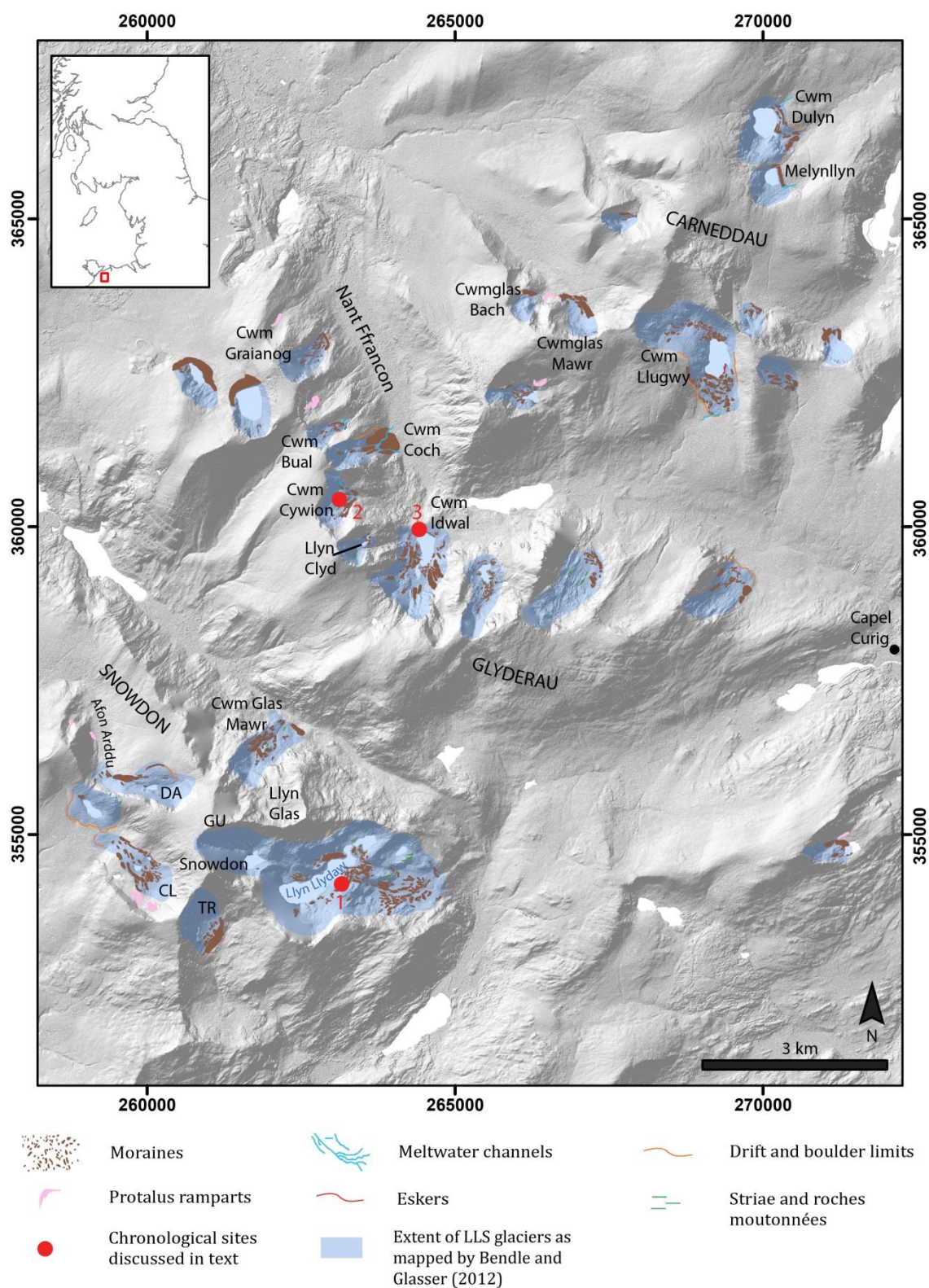
Figure 3.26 The LLS glacial geomorphology of Snowdonia and reconstructed ice extents (after Bendle and Glasser, 2012). DA: Cwm Du'r Arddu, GU: Garnedd Ugain, CL: Cwm Clogwyn, TR: Cwm Tregalan. Underlying hill-shaded image derived from NEXTMap DSM from Intermap Technologies Inc. provided by the NERC Earth Observation Data Centre.
