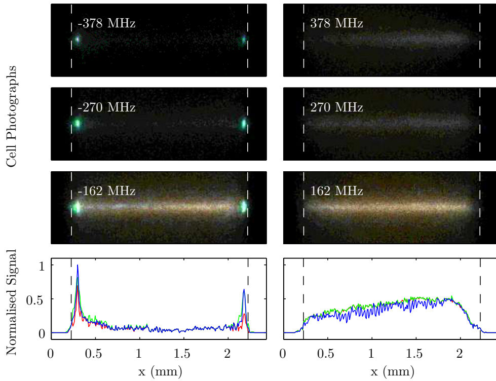
Figure 7.6: Cell wall interaction. Top: Images of background fluorescence for labeled Rydberg laser detuning, \Delta_R/2\pi . Bottom: Cross section for \Delta_R/2\pi = -162 MHz and \Delta_R/2\pi = 162 MHz. The extent of the vapour cell is marked by dashed lines.
