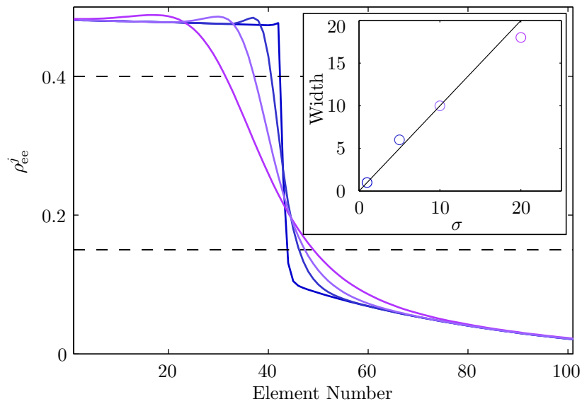
Figure 5.6: Simulations results. We plot the excited state population, \rho_{ee} , in a chain of interacting elements, with interaction length, \sigma = \{1, 5, 10, 20\} . Inset: the width of the phase boundary (between the dashed lines) is plotted as a function of interaction length.
