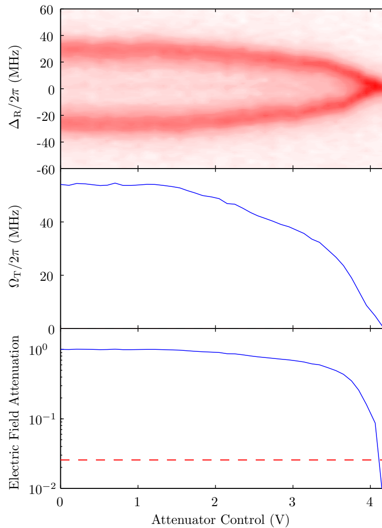
Figure 6.4: Attenuator calibration: We present a colormap showing the change of probe laser transmission in the parameter space of Rydberg laser detuning and the attenuator control voltage (top). In the middle panel we show the fitted terahertz Rabi frequency, \Omega_T . The relative attenuation is shown in the bottom panel, and the measurement floor is indicated with a dashed red line (derived using the 1.4 MHz errorbar found in section 6.4).
