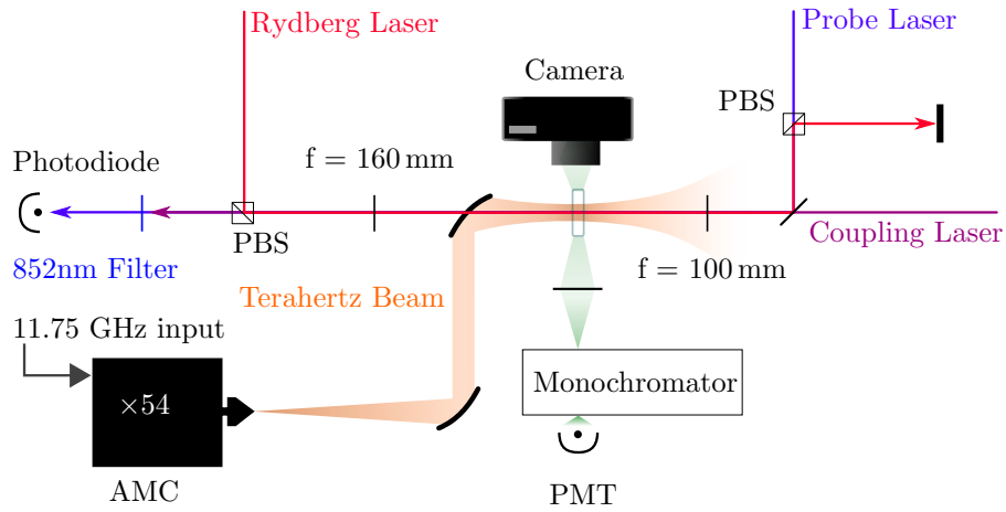
Figure 3.4: Bench layout for Rydberg experiments: The probe, coupling and Rydberg lasers are combined using dichroic mirrors and polarising beam splitting (PBS) cubes, and focused through a 2 mm caesium vapour cell in a co-axial geometry. The vapour is analysed using a photodiode to monitor the transmission of the probe laser, and a camera and spectrometer to measure the atomic fluorescence. A terahertz beam is generated by an amplifier multiplier chain (AMC), and focused through the caesium vapour using gold-coated parabolic mirrors.
