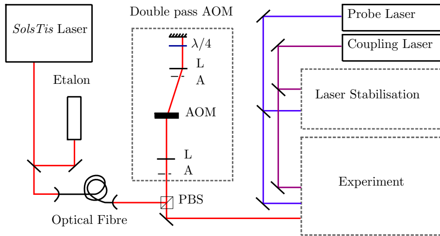
Figure 3.3: Rydberg laser preparation. The Rydberg laser is derived from a SolsTis Ti:Sapphire laser, and passes through an optical fibre and double pass acousto-optic modulator set-up using a quarter waveplate ( \lambda/4 ), polarising beam splitting cube (PBS), apertures (A) and lenses (L). An etalon is used to monitor the frequency scan.
