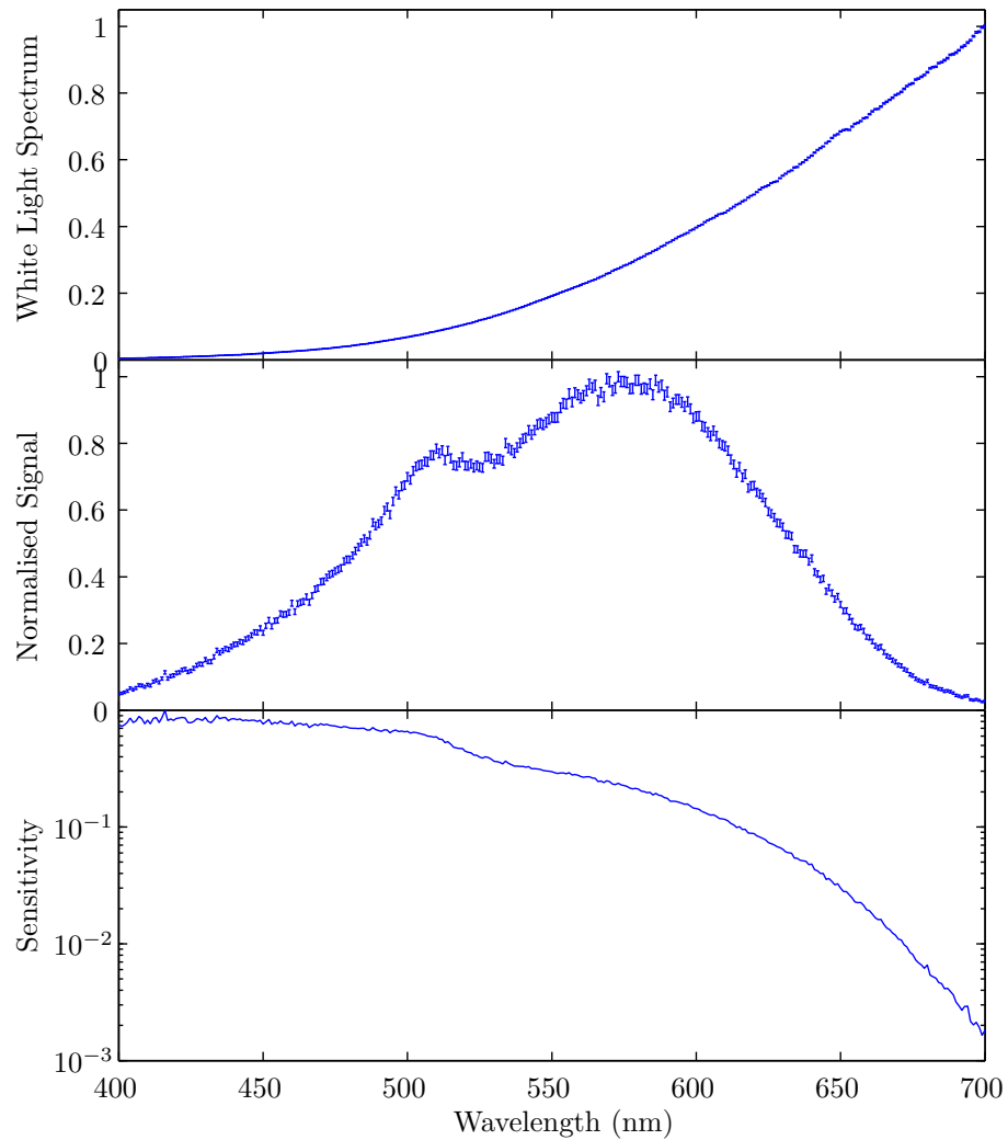
Figure 3.5: Monochromator Calibration: We compare the known spectrum of a white light source (top) to a measurement of the same spectrum using our lab equipment (middle), and deduce the relative sensitivity of our equipment as a ratio between the two (bottom).
