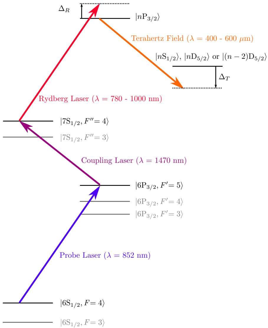
Figure 3.2: Three step ladder excitation scheme. A probe, coupling and Rydberg laser drive a ladder excitation scheme to Rydberg states in caesium, and a terahertz-frequency field drives transitions between Rydberg states.
