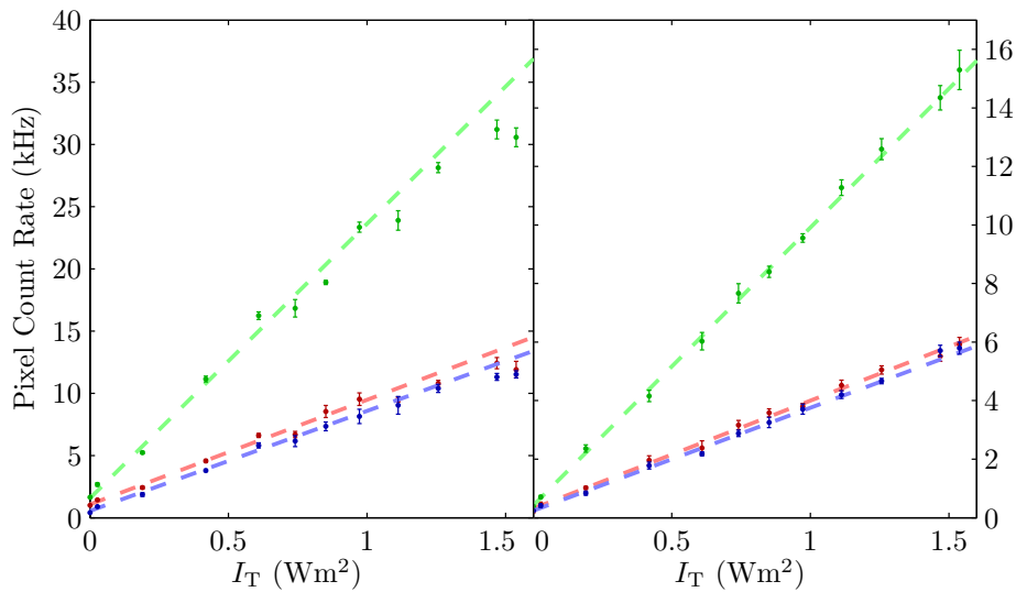
Figure 7.2: Camera Calibration: We present the camera signal as a function of THz intensity for \Delta_R/2\pi = \Delta_T/2\pi = -135 MHz (left) and \Delta_R/2\pi = \Delta_T/2\pi = -243 MHz (right). The red, green and blue (rgb) data points and fit lines correspond to the rgb channels in the camera respectively. The error bars represent statistical variation in five repeated measurements.
