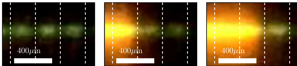
Figure 8.5: Terahertz phase domain photographs. Left: A back reflection of the THz beam causes a standing wave pattern in the atomic fluorescence. The nodes are spaced slightly further than half a wavelength apart ( 237 \mu\text{m} ), because the reflected beam is not coaxial with the incident beam. Middle, Right: A boundary between Rydberg high- and low-density Rydberg collective states is pinned between nodes of the standing wave. The interface is located at the boundary between the bright orange and pale green fluorescence.
