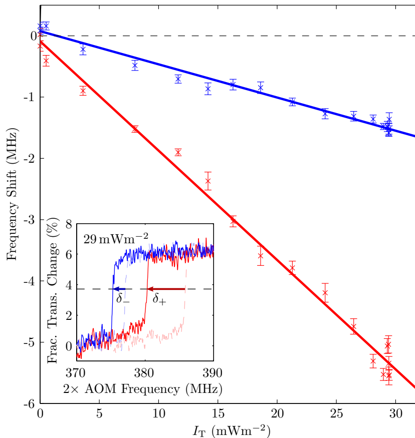
Figure 8.3: Phase Transition Shift. We show \delta_+ (red) and \delta_- (blue) as a function of THz intensity, with a straight line fit. Inset: \delta_+ and \delta_- are read from a frequency scan controlled by an AOM. The bold (faint dashed) line shows the hysteresis with the THz field at intensity I_T = 29 \text{ mWm}^{-2} ( I_T = 0 \text{ mWm}^{-2} ), whilst the laser frequency is increased (red) and decreased (blue). The THz intensity is measured using the Rydberg electrometry technique presented in chapter 6.
