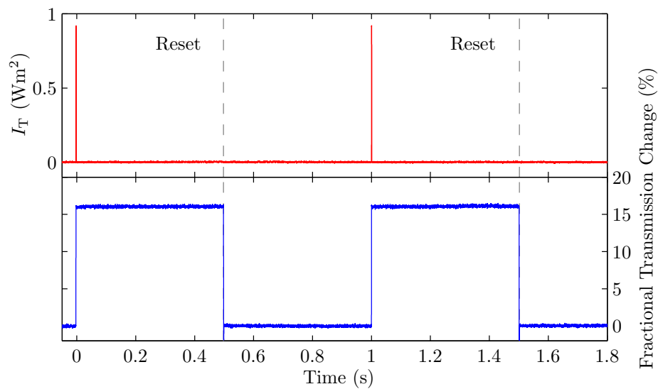
Figure 8.6: Latching detector: A 1 ms pulse from the THz source flips the system between bistable phases. The system remains in its altered state until the Rydberg laser power is cycled (dashed line, ‘reset’).
