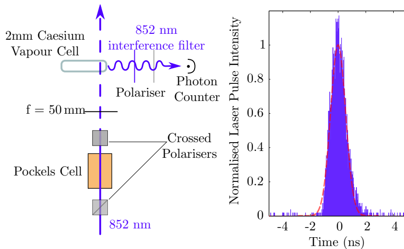
Figure 4.2: Left: Time-resolved atomic fluorescence is recorded by a photon counting unit. Laser pulses are created by a Pockels cell which is placed between crossed polarisers. Right: Measurement of the pulse profile. The red dotted line is a Gaussian fit with 1/e time of 0.8 ns.
