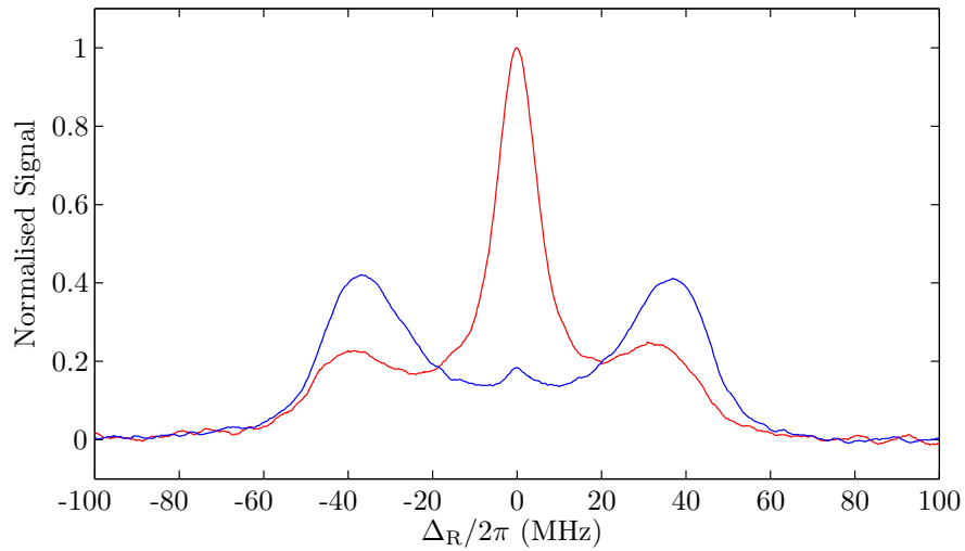
Figure 6.5: Laser polarisation effect on line shape. We show the probe transmission when the Rydberg laser polarisation is parallel (blue) and perpendicular (red) to the THz electric field. The laser powers and beam waists for the probe, coupling and Rydberg lasers were \{0.3 \mu\text{W}, 50 \mu\text{m}\} , \{1 \mu\text{W}, 50 \mu\text{m}\} and \{4 \text{mW}, 60 \mu\text{m}\} respectively.
