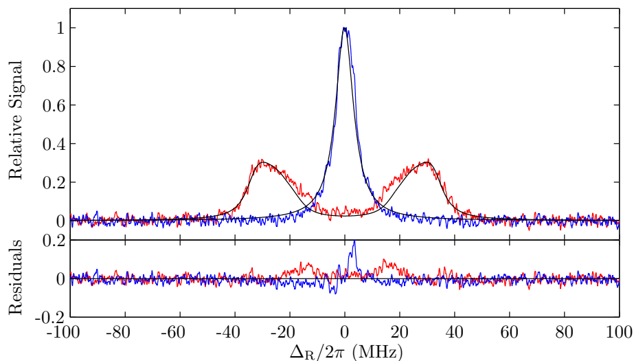
Figure 7.5: THz electric field measurement using electromagnetically induced transparency (EIT): Rydberg EIT is measured for the standing wave image (red), and with the THz field switched off (blue). The peak splitting is proportional to the THz electric field amplitude, and so the doublet peaks are broadened by the field variation in the standing wave.
