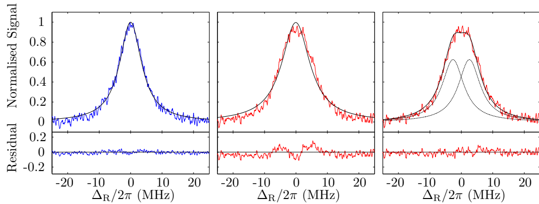
Figure 6.3: THz electric field amplitude measurement. We show the probe transmission line shape for \Omega_T = 0 (left) and \Omega_T = 2\pi \times 5.2 \pm 1.4 MHz (middle, right). The best fit lines (black) are a single Lorentzian (left, middle) and a summed pair of Lorentzian peaks (right, dashed lines). The Rydberg laser and THz fields have matched parallel polarisation, and the laser powers and beam waists for the probe, coupling and Rydberg lasers were measured to be \{0.2 \mu\text{W}, 40 \mu\text{m}\} , \{0.7 \mu\text{W}, 110 \mu\text{m}\} and \{10.2 \text{mW}, 130 \mu\text{m}\} respectively.
