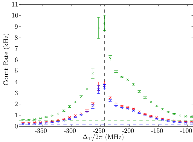
Figure 7.3: Spectral bandwidth: The red, green and blue camera channel sensitivity (red, green and blue points respectively) is shown as a function of the terahertz field detuning, \Delta_T . The Rydberg laser detuning is set \Delta_R/2\pi = -243 MHz (shown by the dashed line), and the THz intensity is set at 1 \text{ Wm}^{-2} .
