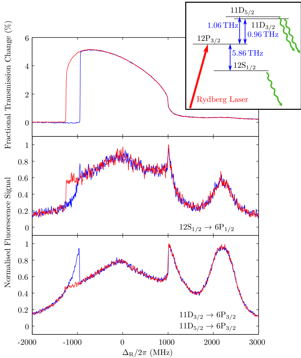
Figure 5.1: Transmission and fluorescence signals as the Rydberg laser is scanned across the 7S_{1/2} to 12P_{3/2} transition (882 nm). The laser is scanned with increasing (blue) and decreasing (red) frequency. We show the measured atomic fluorescence on the 12S_{1/2} \rightarrow 6P_{1/2} (middle, 541 nm) and 11D \rightarrow 6P_{3/2} (bottom, 550 nm) transitions. We note that the spectrometer cannot resolve the 11D fine structure.
