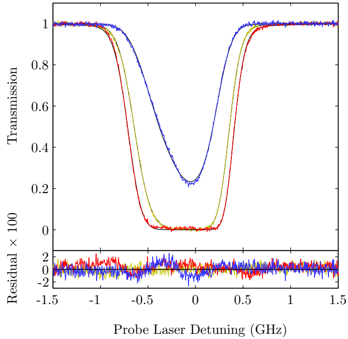
Figure 3.1: Weak probe transmission profile of the D_2 F = 4 \rightarrow F' = \{3, 4, 5\} caesium transition in a 2 mm cell at 48^\circ\text{C} (blue), 68^\circ\text{C} (yellow) and 77^\circ\text{C} (red). The temperatures are inferred from a model fit (black lines) in which temperature is a free parameter. The relative laser detuning was measured using an etalon, and a global frequency shift was used as a fit parameter, setting the F = 4 \rightarrow F' = 5 transition to zero.
