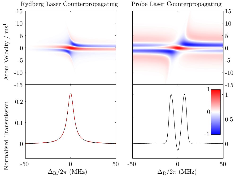
Figure 6.1: Laser geometry effect on 3-photon EIT line shape. We show simulated transmission line shapes (bottom) and velocity class contributions (top) for the laser beam configuration used in this work (left) and previous work [87](right). The velocity class contributions show the change of the probe laser absorption coefficient normalised to the maximum change. The bottom left plot compares the calculated line shape with a Lorentzian function FWHM 8.4 MHz (red dashed line). The laser parameters are set, \Omega_p = \Omega_c = 2\pi \times 2 MHz, \Omega_R = 2\pi \times 8.4 MHz.
