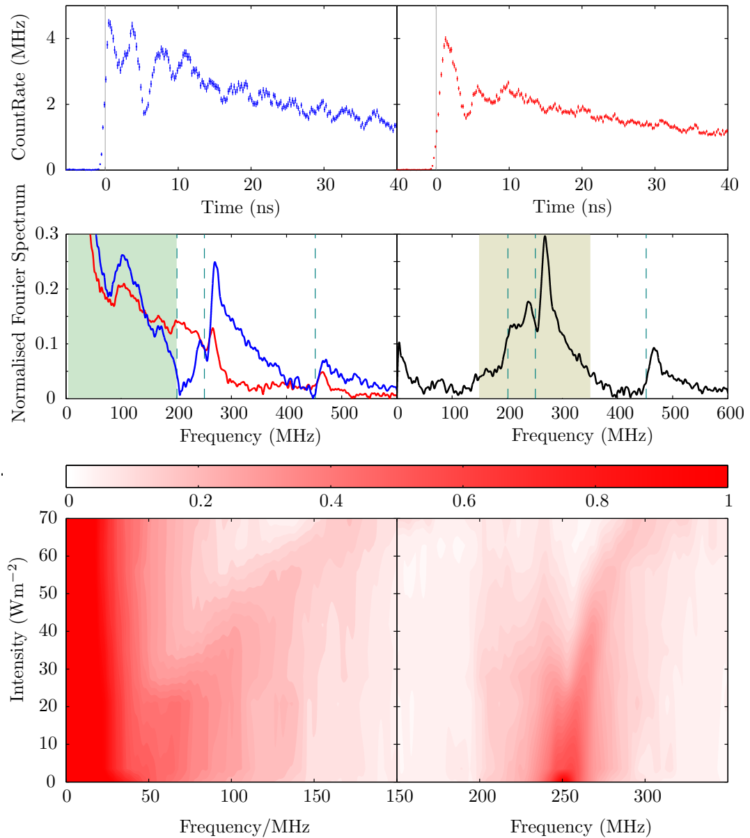
Figure 4.4: Quantum beats modified by an excited state transition. Top row: For measured intensity I_d = 4 \text{ W cm}^{-2} we show the vertical polarised (left) and horizontal polarised (right) fluorescence as a function of time. Middle row: The beat spectra are shown for vertical (blue) and horizontal (red) polarised fluorescence (left), and the difference signal (right). The dashed vertical lines show the bare hyperfine beat frequencies, and the shaded areas correspond to colourmaps (bottom row), showing the vertical polarised signal (left) and the difference signal (right) with changing coupling laser intensity.
