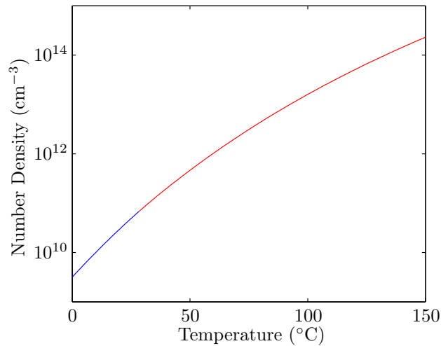
Figure 1.1: Caesium vapour number density with changing temperature, calculated from [39]. The blue (red) line indicates when the vapour is in equilibrium with a solid (liquid) phase.
