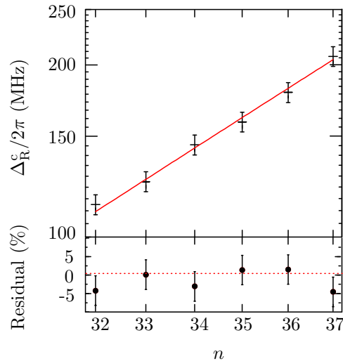
Figure 5.3: Shift of the critical detuning, \Delta_R^c , with changing principal quantum number, n . The data were recorded and analysed by N. R. de Melo .
