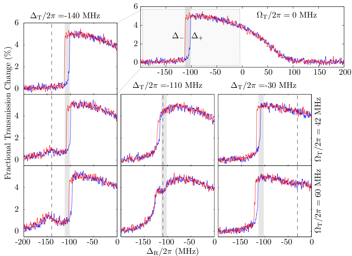
Figure 8.1: Bistability line shape modification: The grey shaded area highlights the bistable scan range before the THz field is applied. The THz field has detuning \Delta_T/2\pi = -140 MHz (left), -110 MHz (middle) and -30 MHz (right), shown by the dashed lines. The THz field has Rabi frequency \Omega_T/2\pi = \{0, 42, 60\} MHz (top, middle and bottom).
