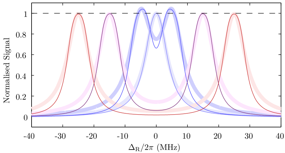
Figure 6.2: Autler-Townes splitting simulation. We compare a 5-level optical Bloch model (coloured lines) with Lorentzian features (shaded lines), for THz Rabi frequencies, \Omega_T = 2\pi \times \{0, 10, 30, 50\} MHz. The line shapes are normalised to the feature calculated for \Omega_T = 0 . The laser parameters are set, \Omega_p = \Omega_c = 2\pi \times 5 MHz, \Omega_R = 2\pi \times 8.4 MHz.
