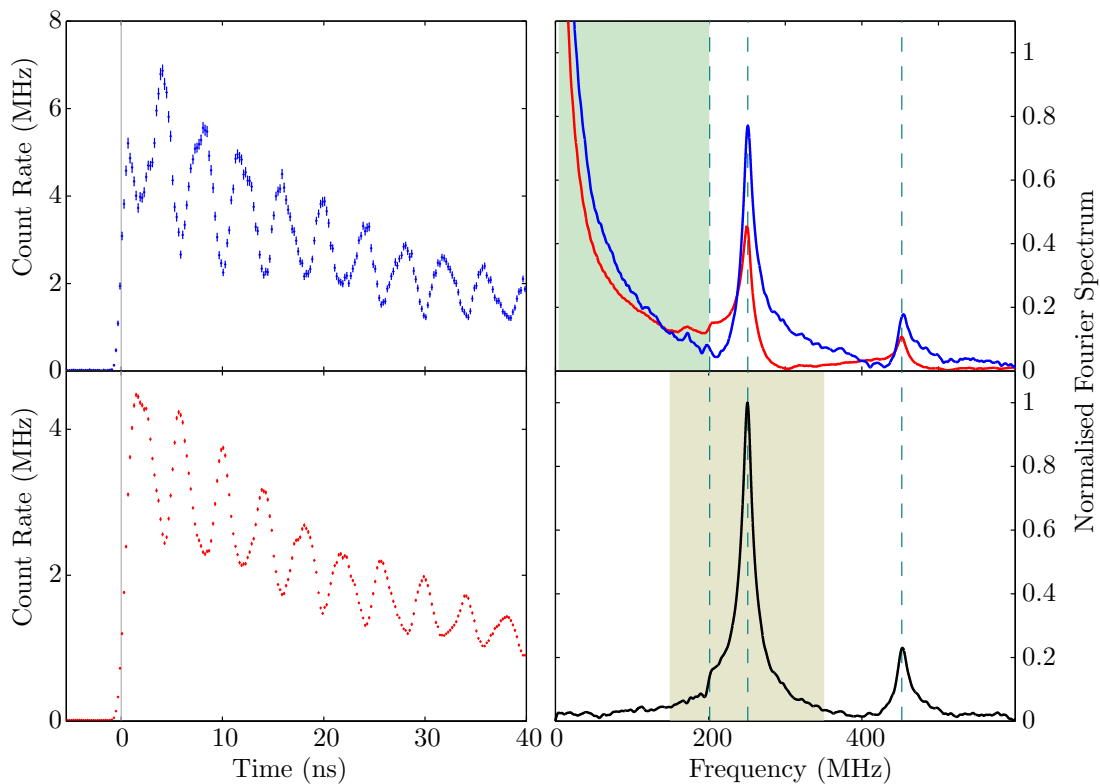
Figure 4.3: Hyperfine quantum beats: Time resolved fluorescence measurements (left column) show the vertical (top) and horizontal (bottom) polarised fluorescence beating in antiphase (the center of the excitation pulse is incident at time t = 0 ns). The Fourier transform of the time signal shows the beat frequencies (right column). We show the magnitude of the Fourier transform (top) for the vertical (blue) and horizontal (red) polarised fluorescence and the difference signal (bottom).
