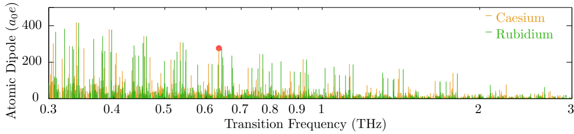
Figure 1.2: Resonant transitions between Rydberg states in the THz band for Rubidium and Caesium. The transition used in this thesis is marked with a red dot. The transition frequencies and dipole strengths were calculated by N. Šibalić [64].
