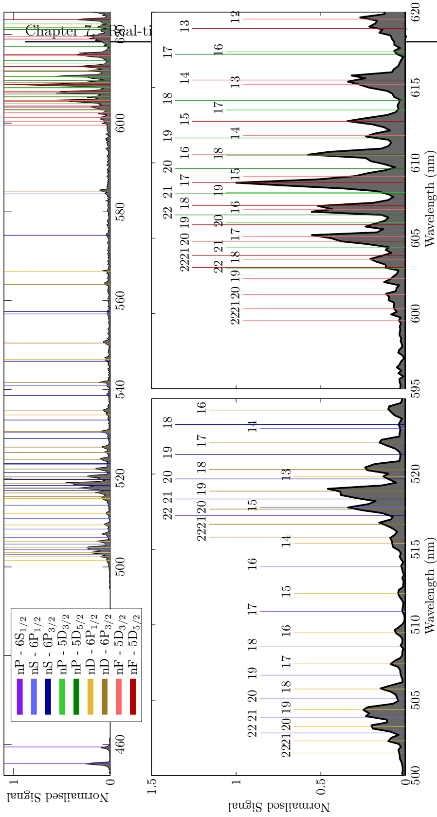
Figure 7.1: Visible atomic fluorescence spectrum. Top: complete scan from 450 - 630 nm. Bottom: Selected regions of the spectrum are shown with labelled atomic transitions. The number associated with each line refers to the principle quantum number of the decaying Rydberg state, and the colour indicates the angular momentum of the Rydberg and final states. The data were recorded with \Delta_R = \Delta_T = 2\pi \times -259 MHz and the cell temperature was 71°C.
