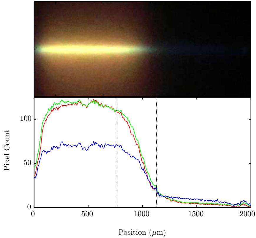
Figure 5.5: Phase boundary. Top: Photograph showing atomic fluorescence. The laser beam propagates left to right across the vapour cell which fills the image. However, the left side shows bright orange fluorescence (high Rydberg number density phase), whereas the right hand side is dark (low Rydberg number density phase). Bottom: Cross section of the camera signal along the laser beam. We show the three camera colour channels (red, green and blue). The vertical lines, spaced 350 \mu\text{m} apart, indicate the 90%-10% width of the domain boundary.
