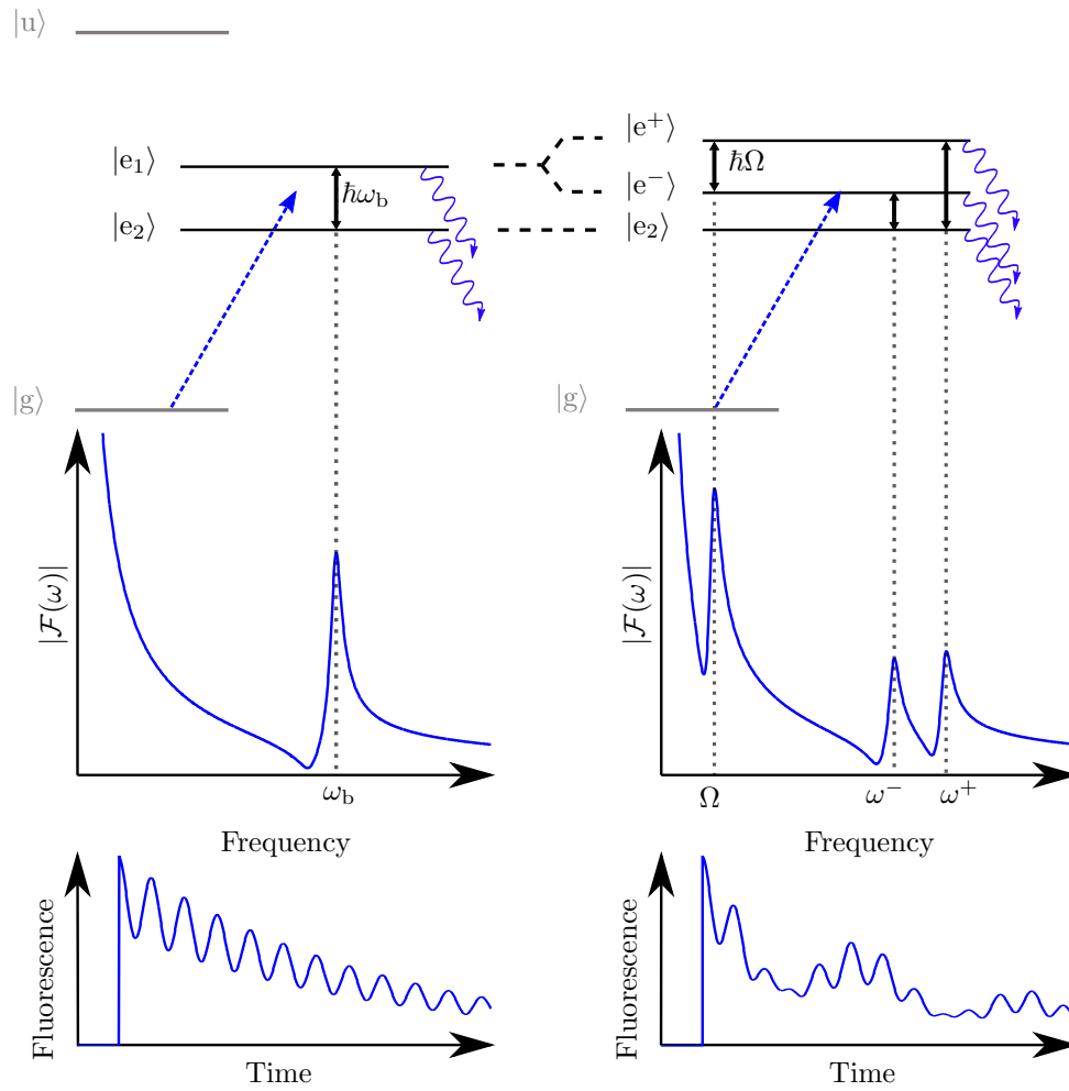
Figure 4.1: Toy model. Left column: A short pulse prepares a superposition of states |e_1\rangle and |e_2\rangle which fluoresce to produce quantum beats. The Fourier transform (middle row) of the fluorescence signal (bottom row) allows the investigator to read off the beat frequency, \omega_b . Right column: Driving an excited state transition is most easily understood in the dressed state picture. State |e_1\rangle is coupled to state |u\rangle to produce dressed states |e^+\rangle and |e^-\rangle . The fluorescence signal now shows a trio of beat frequencies, \Omega , \omega^+ and \omega^- .
