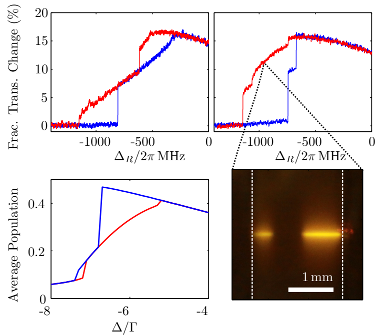
Figure 5.7: Phase boundary connection to line shape. Left: A double hysteresis loop is seen as the Rydberg laser frequency is increasing (blue) and decreasing (red), for experiment (top) and theory (bottom). Right: Two simultaneous phase boundaries are observed. The dashed white lines in the photograph show the ends of the vapour cell.
