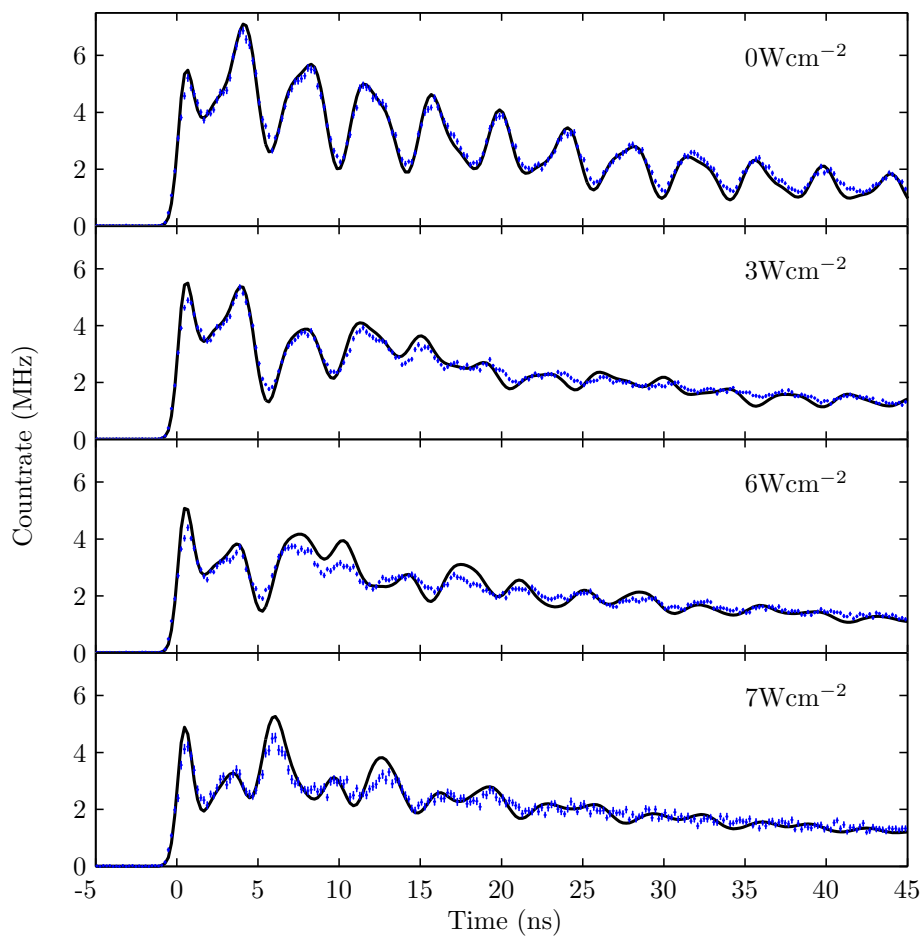
Figure 4.5: Vertically polarized fluorescence: We compare the model (black line) and experimental data points (blue) for measured excited-state transition laser intensity I_d = (0, 3, 6, 7) \text{ W cm}^{-2} (top to bottom). We note that the visibility of the peaks is always smaller than the model predicts. The incident light pulse occurs at time t = 0 ns and the error bars are calculated from Poissonian photon counting statistics [100].
