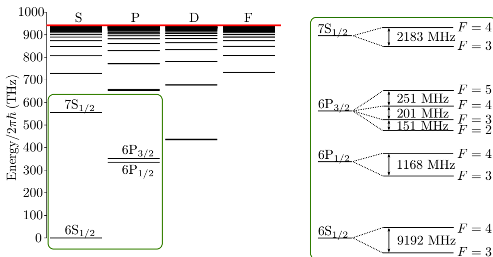
Figure 2.1: Caesium energy levels [78]. Left: S,P,D and F energy levels from the ground state to the ionisation threshold (red line). Right: Schematic representation of the hyperfine splitting of selected states.
