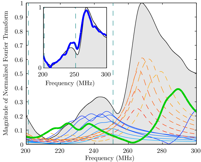
Figure 4.6: Calculated magnitude of the normalized Fourier transform of the vertically polarized fluorescence: We show a break down of velocity class contributions, with dashed (red) lines showing individual velocity classes travelling away from the 852 nm laser, and solid (blue) lines showing velocity classes traveling towards the 852 nm laser. The velocity classes are spaced at 33 \text{ m s}^{-1} intervals and the bold (green) line shows the contribution from zero-velocity atoms. The gray shaded area shows the scaled sum of the signals and the calculation relates to probing a region with a uniform excited-state transition driving field intensity I_d^{\text{Sim}} = 0.9 \text{ W cm}^{-2} . The inset compares the data taken for measured CW driving field intensity I_d = 3 \text{ W cm}^{-2} shown in bold (blue) and the summed model (gray shaded area and black line).
