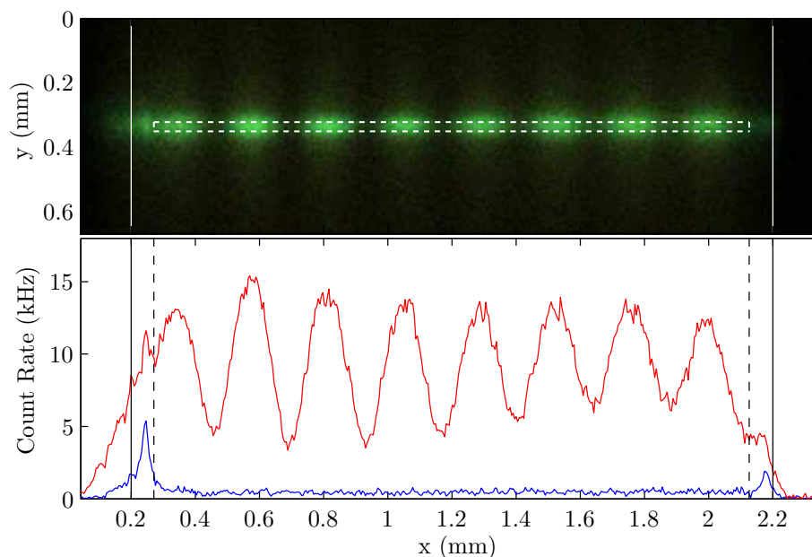
Figure 7.4: Standing Wave Image. Top: THz-induced atomic fluorescence (proportional to the THz intensity) is imaged. The dark vertical stripes indicate the nodes of the THz standing wave, spaced at \lambda/2 intervals ( 237 \mu\text{m} ). Bottom: Cross section of the THz standing wave image (red) and background fluorescence (blue). The dashed lines show the region used to model the line shape, and the bold lines show the extent of the 2 mm vapour cell.
