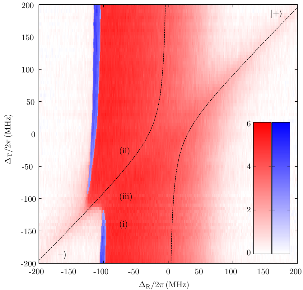
Figure 8.2: Terahertz bistability phase map ( \Omega_T/2\pi = 60 MHz). In monostable regions (red) the colourmap shows the fractional transmission change in the probe beam (%). In bistable regions (blue) we show the difference signal. The black lines show the dressed states, |+\rangle and |-\rangle . The cell temperature was 77^\circ\text{C} and the probe, coupling and Rydberg lasers had 1/e^2 radii and beam power \{30\ \mu\text{m}, 70\ \mu\text{W}\} , \{90\ \mu\text{m}, 28\ \mu\text{W}\} and \{130\ \mu\text{m}, 310\ \text{mW}\} respectively.
