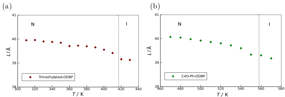
Figure 6.20: The average molecular length as a function of temperature for (a) trimethylated-ODBP and (b) C4O-Ph-ODBP. [Dotted vertical lines show the respective T_{NI} ].
