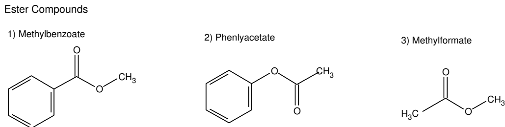
Figure 4.6: Ester structures
