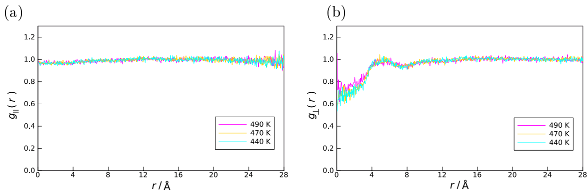
Figure 5.25: Radial distribution functions obtained for the oxadiazole axis for C4-Ph-ODBP-Ph-C7 (a) along the director and (b) perpendicular to the director.
