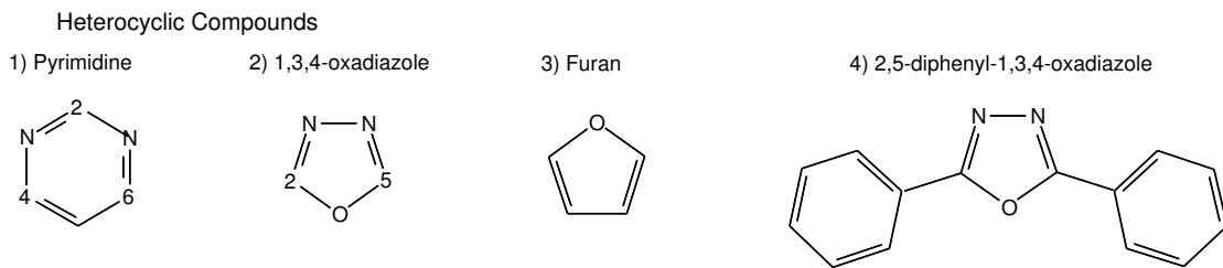
Figure 4.7: Heterocyclic structures
