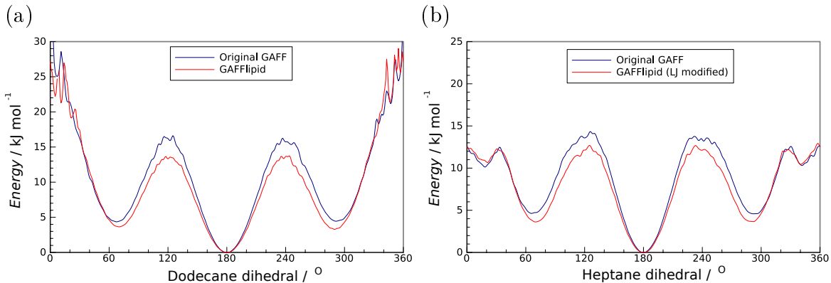
Figure 4.13: Torsion profiles for the \text{CH}_2\text{—CH}_2\text{—CH}_2\text{—CH}_2 dihedral of (a) dodecane and (b) heptane
