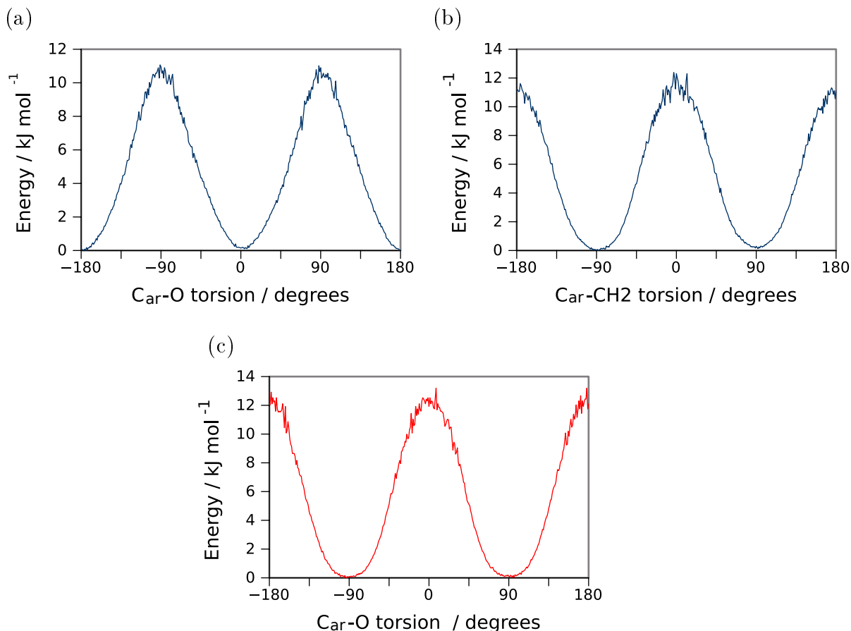
Figure 5.28: Effective torsional potentials obtained by Boltzmann inversion of dihedral distributions obtained from gas phase simulations of C5-Ph-ODBP-Ph-OC12. (a) C ar -O torsion (GAFF-LCFF), (b) C ar -CH 2 torsion (GAFF-LCFF), (c) C ar -O torsion (Test 1).
