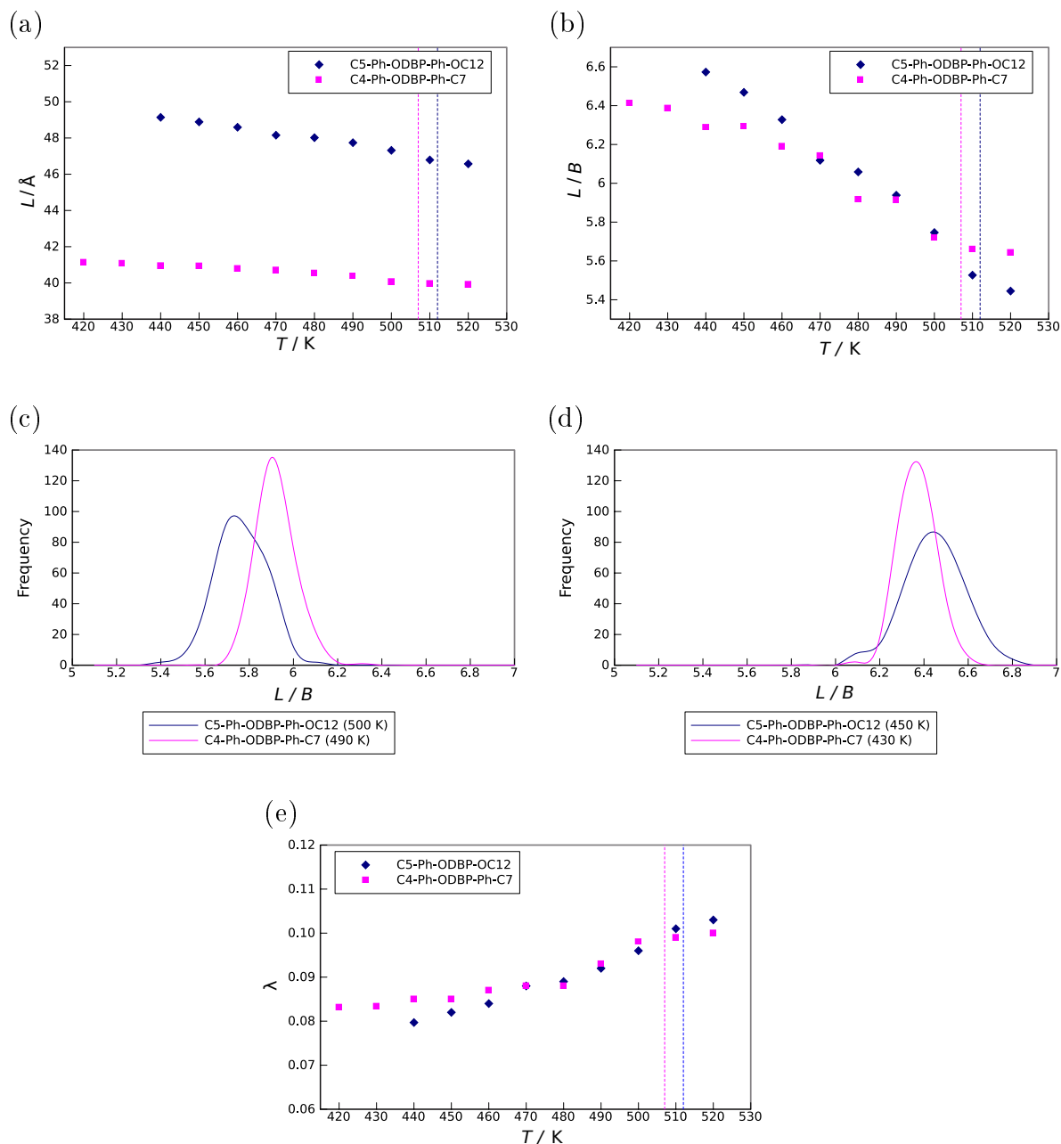
Figure 5.27: Comparisons of: (a) The average molecular length as a function of temperature for the two ODBP systems, (b) The average length to breadth ratio as a function of temperature for the two systems, (c) and (d) The frequency of length to breadth ratio in the high and low temperature nematic range for each mesogen, (e) The average molecular biaxiality as a function of temperature for the two systems. [Dotted vertical lines show the respective T_{NI} ].
