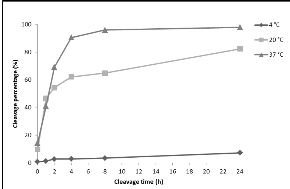
Figure 3.13. Quantification of the cleavage activity over time.
