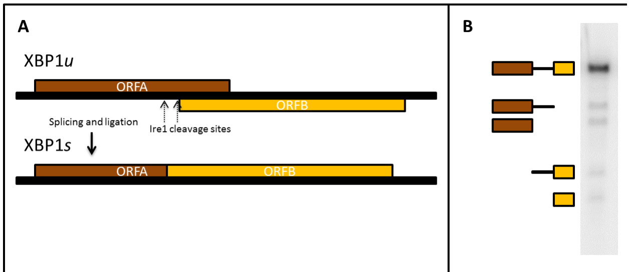
Figure 3.7. The structure of XBP-1 mRNA.
