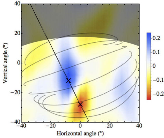
Figure 3.7 – 2D red-blue imbalance map for MAST shot #27969. The color-bar is given in units of volts. The data is generated using the SAMI diagnostic for a 16 GHz omni-directional probing beam 300 ms into the shot. The over-plotted curved lines indicate the magnetic field lines taken from MSE constrained EFIT. The EFIT location was matched against the SAMI probing frequency with the help of TORBEAM using TS data (taken from [111]).
