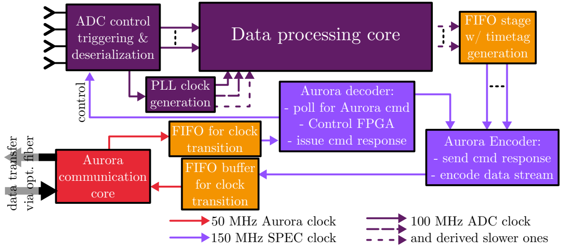
Figure 2.7 – Top level of the diagnostic firmware. The top level design with the communication and the deserialization core is written in VHDL. The processing core is designed using System Generator for MATLAB Simulink. Colors denote different clock regions as indicated in the figure. Orange components transition between clock domains.
