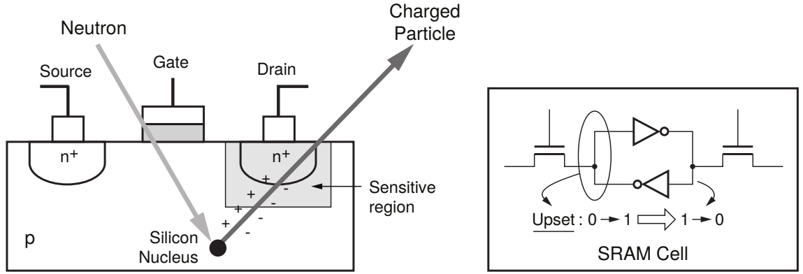
Figure 1.5 – The basic source for a SET. A charged particle, e.g. generated by a neutron striking an atom, traverses the depletion region creating a cloud of electron-hole pairs in the doped silicon substrate thus potentially leading to an unwanted bit flip or a current surge (taken from [43]).
