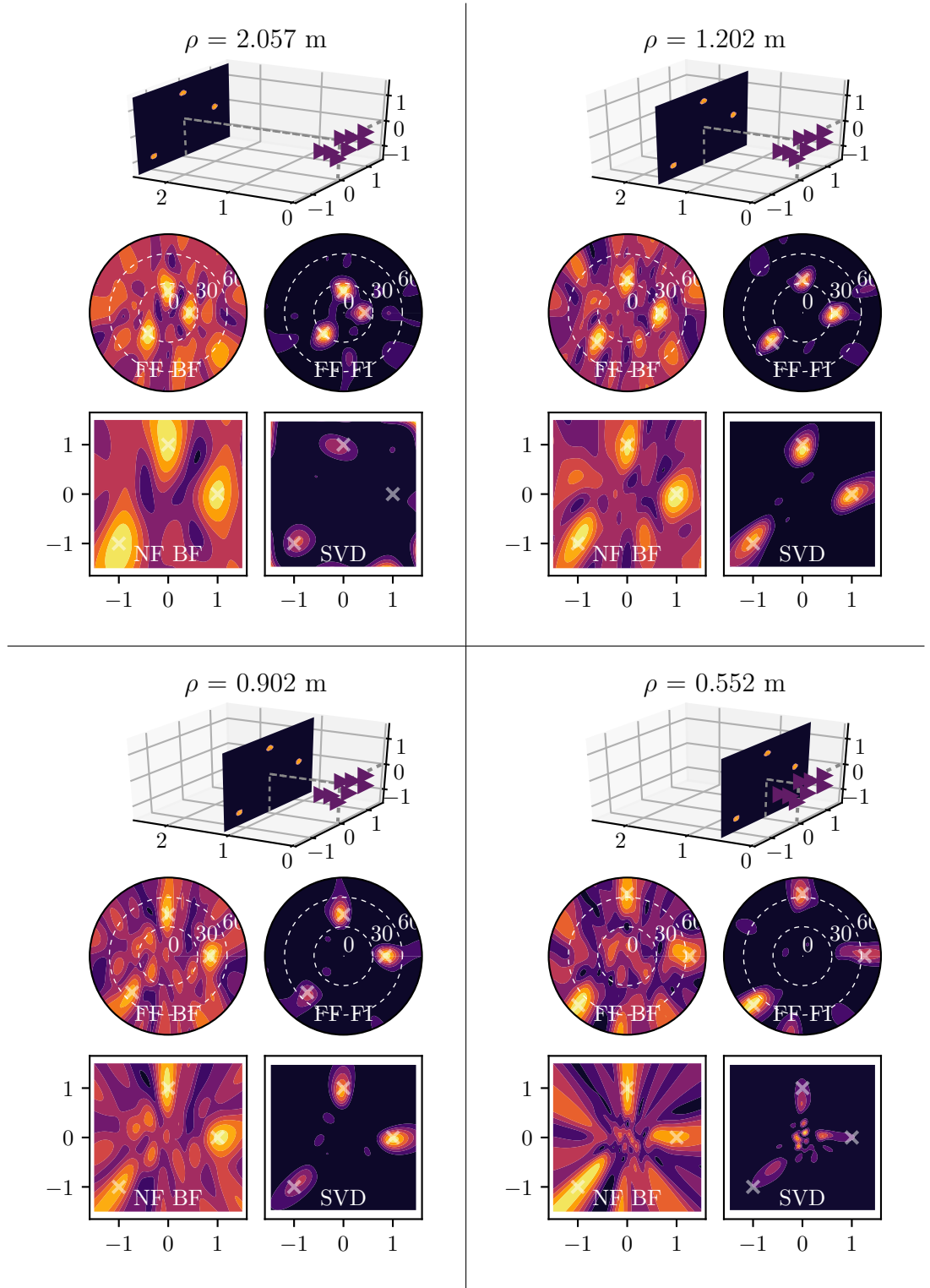
Figure 3.16 – Comparison of image reconstruction algorithms for a planar source emitting at 16 GHz. In each quadrant the simulated geometry is depicted at the top, with \rho given in meters; purple triangles mark the array geometry (scaled by a factor of 20 for visualization purposes). The polar plots in the middle use FF reconstruction with BF (left) and Fourier inversion (right). The bottom plots show the NF reconstruction using BF (left) and SVD inversion (right). Axis descriptions have been omitted for illustration purposes. Cartesian axis labels are in meters. The opening angle in the polar plots is in degree.
