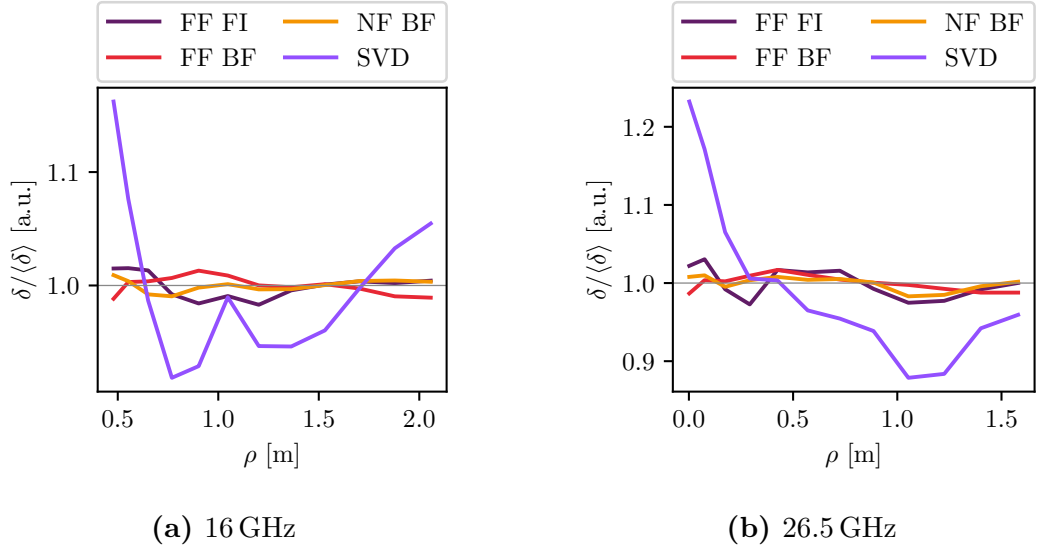
Figure 3.18 – Normalized distortedness \delta over \rho for all four image reconstruction methods and two different probing frequencies. delta is normalized to the average over \rho . Quantitative comparison of the distortedness curves should be taken with great care.
