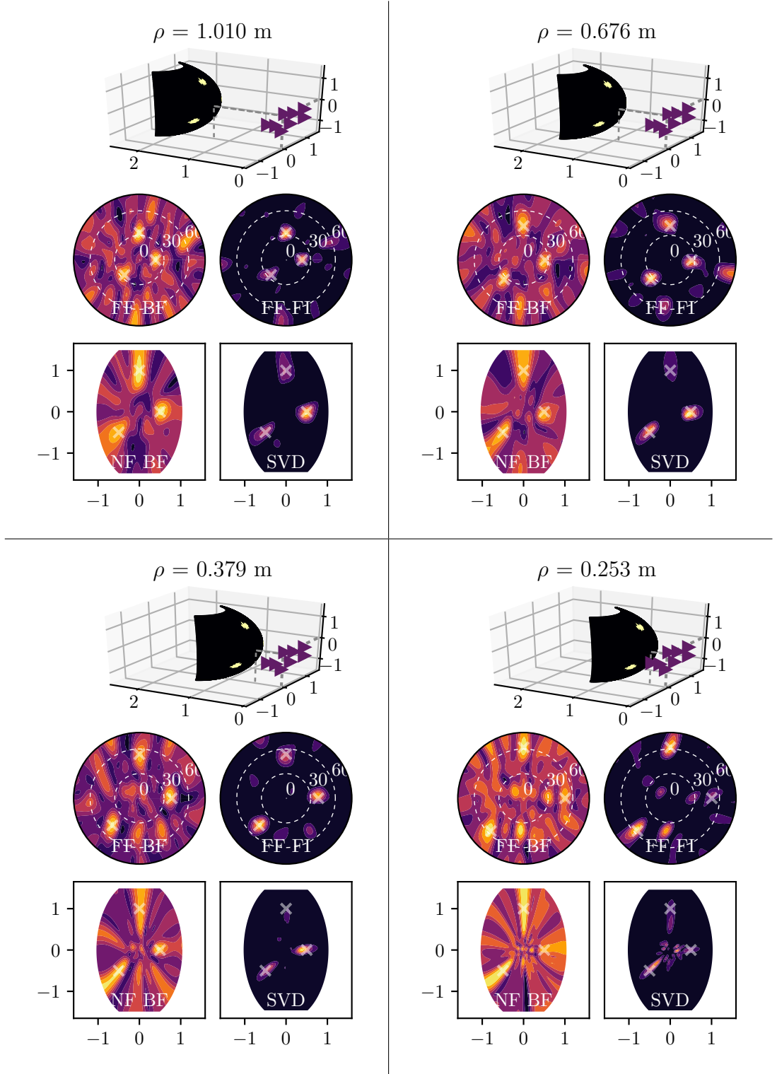
Figure 3.19 – Image reconstruction algorithms compared for different distances of a ellipsoid source emitting at 20.5 GHz. The plot-layout is identical to fig. 3.16.
