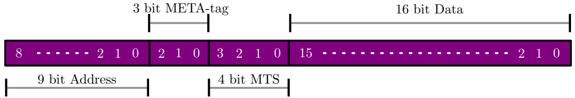
Figure 2.17 – The protocol used on the MAST-U “Aurora network”. Data is transmitted in 4 B(byte) little endian packages. Only half of the bandwidth is used for data transmission. The MTS is used for transmission error checks, the META tag identifies the nature off the package (Read request, Write request etc.).
