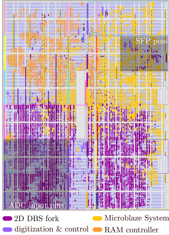
Figure 3.13 – Layout of the SAMI firmware logic on the Virtex-6 FPGA generated using Xilinx PlanAhead. The serial data pins from the ADC are placed in the lower left of the FPGA. The pins related to streaming the data via fiber optic are in the top right. The logic in between is heavily constrained in placement due to the clock speeds it is operated at and the location of the physical pins it controls, most notably the RAM controller.
