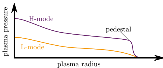
Figure 3.1 – Schematic of the plasma pressure in L-mode and H-mode. The formation of a strong edge pressure gradient and pedestal are the defining properties of H-mode.
