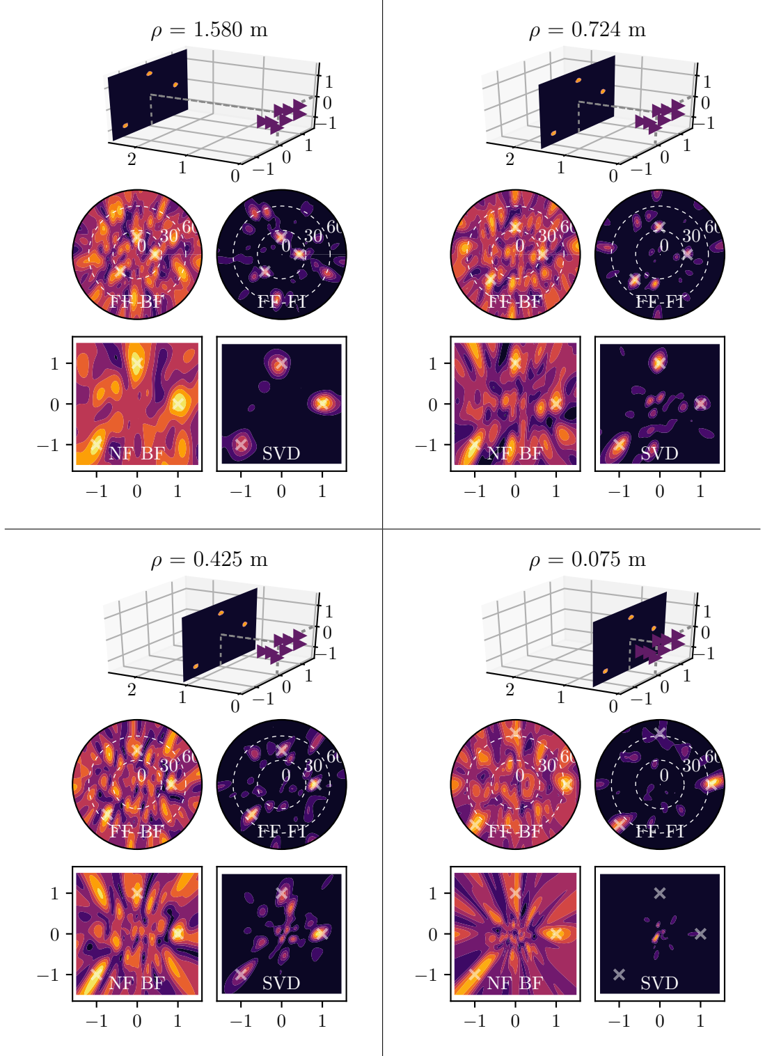
Figure 3.17 – Image reconstruction algorithms compared for different distances of a planar source emitting at 26.5 GHz. The simulation geometry and plot-layout are identical to fig. 3.16.
