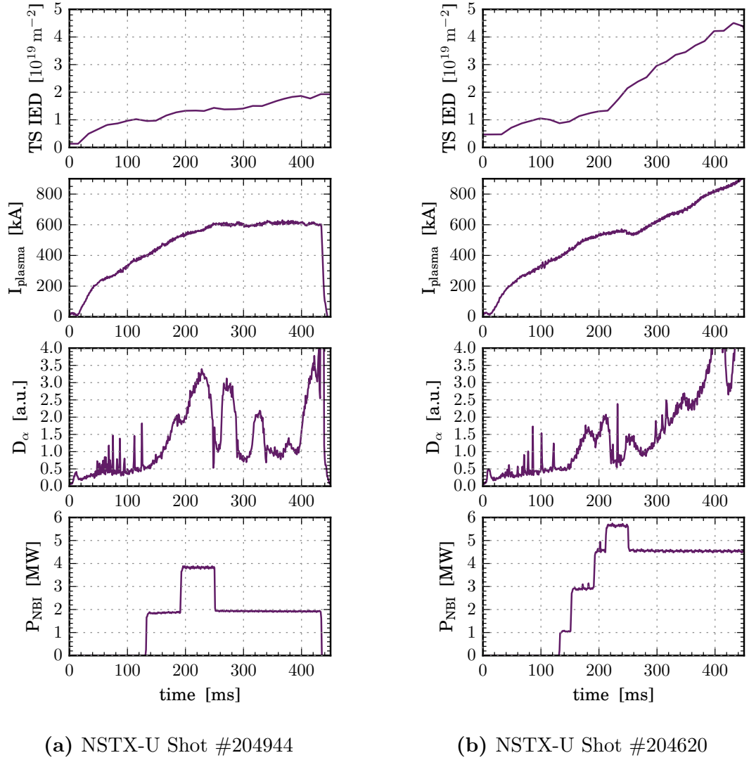
Figure 3.24 – Selection of plasma parameters for the shots shown in figure 3.23. The top depicts the TS calculated IED. Below are the measured toroidal plasma current and the midplane Deuterium- \alpha light intensity. The bottom is the applied NBIH power.
