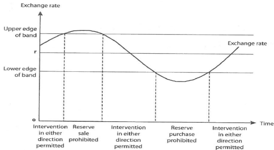
Figure 5.1 Operation of the Reference Rate Rule
