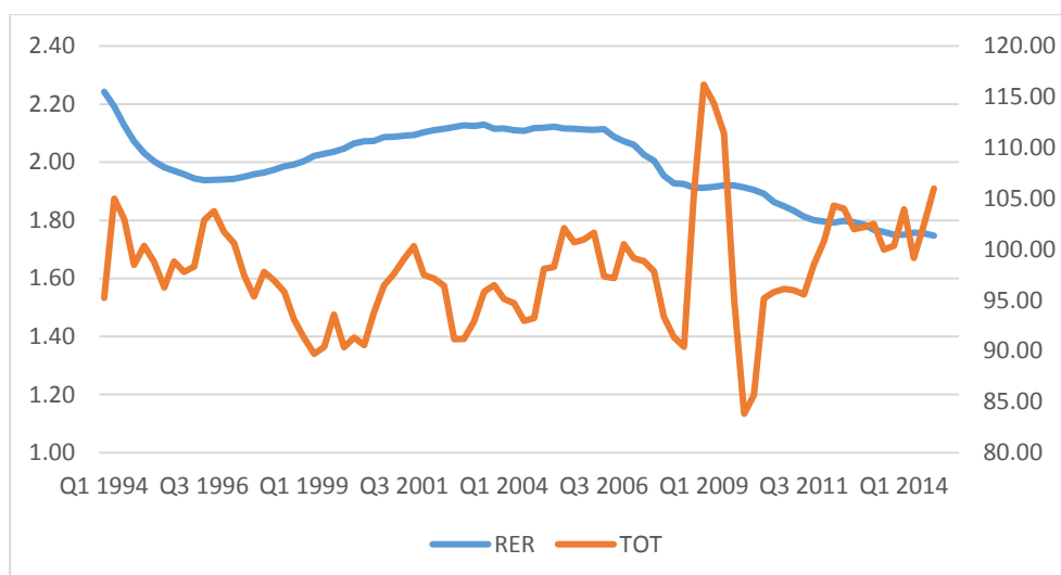
Figure 3.3 RER and TOT
