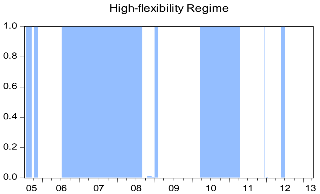
Figure 2.3 Smooth Probabilities of Regimes
