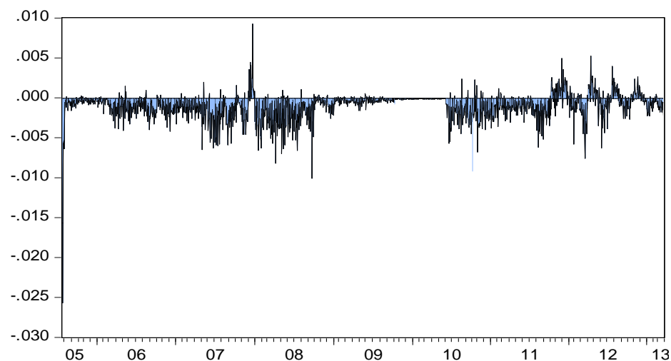
Figure 2.2 Exchange Market Pressure of RMB
