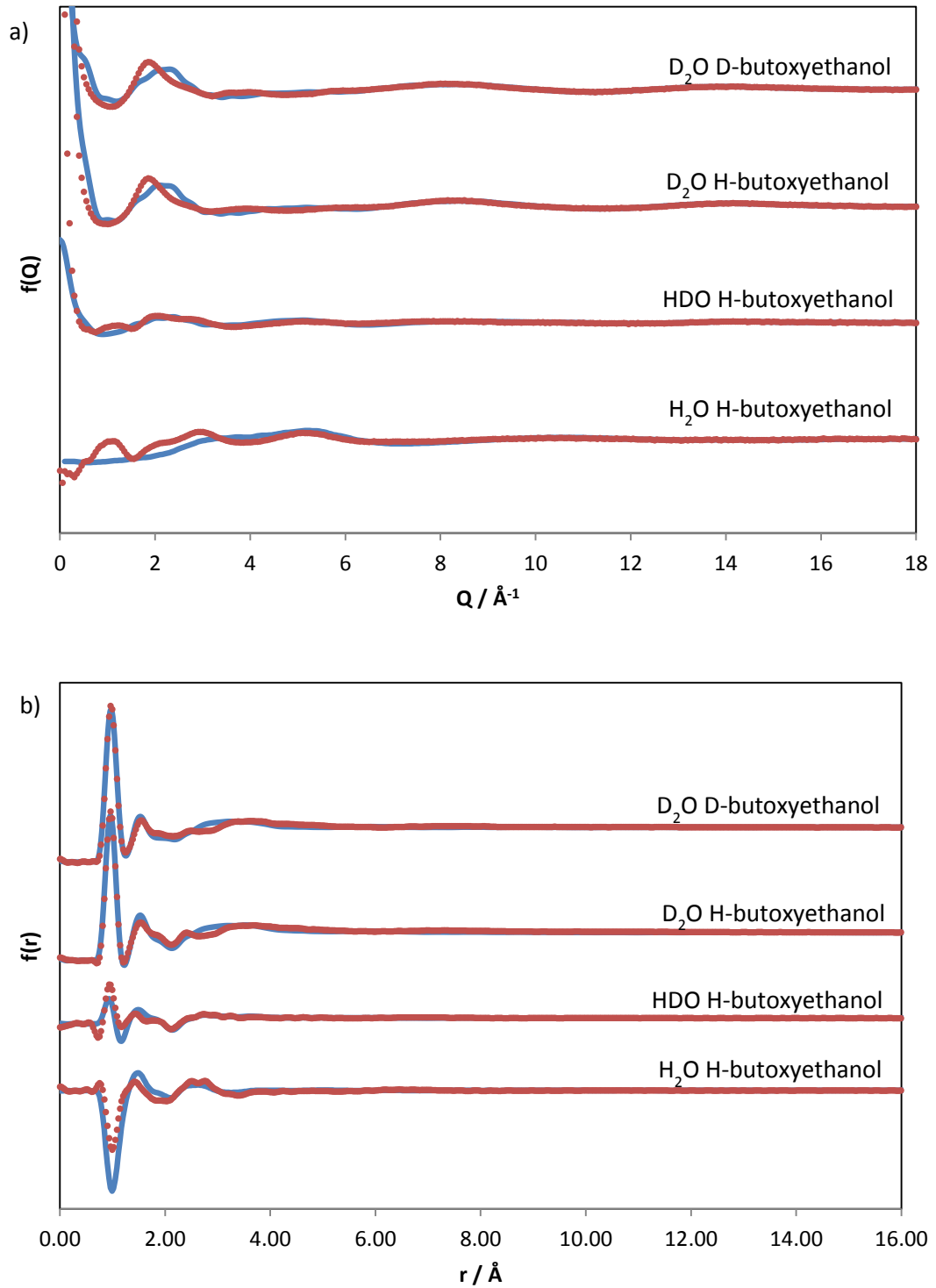
Figure 6.6 – Quality of fit for the EPSR simulation of butoxyethanol/water shown in a) reciprocal space and b) real space. The experimental data are shown by dotted red lines whilst the simulated data are shown by solid blue lines.
