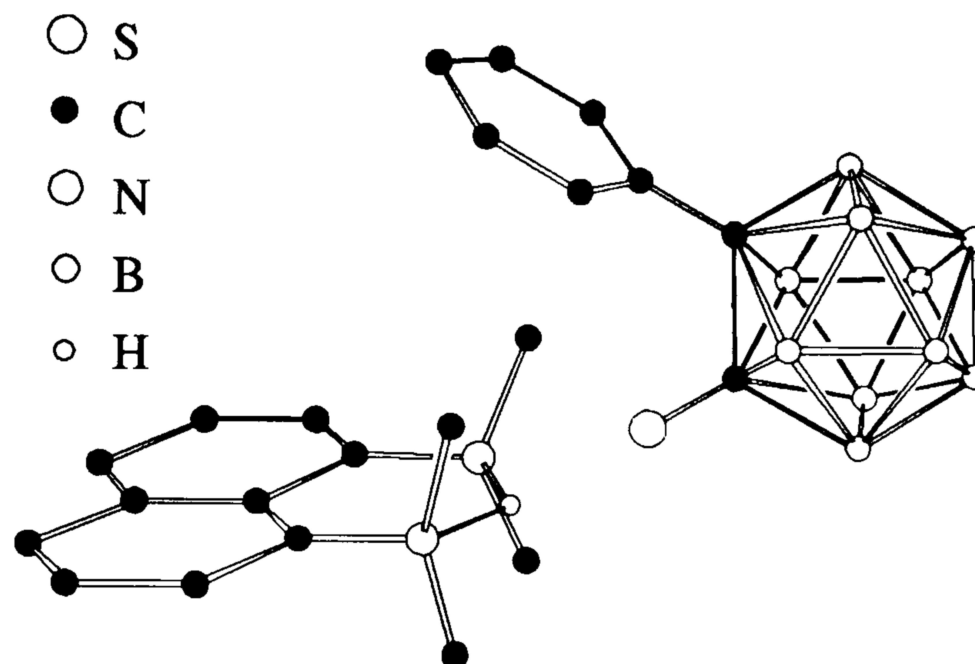
X-ray structure of X , \text{PhCB}_{10}\text{H}_{10}\text{CS}_3\text{CB}_{10}\text{H}_{10}\text{CPh}
