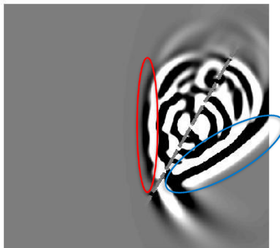
Figure 4.13: X-Z 2D cut plane of electric field for 30 degree incident angle FDTD simulation at t \approx 2 ps.
