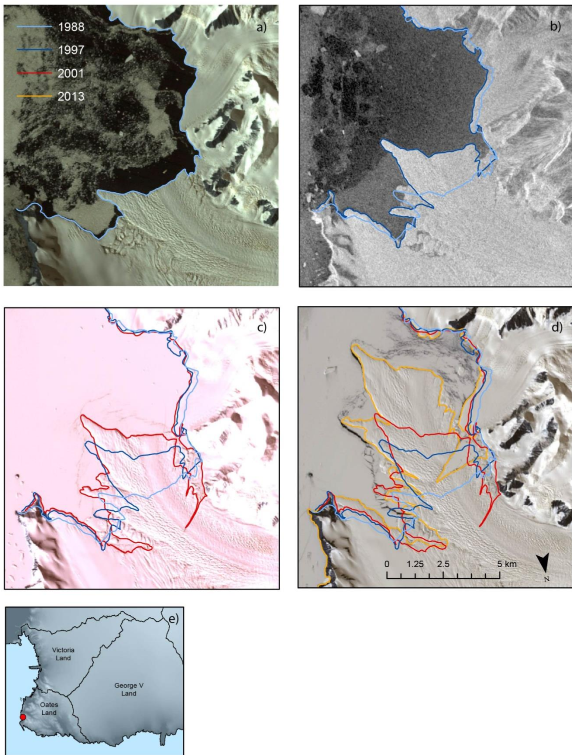
Figure 4.3: Examples of terminus digitisation on Ironside Glacier using imagery from different years a) Landsat TM: 1988, b) ERS SAR: 1997, c) Landsat ETM+: 2001, d) Landsat OLI TIRS: 2013 and e) location map.
