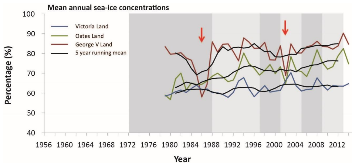
Figure 5.6: Mean annual sea-ice concentrations. The black line represents the 5 year running mean. Red arrows mark the decreases in sea ice in George V Land. Epochs where glacier changes were measured are shaded in background.
