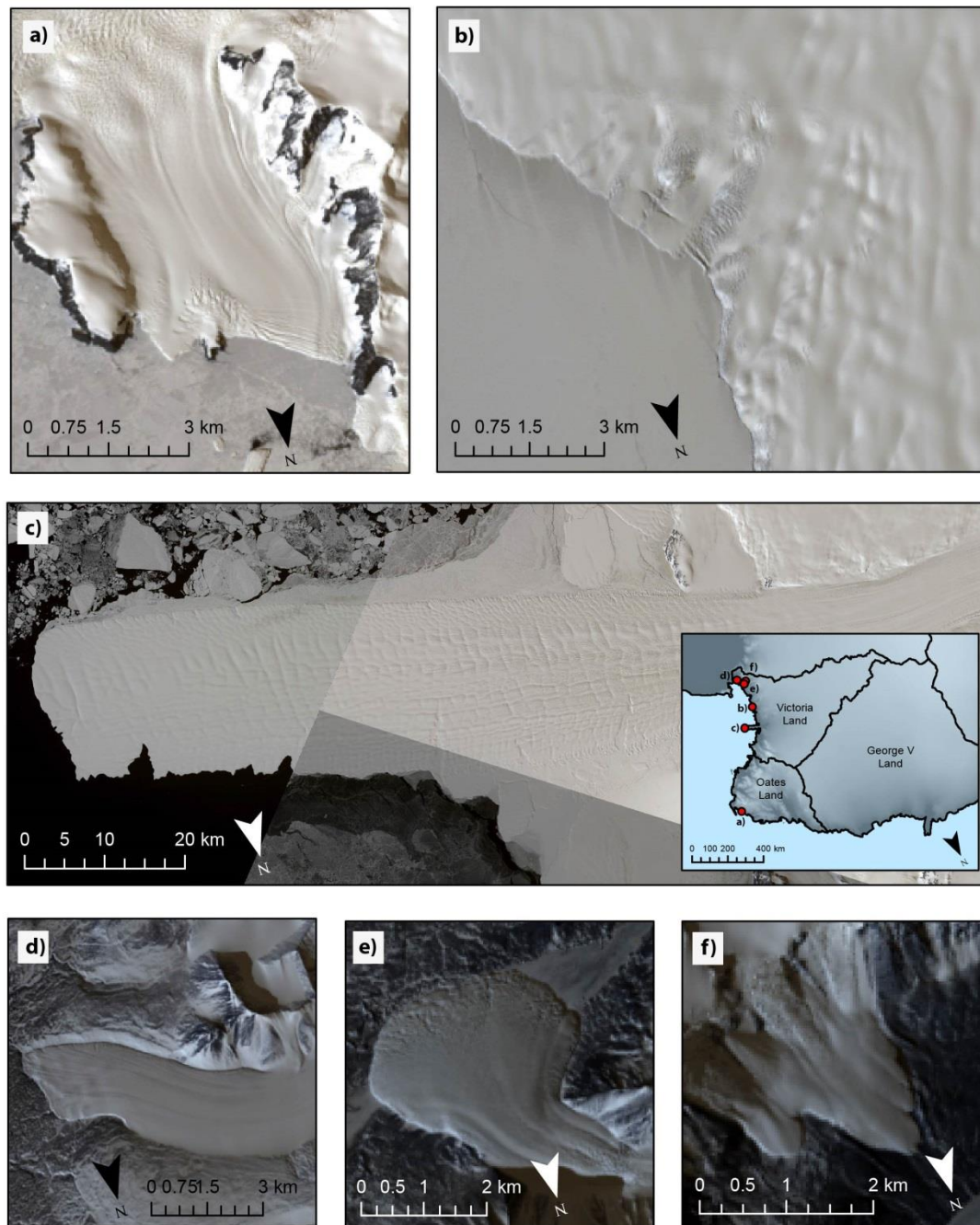
Figure 3.1: Examples of different types of marine-terminating glacier termini: a) floating constrained (FC) terminus (Shipleigh Glacier), b) grounded (G) glacier terminus (Oates Piedmont Glacier), c) floating unconstrained (FU) tongue (David Glacier); and land-terminating glacier termini: d) valley (V) glacier terminus (Hobbs Glacier), e) piedmont (P) glacier terminus (Canada Glacier) and f) lobate (L) glacier terminus (Hughes Glacier). Inset map shows locations of the different glaciers (red circles).
