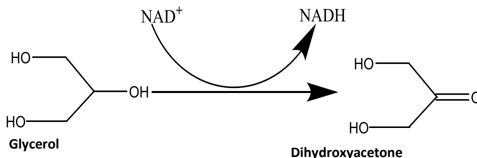
Scheme 5.2: Glycerol oxidation pathway 108 .
