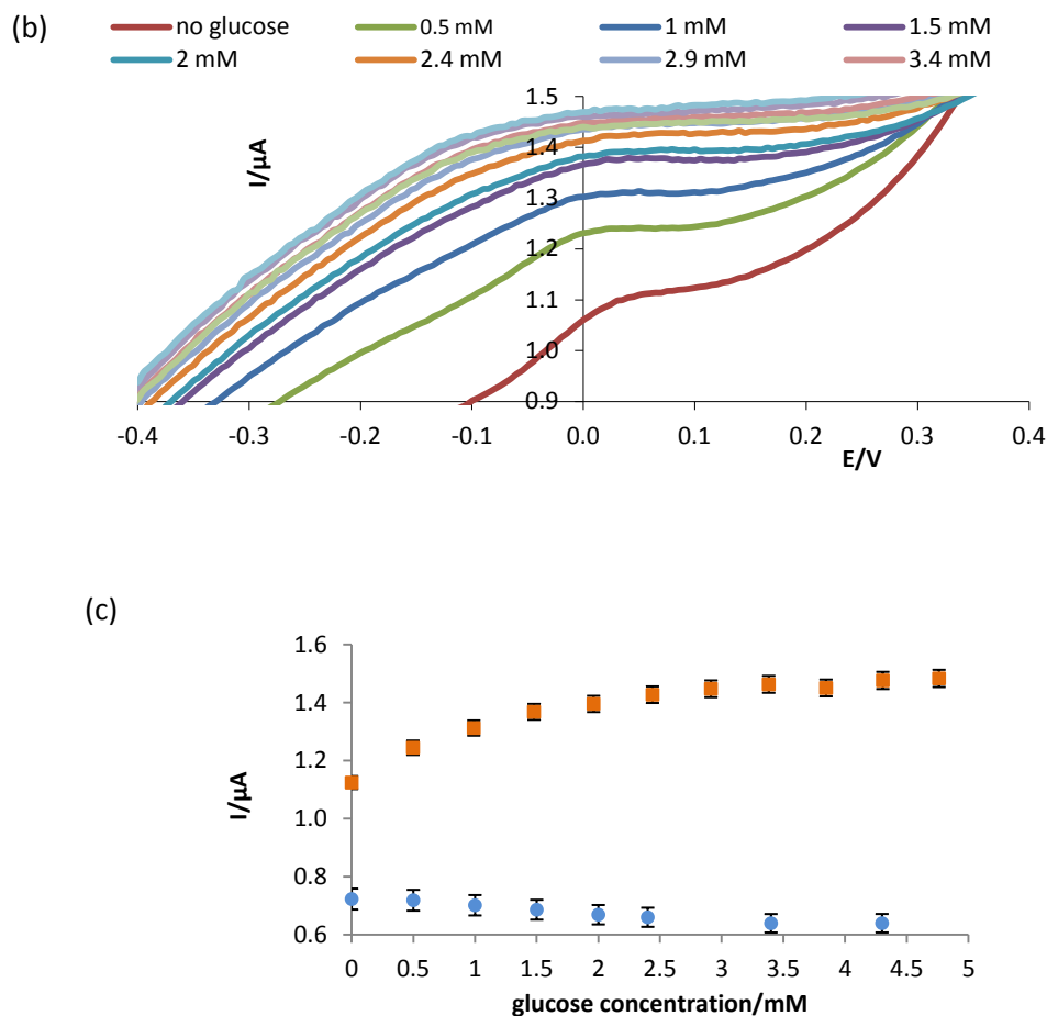
Figure 5.9: (a) CVs for GOx in solution, (b) CVs for immobilised sol-gel/FcAuNP/GOx enzymatic carbon macroelectrode and (c) shows the change in current against glucose concentration plot for GOx in solution (blue circles) and for immobilised sol-gel/FcAuNP/GOx enzymatic macroelectrode (orange square).
