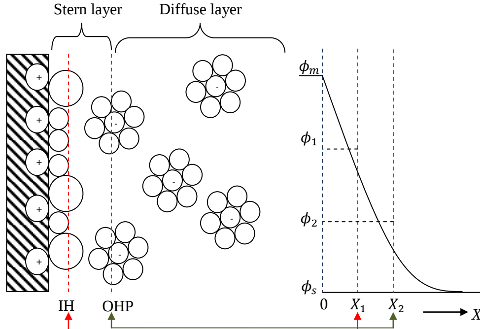
Figure 2.7: Schematic representation of the double layer model.
