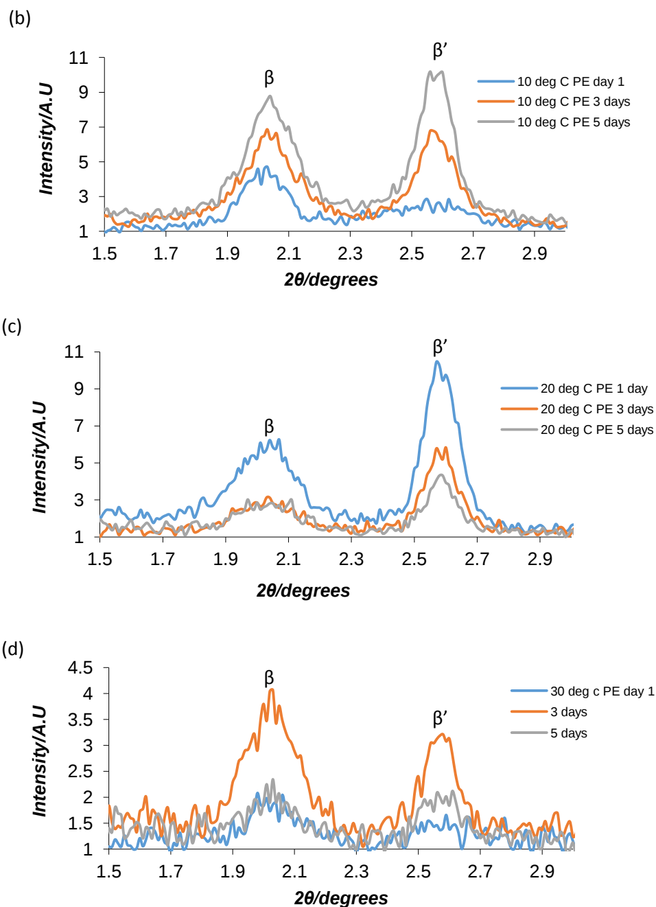
Figure A3.4: SAXS data for soiled polyester (PE) fabrics obtained at temperatures of (a) -10\text{ }^{\circ}\text{C} (b) 10\text{ }^{\circ}\text{C} (c) 20\text{ }^{\circ}\text{C} and (d) 30\text{ }^{\circ}\text{C} over a period of 5 days.
