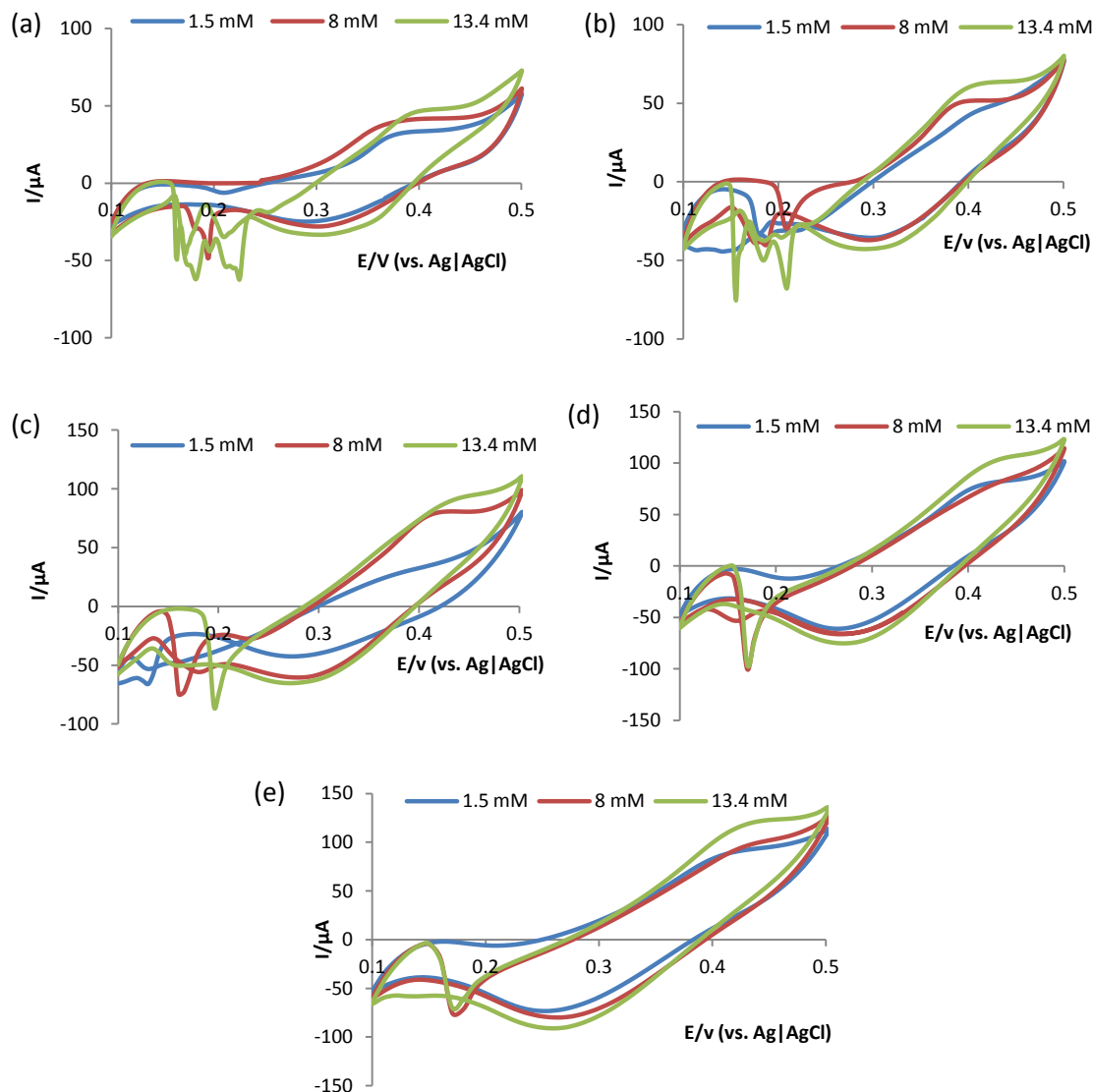
Figure 4.8: CVs showing the transfer and adsorption of 1.5 mM- 13.4 mM of SDBS surfactant, at the aqueous (with LiCl) and 1,2-DCE (with TBATPB) interface at a scan rate of (a) 10 mVs^{-1} , (b) 20 mVs^{-1} , (c) 50 mVs^{-1} , (d) 70 mVs^{-1} and (e) 100 mVs^{-1} .
