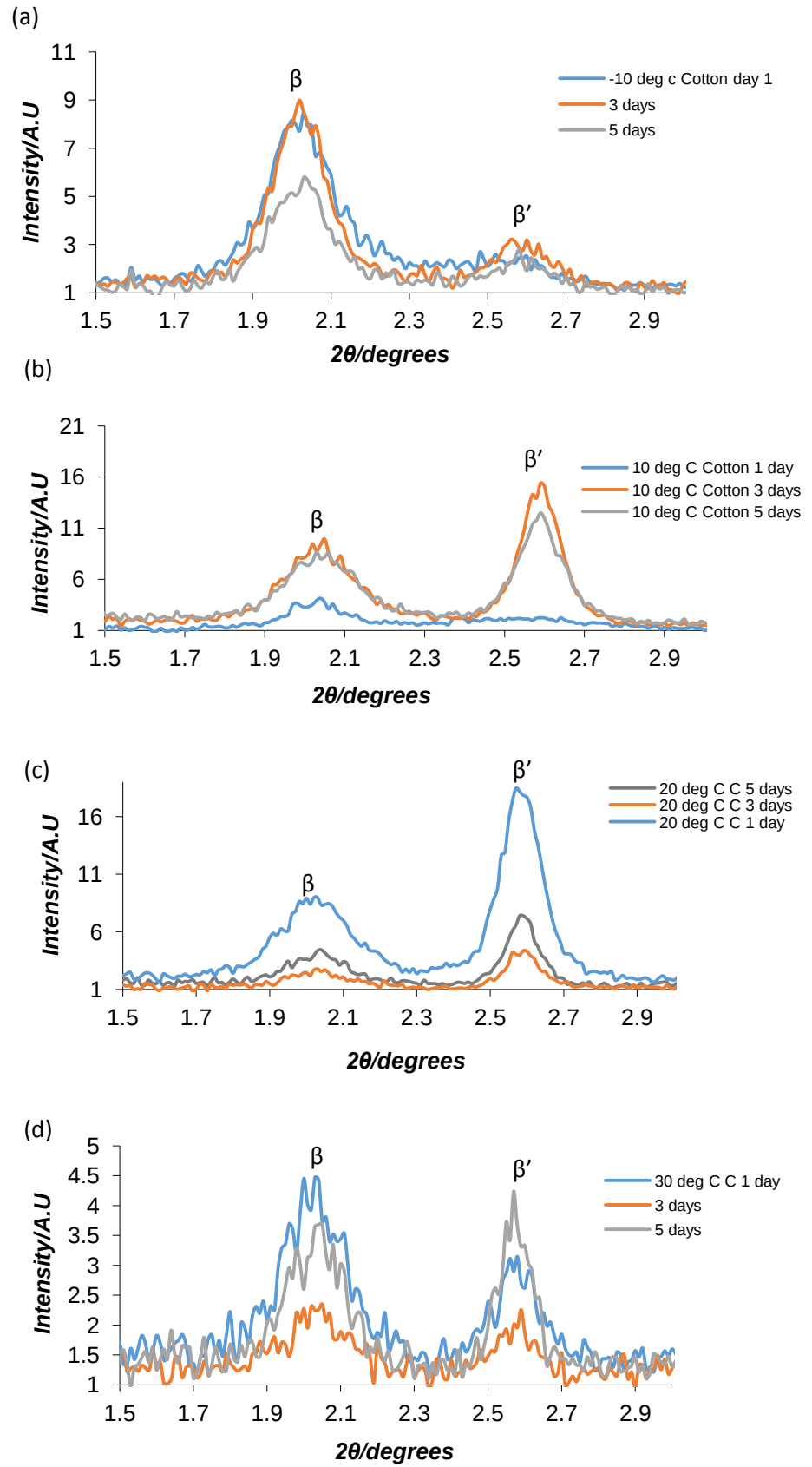
Figure A3.5: SAXS data for soiled cotton (C) fabrics obtained at temperatures of (a) -10 °C (b) 10 °C (c) 20 °C and (d) 30 °C over a period of 5 days.
