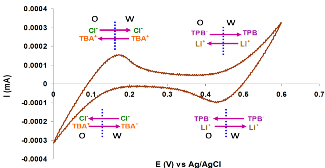
Figure 2.2: A typical voltammogram of polarised ITIES 27 .
