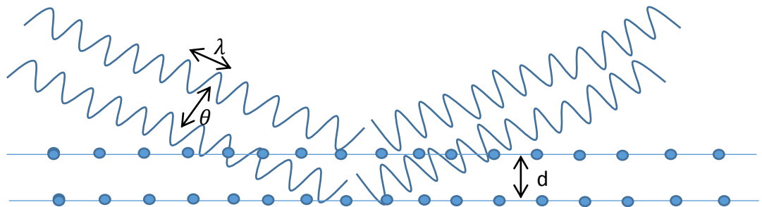
Figure 3.20: Diagram illustrating Bragg's Law 60 .
