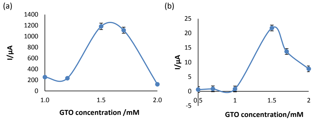
Figure 5.16: shows the change in current against GTO concentration using the data from (a) CVs and (b) CA, for the immobilised sol-gel/FcAuNP/ \text{NAD}^+ - dependent DP and GDH enzymatic SPE biosensor, in the presence of lipase and GTO in solution.
