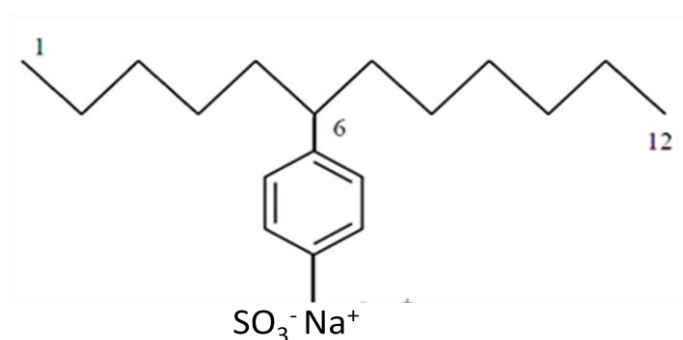
Figure 6.13: Structure of LAS 72 .
