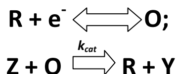
Scheme 5.1: kinetic of the EC' mechanism 69 .
