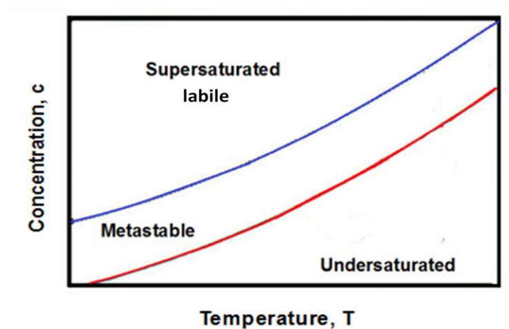
Figure 6.7: showing change in solubility of a compound with concentration and temperature 38 .
