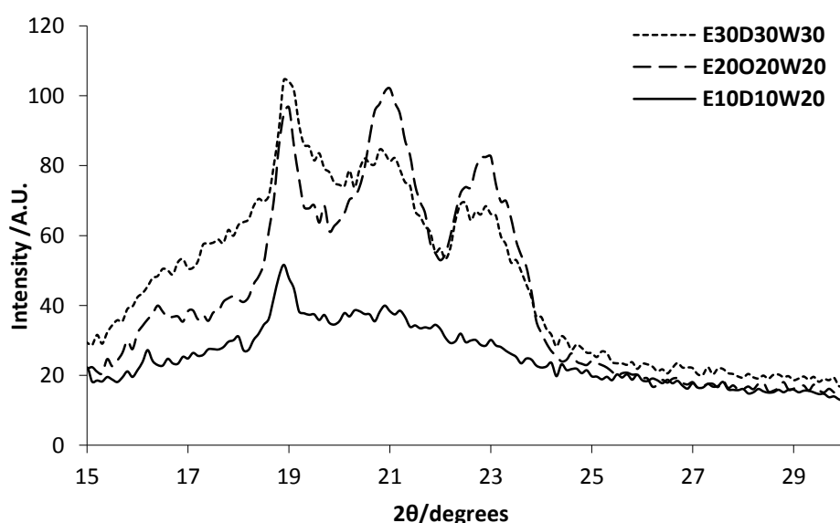
Figure 6.28: WAXS data for the fat globules obtained from the wash water when a high concentration (50 mg/mL) of the C24E3S surfactant was applied.
