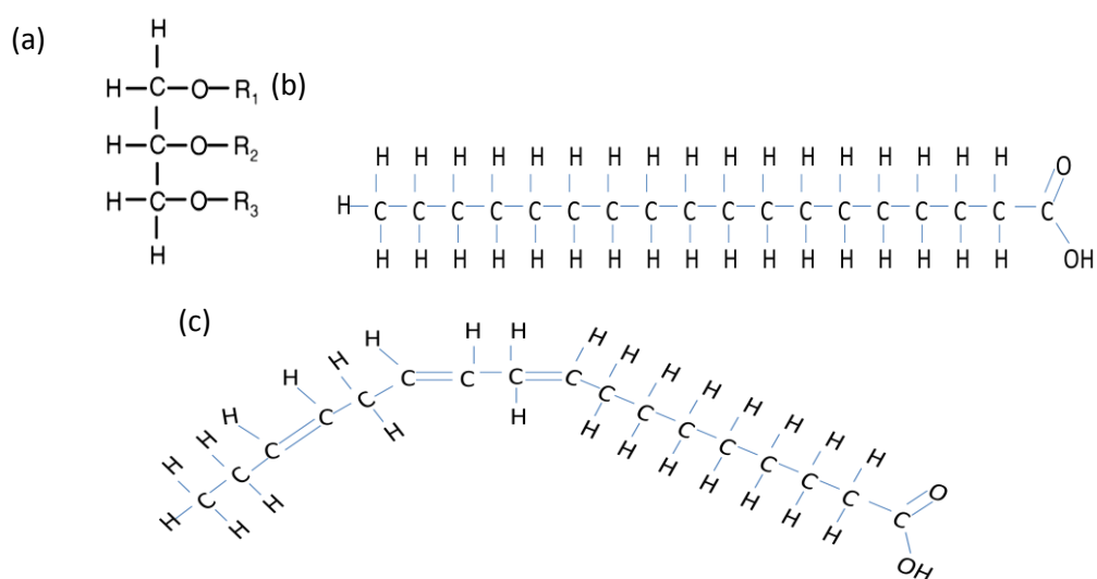
Figure 6.3: molecular structure of (a) a triacylglyceride ( R_1 , R_2 & R_3 are fatty acids) (b) a saturated fatty acid - Stearic acid & (c) an unsaturated fatty acid – Linolenic acid 23 .
