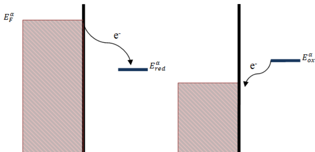
Figure 2.4: A model showing the change in E_F^\alpha upon applying a potential leading to (a) reduction ( E_{red}^\alpha ) and (b) oxidation ( E_{ox}^\alpha ) reaction.
