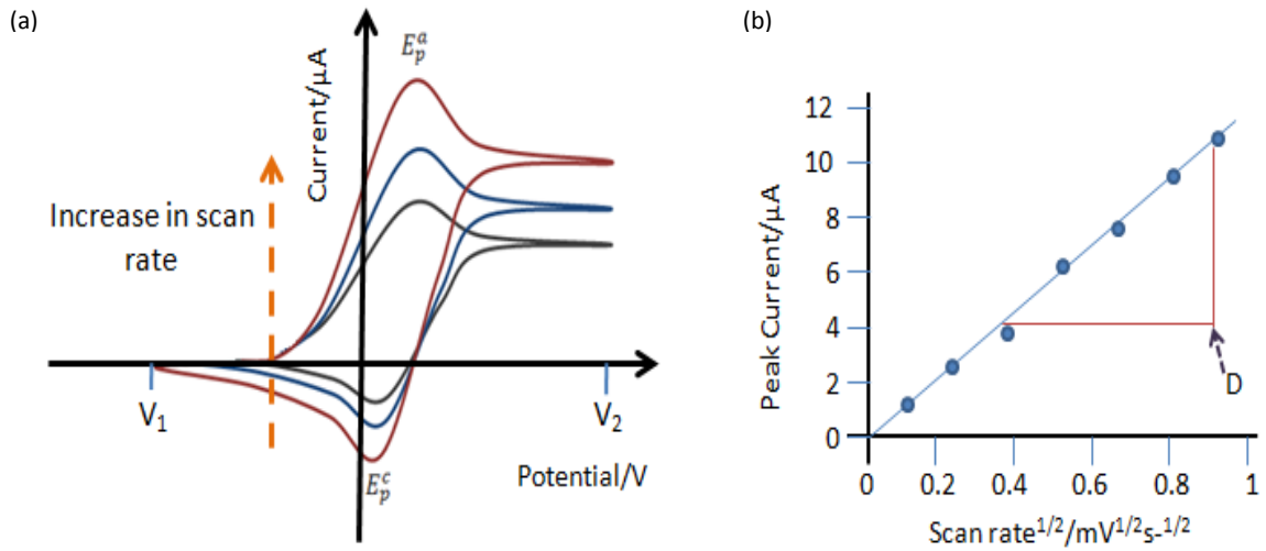
Figure 3.10: (a) Change in scan rate as a function of applied potential and, (b) peak current versus scan rate 1/2 . Where, D is the diffusion coefficient value of the electroactive species (cm 2 /sec).
