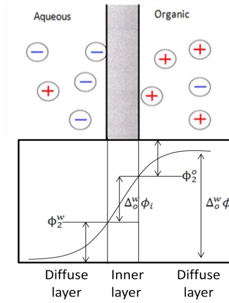
Figure 2.6: Model of ITIES with an inner layer separating the two-space charge regions 59 .
