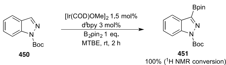
Scheme 41: Borylation of Boc-1H-indazole
