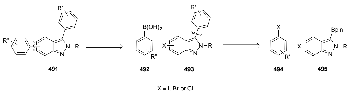
Scheme 42: Retrosynthetic analysis of bis-arylindazoles
