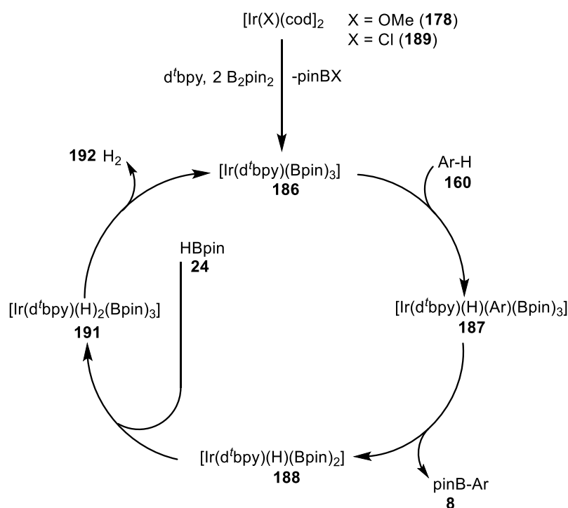
Figure 21: The HBpin-mediated cycle
