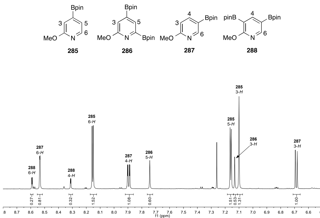
Figure 33: Borylation of 2-methoxypyridine ( 274 ) ( 1 H NMR spectrum of crude product mixture)
