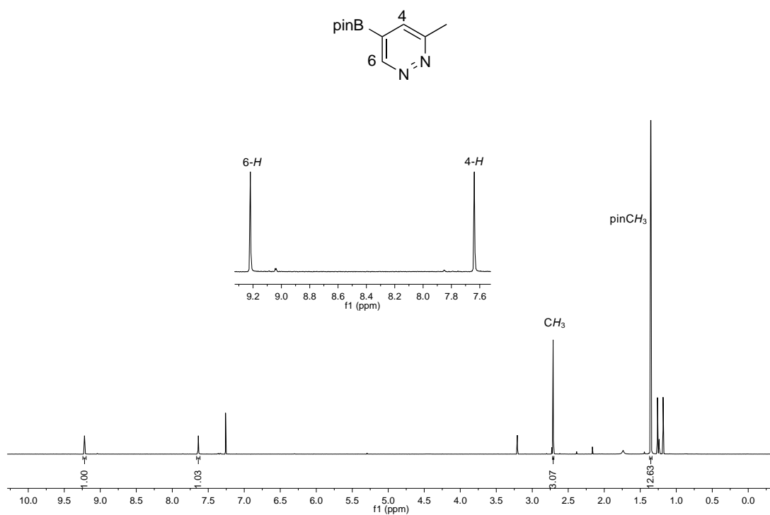
Figure 50: ^1\text{H} NMR spectrum of 3-methyl-5-(Bpin)-pyridazine
