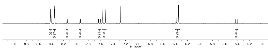
Figure 75: ^1\text{H} NMR spectrum of E/Z isomeric mixture (aromatic enhancement)
