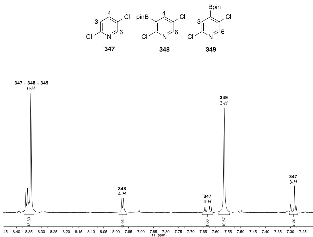
Figure 41: Borylation of 2,5-dichloropyridine ( 347 ) ( 1 H NMR spectrum of crude product mixture)
