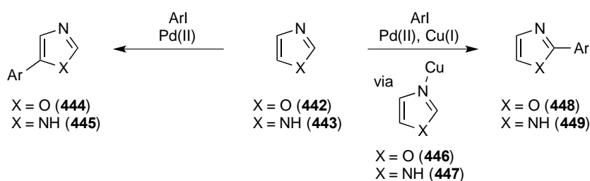
Figure 56: Regioselectivity tuning with Cu(I) salts
