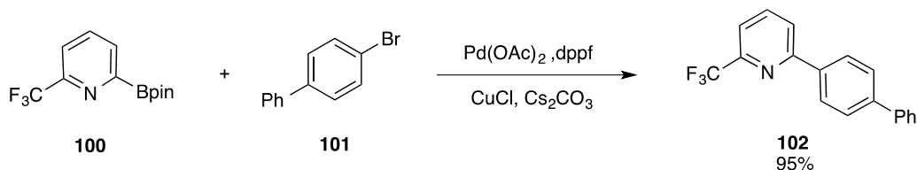
Scheme 9: Application of boronate esters in the cross-coupling of the unstable 2-pyridyl moiety
