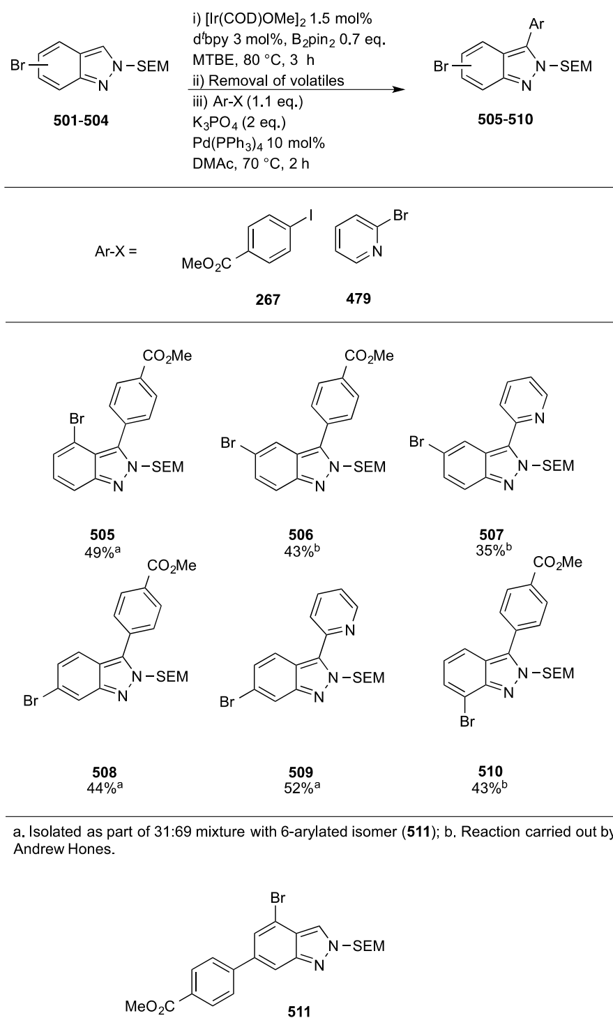
Figure 61: Tandem ‘one-pot’ borylation/Suzuki-Miyaura cross-couplings of bromo-indazoles
