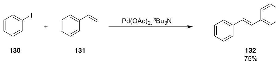
Scheme 11: Seminal Mizoroki-Heck coupling
