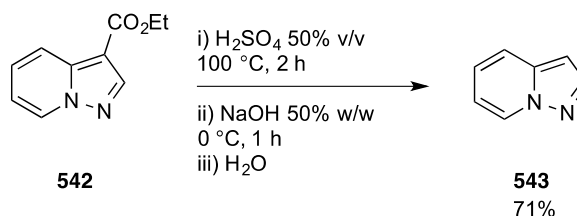
Scheme 48: Synthesis of pyrazolo[1,5-a]pyridine
