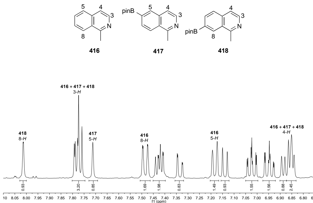
Figure 51: Borylation of 1-methylisoquinoline ( In-situ ^1\text{H} NMR spectrum)
