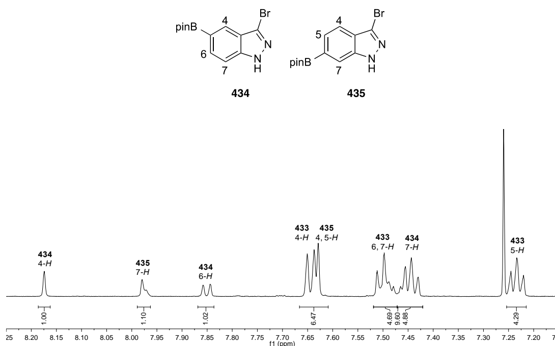
Figure 53: Borylation of 3-bromoindazole ( 433 ) ( 1 H NMR spectrum of the crude product mixture)
