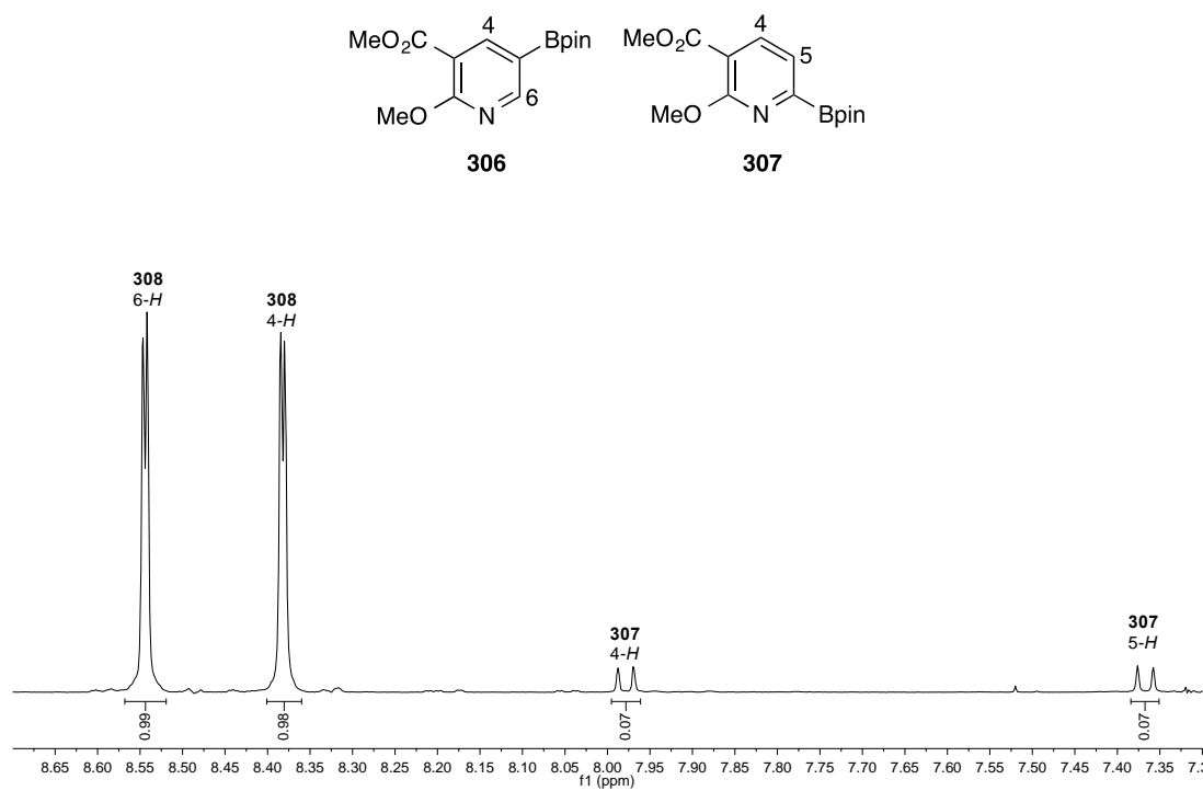
Figure 36: Borylation of methyl-2-methoxynicotinate ( 304 ) ( 1 H NMR spectrum of crude product mixture)
