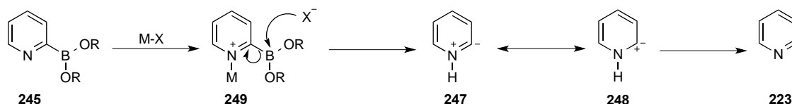
Scheme 26: Mechanism of metal-mediated protodeborylation
