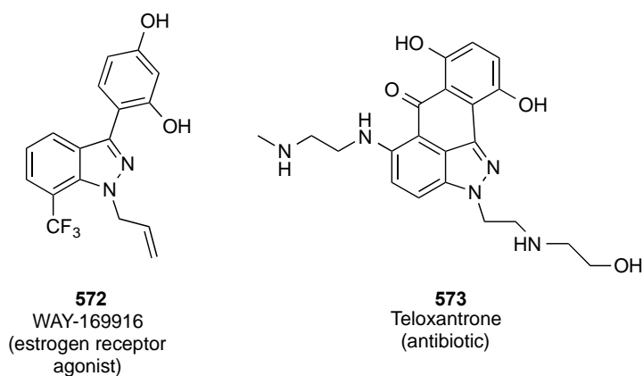
Figure 74: Biologically active 3-aryl indazoles
