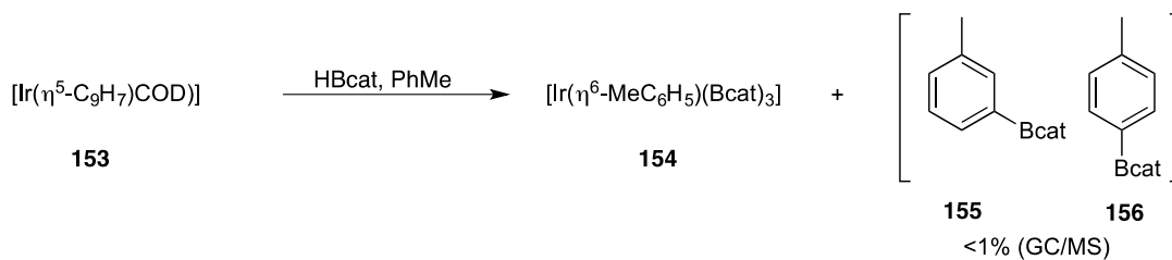
Scheme 16: First reported C-H borylation products
