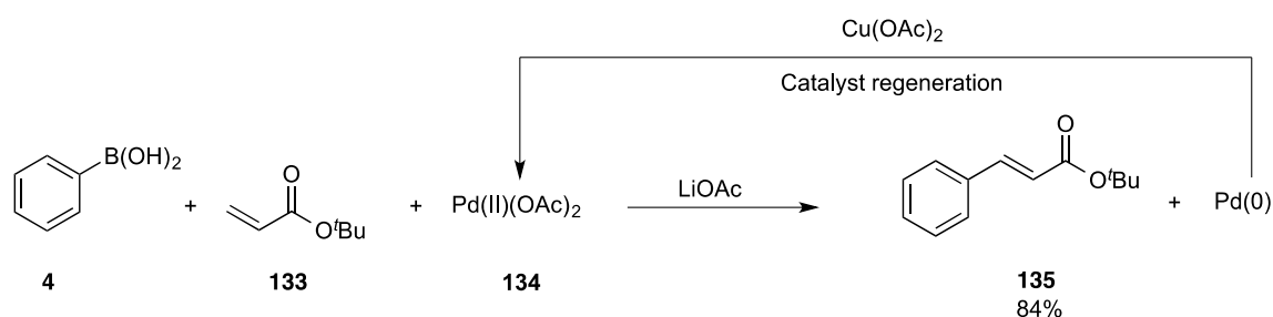
Scheme 12: Pd(II) catalysed oxidative Heck coupling
