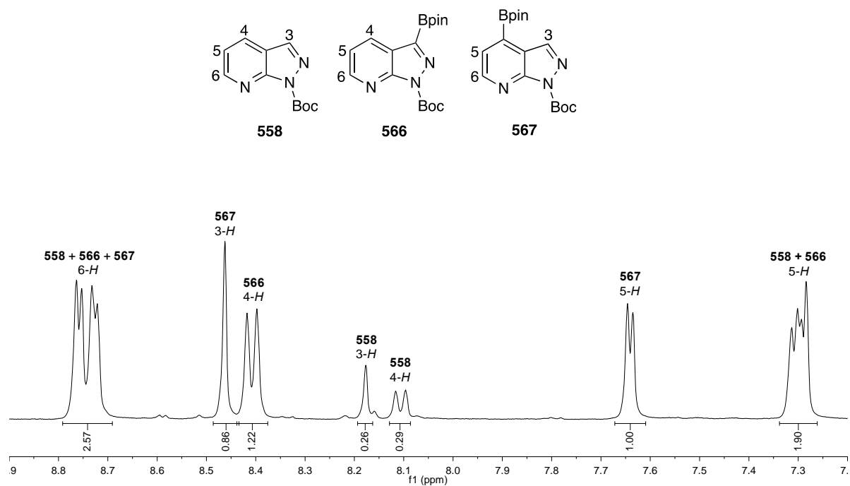
Figure 72: 1 H NMR spectrum of borylation of 7-azaindazole
