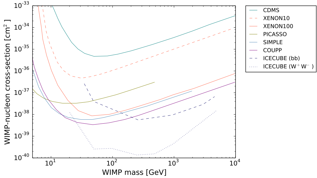
Fig. 1.3.: Exclusion limits on spin dependent WIMP scattering with a proton [34, 35, 43–46]. The results of IceCube are model dependent, representing limits on annihilation to the indicated particle pairs. The neutron limits are similar [30], though XENON100 is strongest, and IceCube present no constraint.
