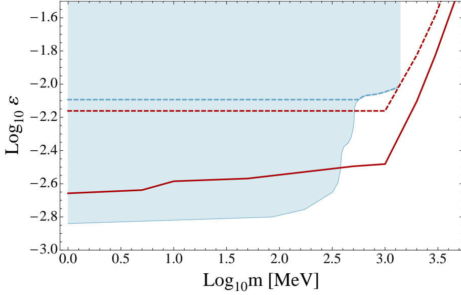
Fig. 5.9: E613 constraints only. The blue shaded area shows a previously existing constraint [242]. The red lines represent the DIS only (dashed) and DIS plus saturation (solid) exclusion regions. The dashed blue line estimates the previous constraint without production from meson decays.
