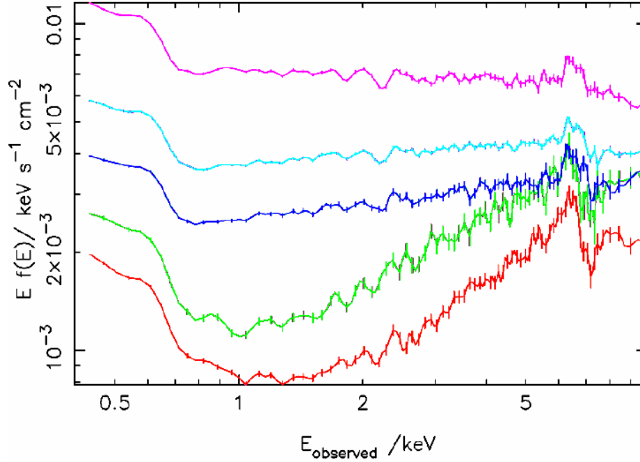
Figure 3.7: Intensity-sorted X-ray spectra of the NLS1 MRK 766, showing systematic spectral changes with luminosity, from Miller et al. (2007).
