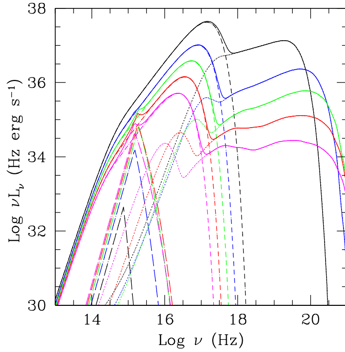
Figure 4.2: Model SEDs, with truncated disc (short dashed line), hot flow cyclo-synchrotron emission (long dashed line) and Comptonisation of both disc and cyclo-synchrotron seed photons (dotted line) for increasing truncation radius: 20 R_g (black), 35 R_g (blue), 50 R_g (green), 70 R_g (red) and 100 R_g (magenta). Solid line shows sum of all three components.
