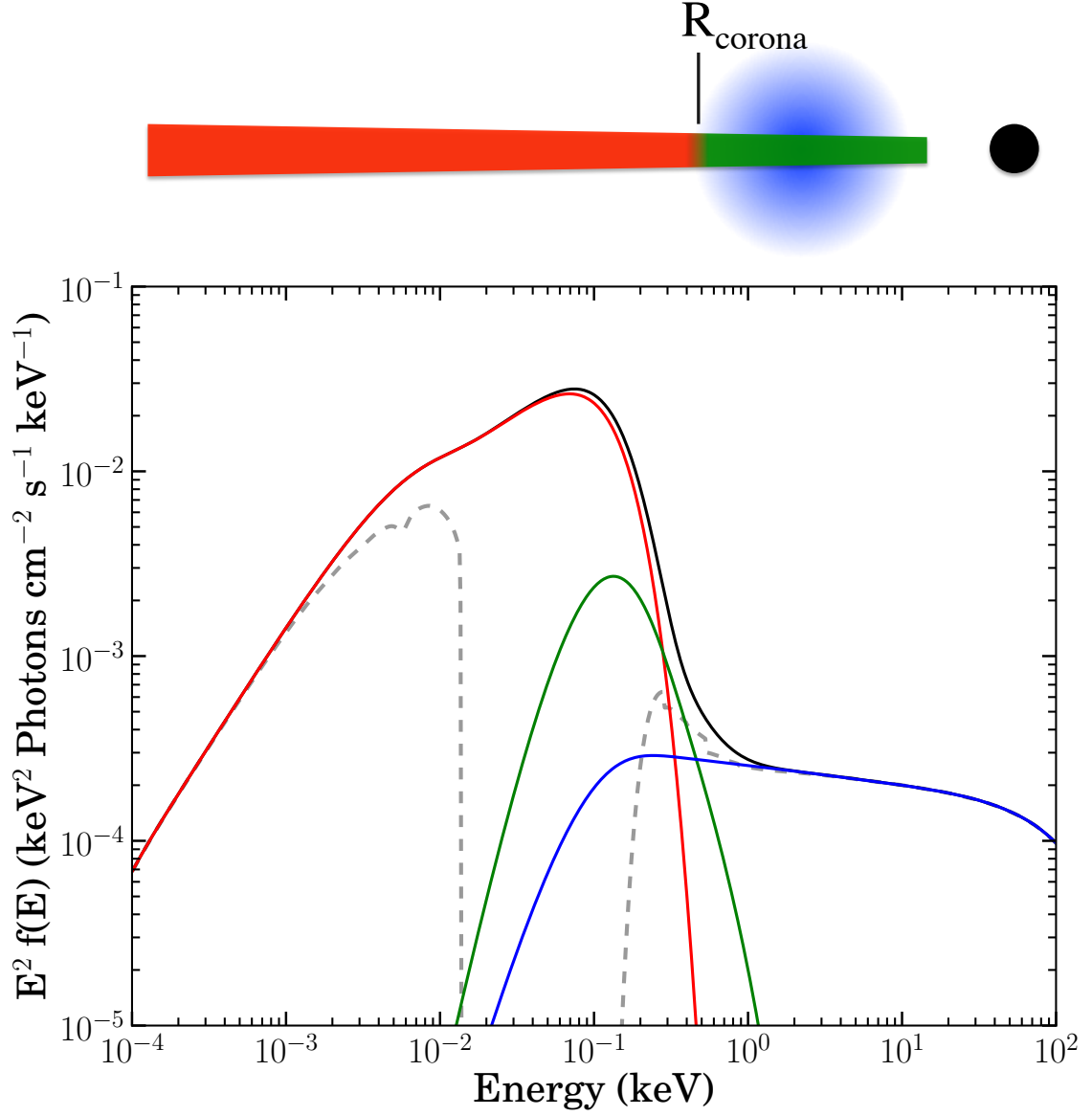
Figure 3.6: Schematic showing AGN spectral components together with proposed accretion flow geometry, including emission from a truncated accretion disc (red), optically thick soft excess Comptonising region (green) and optically thin Comptonising corona (blue). Black line shows total spectrum, grey dashed line shows spectrum after including external absorption. From Collinson et al. (2015).
