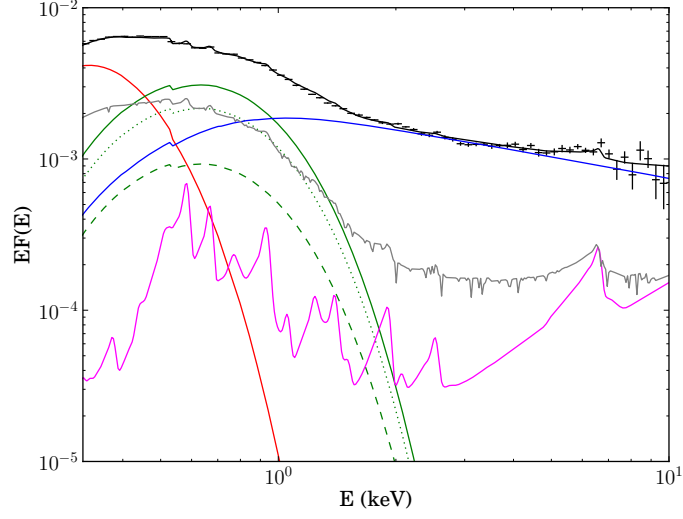
Figure 8.12: Spectral decomposition for PG1244+026: disc (red), soft excess (green, with dashed line for intrinsic emission, dotted line for reprocessed emission, solid line for total), corona (blue), reflection (magenta), total (black). Data points show time averaged spectrum (OBS ID: 0675320101). Grey line shows an example of the spectrum after introducing absorption by intervening clouds.
