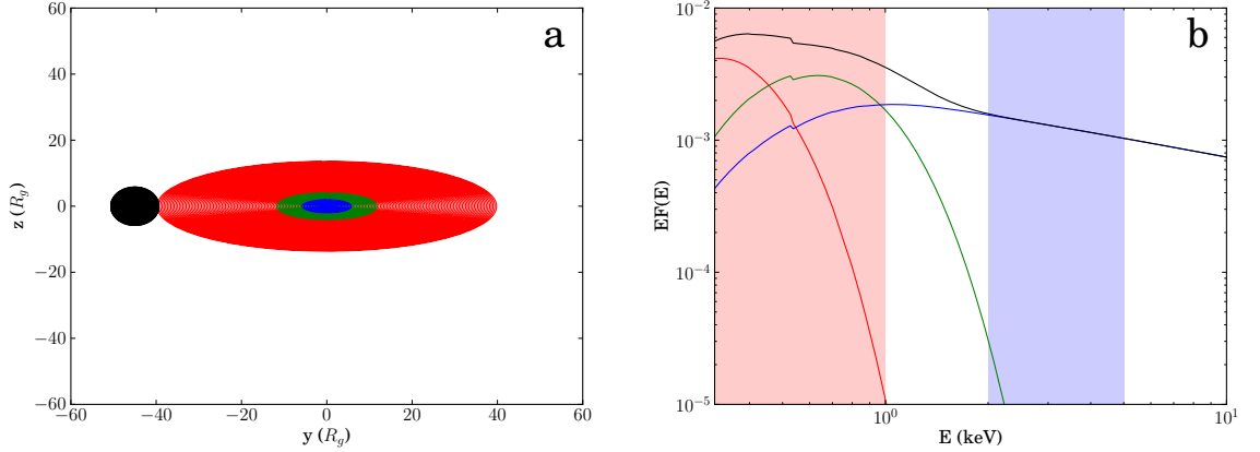
Figure 8.1: a). Physical location of accretion flow model components, as viewed at high inclination ( i = 70^\circ ): disc (red), soft excess (green), corona (blue), obscuring cloud (black). For simplicity we have approximated the geometry of the accretion flow as a flattened disc. b). Spectrum emitted by each component, with total spectrum shown in black, and hard and soft bands shaded in blue and red respectively.
