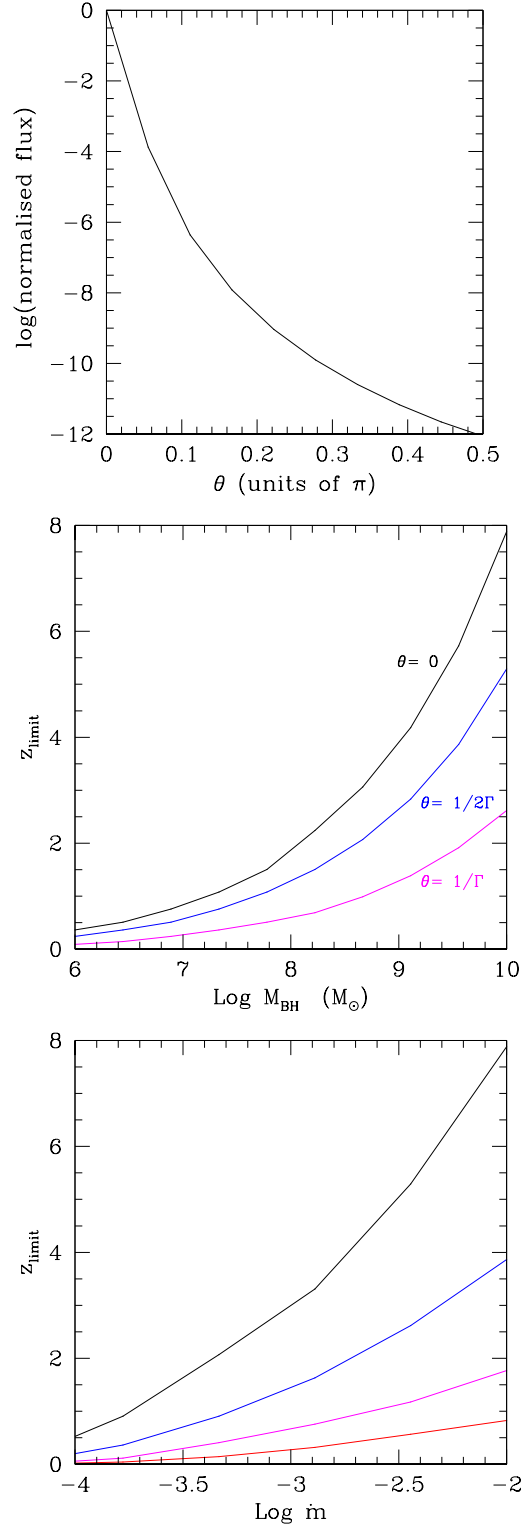
Figure 5.3: a). Decrease in observed flux with increasing viewing angle, where \theta is measured in radians from the jet axis, for \Gamma = 15 . b). Redshift limits for Fermi visible BL Lacs as a function of black hole mass, for increasing viewing angle and \dot{m} = 10^{-2} . c). Redshift limits for Fermi visible BL Lacs as a function of accretion rate, for M_{\text{BH}} = 10^7 (red), 10^8 (magenta), 10^9 (blue) and 10^{10} M_{\odot} (black) and \theta = 0 .
