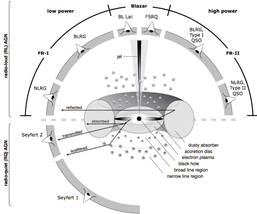
Figure 3.4: Unified model of active galactic nuclei, from Beckmann & Shrader (2012).
