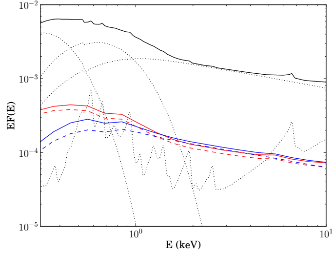
Figure 7.11: 4–10 keV covariance spectra for low frequencies ( 2.3 \times 10^{-5} - 7.3 \times 10^{-5} Hz, red) and high frequencies ( 2.3 \times 10^{-4} - 7.3 \times 10^{-4} Hz, blue) for the model including reprocessing on the soft excess (solid red and blue) and model including reprocessing on both the soft excess and the disc (dashed red and blue). Black solid line shows total spectrum, dotted lines show model components.
