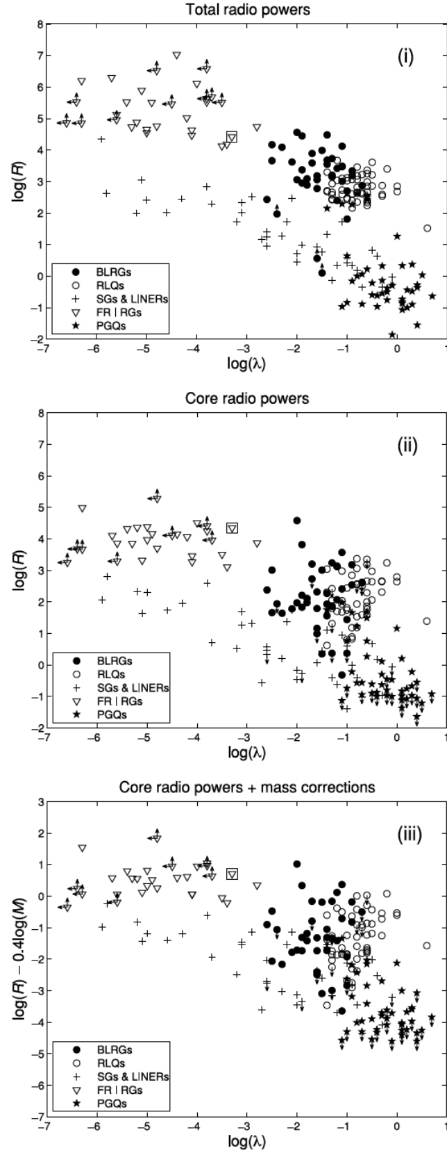
Figure 3.13: Radio loudness (where R = L_{5\text{ GHz}}/L_{4400\text{ \AA}}^\circ ) as a function of Eddington ratio calculated using i). total radio luminosity, ii). only core radio luminosity and iii). core radio luminosity plus a correction for AGN mass, from Broderick & Fender (2011).
