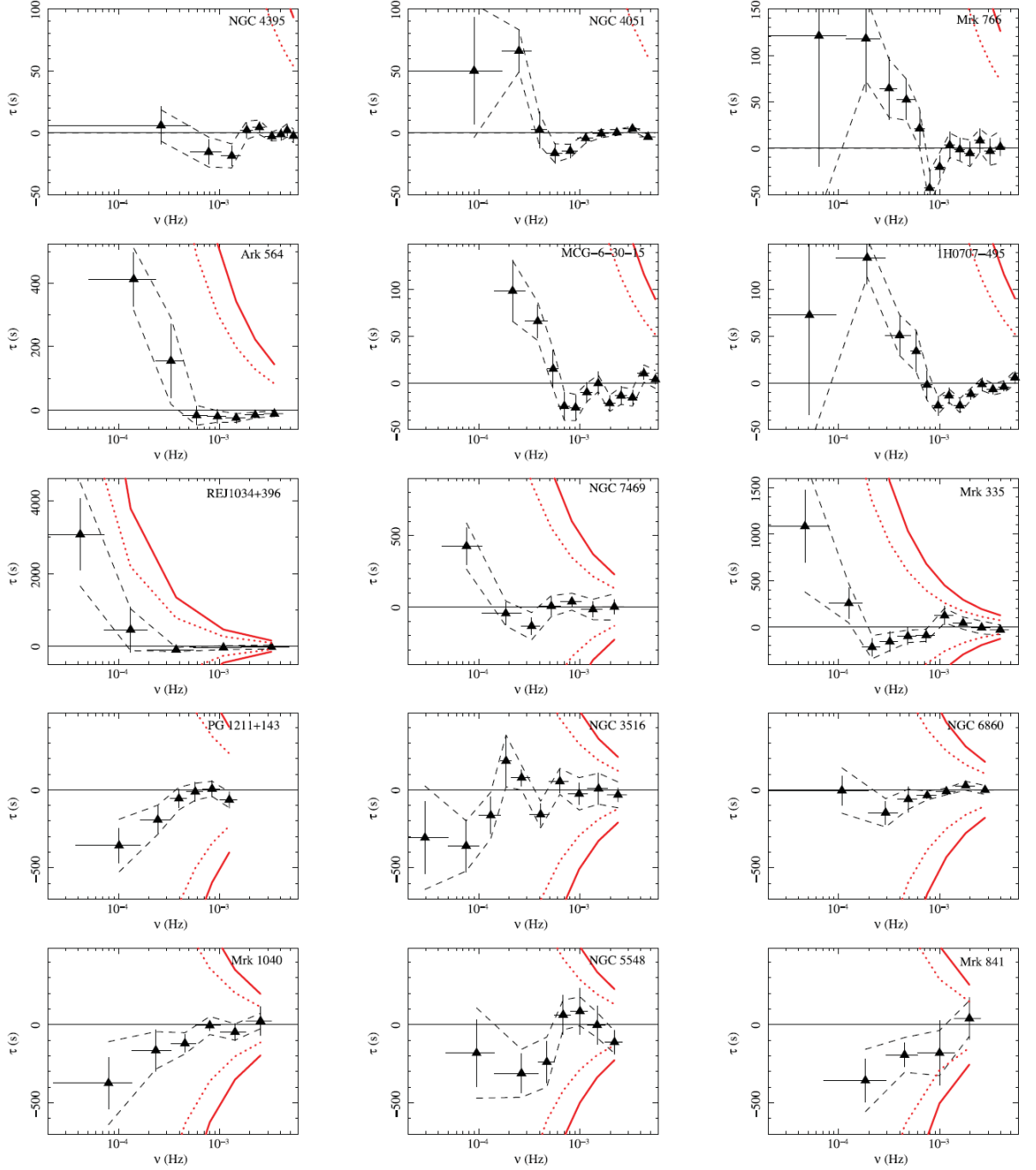
Figure 3.11: Lag-frequency spectra for a sample of AGN, where positive lags indicate the hard X-ray band lagging the soft X-ray band, from De Marco et al. (2013). Dashed black lines bound the 1\sigma confidence levels for the observed lags. Red solid lines show the range of allowed lag values at each frequency ( \tau = -\nu/2, +\nu/2 ). Red dotted lines show the standard deviation of a uniform distribution defined on the same interval of lag time permitted values — Poisson noise errors become important when the spread on the measured lags (defined by the 1\sigma confidence levels) approaches this line.
