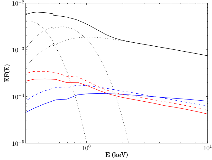
Figure 7.5: 4 – 10 keV covariance spectra for low frequencies ( 2.3 \times 10^{-5} - 7.3 \times 10^{-5} Hz, red) and high frequencies ( 2.3 \times 10^{-4} - 7.3 \times 10^{-4} Hz, blue) for the propagating model including spectral pivoting of the power law (solid red and blue) and the propagating model without spectral pivoting (dashed red and blue). Black solid line shows total spectrum, dotted lines show model components.
