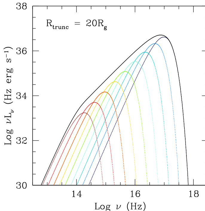
Figure 2.4: Model disc spectrum around a 10 M_{\odot} black hole with R_{trunc} = 20 R_g . Each annulus of the disc radiates as a black body with temperature increasing as radius decreases. The peak disc luminosity is therefore determined by the inner radius of the disc.
