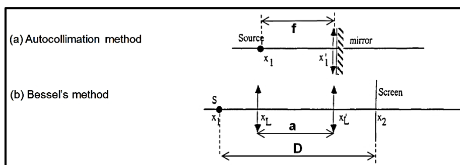
Figure 2.26 Methods of finding focal length( f ) (Séré et al., 1993, p.429)
