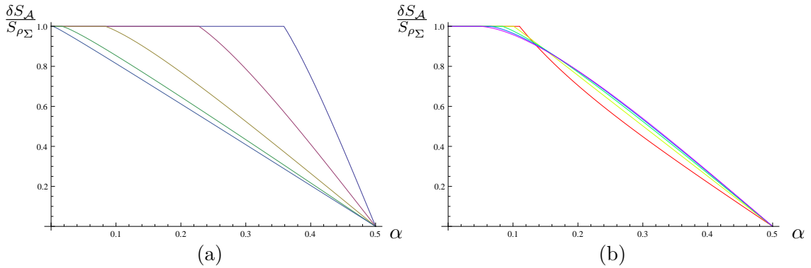
Figure 2.5: Entanglement entropy plateaux for Schwarzschild- AdS black holes dual to thermal field theories. (a). Behaviour in Schwarzschild- AdS_5 for varying r_+ . From right to left we have r_+ = \frac{1}{4} (blue), r_+ = \frac{1}{2} (purple), r_+ = 1 (yellow), r_+ = 2 (green) and r_+ = 4 (blue). (b). Dimension dependence of the plateaux, at the Hawking-Page transition point RT = \frac{d-1}{2\pi} for d = 2, 3, 4, 5, 6 (red, yellow, green, blue, purple respectively). Note that the horizon size is related to the temperature via r_+ = \frac{2\pi}{d} \left( RT + \sqrt{(RT)^2 - \frac{d(d-2)}{4\pi^2}} \right) .
