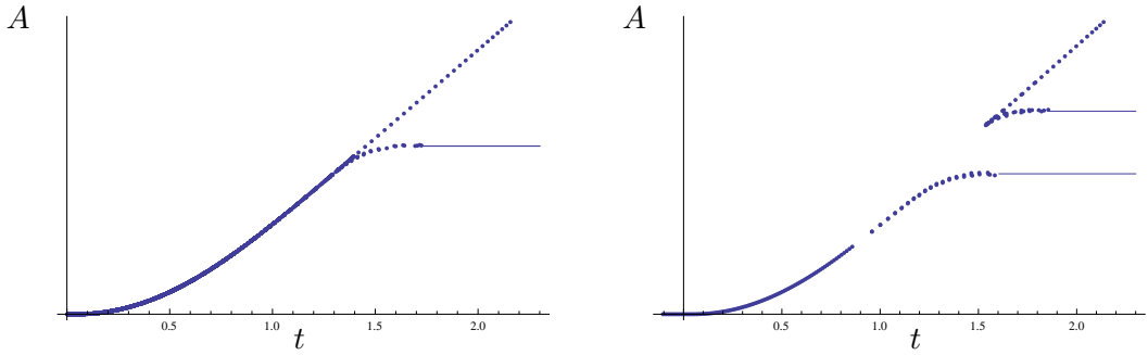
Figure 3.20: Thermalization of entanglement entropy for a hemisphere (left), and a slightly smaller region (right). Data points for extra branches of surfaces are shown, and can be seen to have larger areas.
