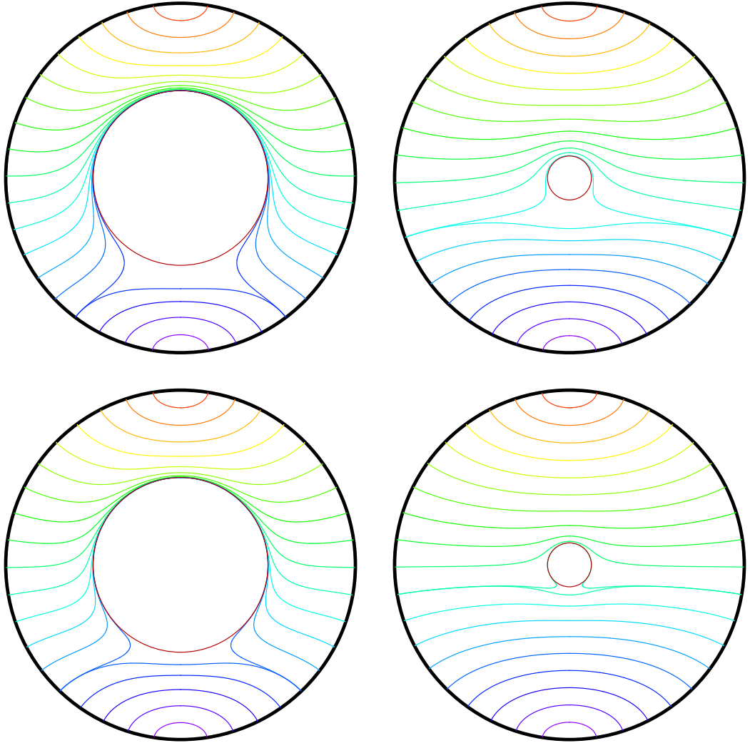
Figure 2.4: Minimal surfaces for r_+ = 1 (left) and r_+ = 0.2 (right) black holes in Schwarzschild- AdS in 3+1 (top) and 4+1 (bottom) dimensions, analogous to the plots of fig. 2.1. In each panel, the thick black circle represents the AdS boundary, and the thin red circle the black hole horizon. The boundary region \mathcal{A} is centered at \theta = 0 (North Pole) which is plotted on top. Further plots with other black hole sizes and higher dimensions can be found with the submission.
