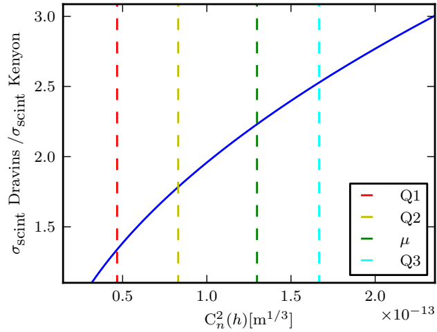
Figure 4.2: Applying an average atmosphere estimate to calculate the noise due to scintillation causes the scintillation noise to be underestimated by a factor of 2 on average for the turbulence profiles measured on La Palma. This is seen from the intersection of the mean line with the ratio of \sigma_{\text{scint Dravins}} / \sigma_{\text{scint Kenyon}} . The red, yellow, green and cyan dashed lines indicate the C_n^2 profiles for the first quartile, second quartile (median), mean and third quartile of the seeing distribution respectively.
