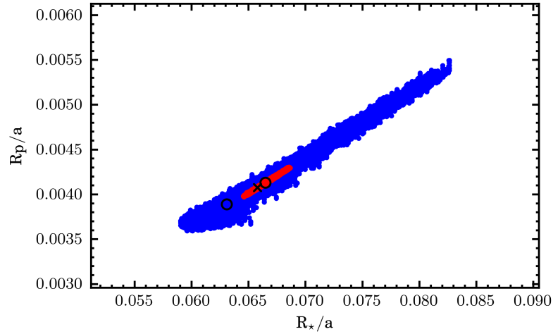
Figure 4.24: The distribution of the results from the MCMC runs for fitting the light curve of HAT-P-11b in the I band for the planetary radius, R_p/a against the stellar radius, R_{\star}/a . The blue and red points show the distribution of the results with, and without the presence of scintillation, respectively. The blue and red circled points show the mean of the respective distributions, while the black cross shows the starting parameters based on which the the model light curve was produced.
