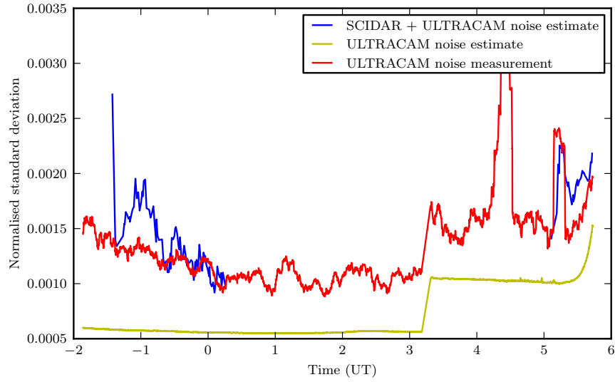
Figure 6.8: Comparison between predicted and measured scintillation from ULTRACAM on 2013-07-20. The red line shows the normalised standard deviation of the measured flux from ULTRACAM. The prediction from SCIDAR (blue) takes into account scintillation, which is scaled according to exposure time, telescope diameter and airmass of the observation, and the predicted noise from ULTRACAM. The predicted ULTRACAM noise includes photon noise and the small amount of system noise in ULTRACAM, shown in yellow.
