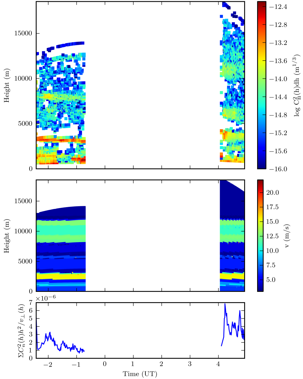
Figure 6.5: Atmospheric data for the night of 2013-07-20 obtained using SCIDAR on the 1.0m Jacobus Kapteyn Telescope. The top panel shows the measured C_n^2 profile with height. Data points with C_n^2 weaker than 10^{-16} \text{ m}^{2/3} have been removed for clarity. The middle panel shows the determined average wind velocity for the layers for each night. The bottom panel shows the calculated sum of C_n^2(h) h^2 / v_{\perp} from the information in the top two panels.
