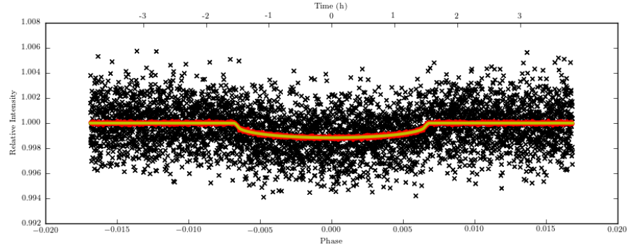
Figure 4.22: Synthetic light curve of the HD 97658b transit in the V band, for a 4.2m telescope under seeing conditions corresponding to an r_0=10\text{cm} at 10km. The yellow line shows the simulated light curve and the black crosses indicate simulated data points with photon noise and scintillation based on a 4.2m telescope with a 6s exposure time. The red dots show a light curve without any scintillation noise present, only photon noise.
