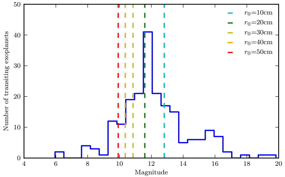
Figure 4.10: Histogram showing the V-band magnitude distribution of known transiting exoplanets. Scintillation noise dominates to the left of the vertical dashed lines, for a 0.5m telescope.
