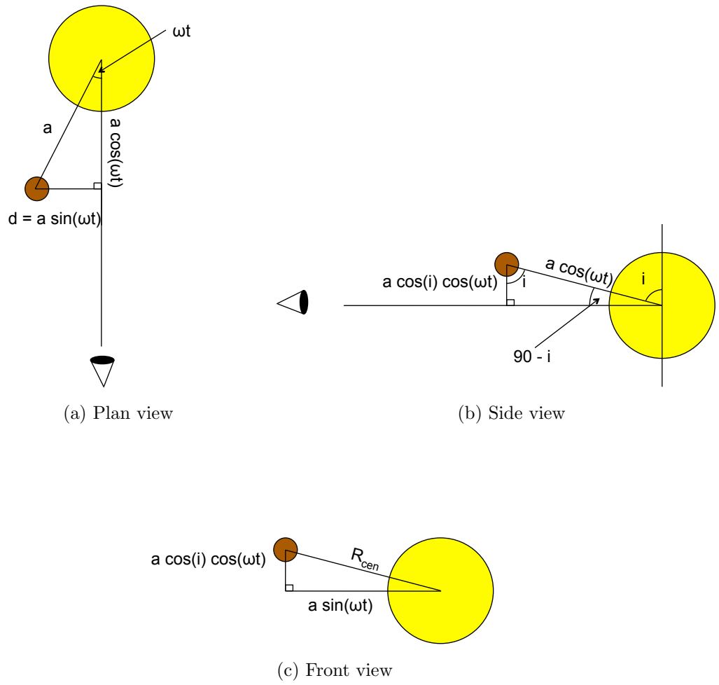
Figure 2.4: Projected planet-star separation for numerical calculation of area obstructed during a transit. Diagrams based on [121].
