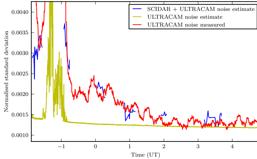
Figure 6.13: Comparison between predicted and measured scintillation from ULTRACAM on 2014-03-16 in the r' band. The red is line shows the normalised standard deviation of the measured flux from ULTRACAM. The prediction from SCIDAR (blue) takes into account scintillation, which is scaled according exposure time, telescope diameter and airmass of the observation, and the predicted noise from ULTRACAM. The predicted ULTRACAM noise includes photon noise and the small amount of system noise in ULTRACAM, shown in yellow.
