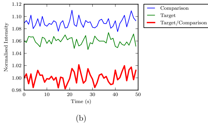
Figure 5.2: False-colour images of two simulated, 1s exposure images of a star with a photometry aperture in red demonstrating the process of differential aperture photometry (figure a). The intensities have been arbitrarily offset for clarity. The arrow shows some of the speckles falling outside of the photometry aperture due to seeing and scintillation. Figure b shows the corresponding intensity variations measured. As we are only investigating the effect of speckle noise in this section, effects due to shot noise from the target and sky, and detector noise have not been included. The red line shows the final intensity measured after performing differential photometry. The intensities have been arbitrarily offset for clarity.
