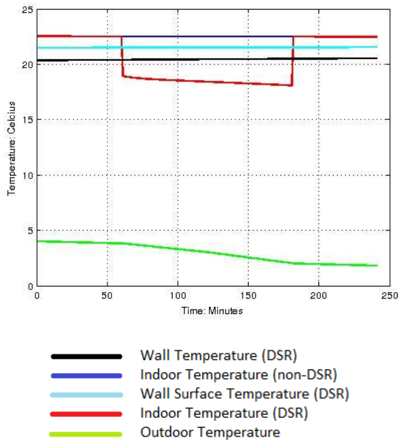
Figure 37: Deviation of temperatures during DSR
