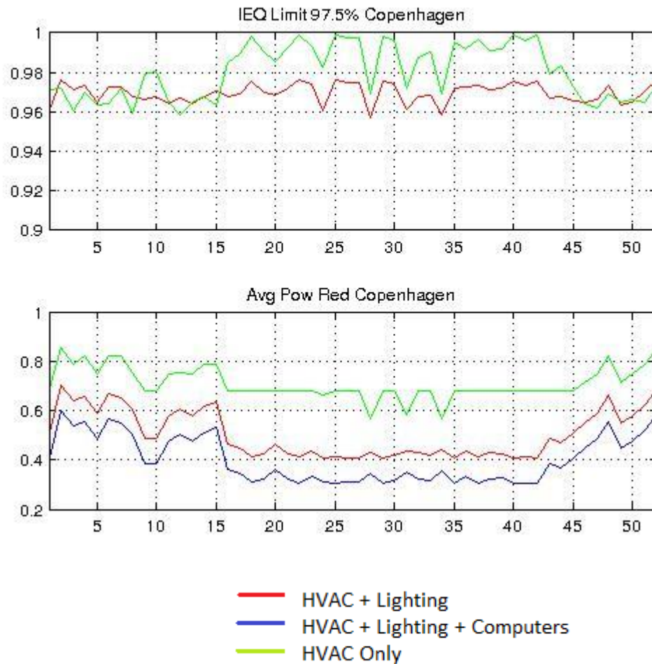
Figure 55: Copenhagen simulation result for 97.5% IEQ.
