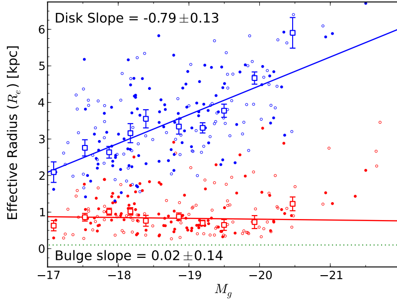
Figure 5.4: As Figure 5.2: bulge (red) and disk (blue) effective half-light radii ( R_e ; kpc) measured from g band (analysis sample) galaxy models plotted against the corresponding absolute (bulge + disk) magnitudes ( M_g ).
