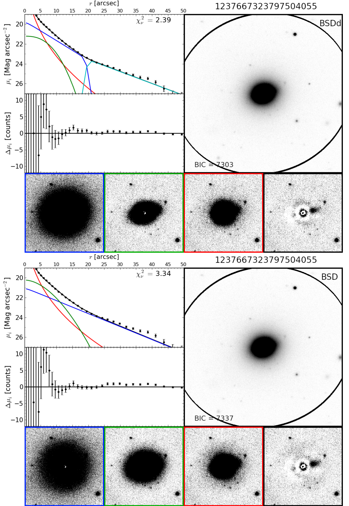
Figure 7.12: An example galaxy best fit by a BSDd model (SDSS DR8 ObjID 1237667323797504055). As Figure 7.5 for a BSDd model ( top : bulge = red, bar = green, inner/outer disk = blue/cyan), and the corresponding BSD model ( bottom : bulge = red, bar = green, disk = blue).
