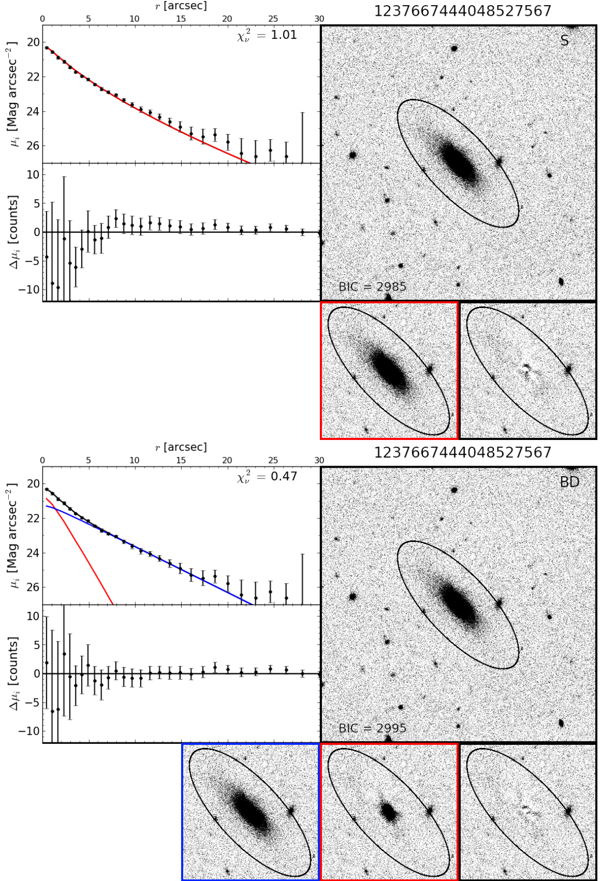
Figure 7.5: An example galaxy best fit by an S model (DR8 ObjID 1237667444048527567): Surface brightness profiles ( \mu_i ), residuals ( \Delta\mu_i ), and i band thumbnails for the S model ( top: Sérsic = red), and the corresponding BD model ( bottom: bulge = red, disk = blue). Small images depict isolated model components (border colours \equiv \mu_i plot), and the total residual (black borders). The target ellipse is noted in black in all thumbnails, and 1D \chi^2_\nu (major axis) and 2D BIC values are included for both models.
