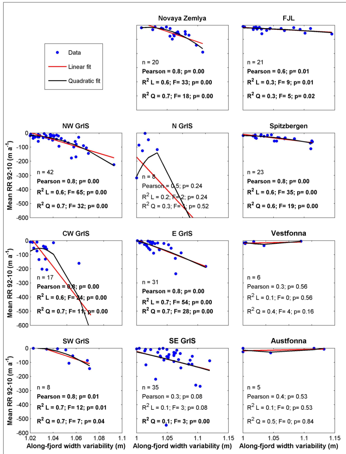
Figure 6.11. Scatter plots of along-fjord width variability versus mean retreat rate (m a -1 ) between 1992 and 2010. Plots are divided according to region and each plot includes all study glaciers within that region with continuous fjord walls (top left). This encompasses approximately 75 % of the total number of study glaciers. Width variability was measured between the least
