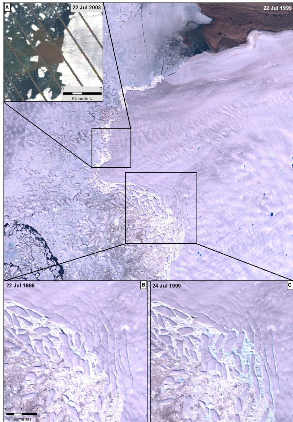
Figure 5.6: Subglacial meltwater plume and the pattern of iceberg calving / rift formation on northern section of HG's terminus. A) Turbid meltwater plume exiting the calving front. B) & C) Large tabular icebergs calving back to rifts over a two day period.
