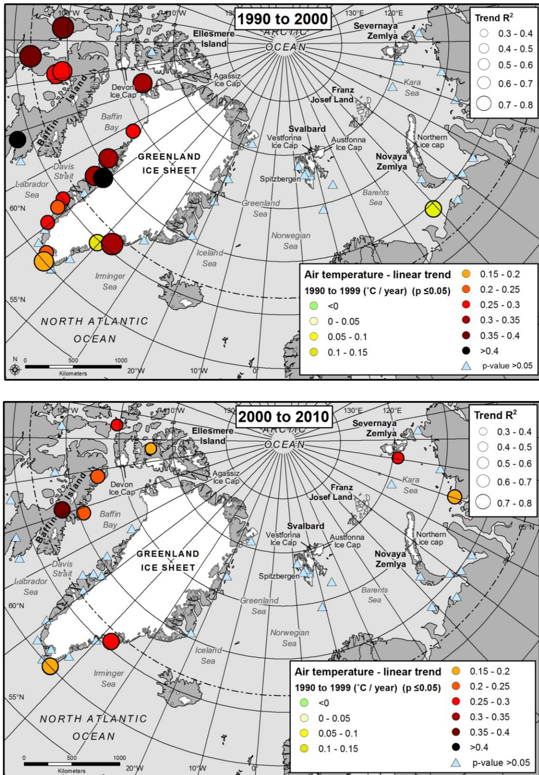
Figure 6.8. Linear trend in mean annual air temperatures between 1990 and 2010 for selected Arctic meteorological stations. Symbol colour shows the magnitude of the linear trend in ^{\circ}\text{C} per year between 1990 and 2010. Symbol size shows the R^2 value of the relationship. Trends are shown only for locations where the p-value associated with the F-statistic was \leq 0.05 , i.e. locations where the trend was statistically significant.
