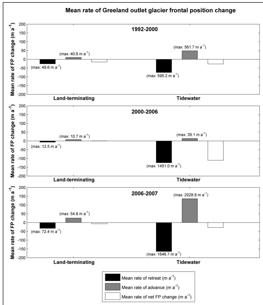
Figure 2.7. Mean rate of Greenland outlet glacier frontal position change ( \text{m a}^{-1} ) grouped according to terminus type. The mean rate of retreat, advance and net frontal position change were calculated for land-terminating and tidewater glacier termini and are shown in the bars above. Values were calculated for three time periods (1992–2000, 2000–2006 and 2006–2007) and maximum rates of retreat/advance are given in brackets above the corresponding bar. Mean values are calculated from a sample of 139 (1992–2000), 169 (2000–2006) and 154 (2006–2007) tidewater glaciers, and 10 (1992–2000), 14 (2000–2006) and 13 (2006–2007) land-terminating glaciers. Glaciers terminating in ice shelves were excluded from the analysis, as data were only available from three glaciers for 1992–2000 and 2000–2006 and no data were available for 2006–2007. Source: Data provided by T. Moon, 2011 (Moon and Joughin, 2008).
