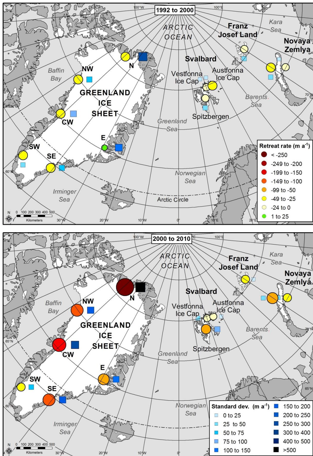
Figure 6.3 Mean regional marine-terminating outlet glacier retreat rates for the periods 1992-2000 and 2000-2010. Symbol colour shows the magnitude of glacier retreat (yellow through red circles) and standard deviation in retreat rates (blue squares) between 1992 and 2010. In both cases, symbol size shows the R^2 value of the relationship: a larger symbol represents a larger R^2 value and therefore the trend line better fits the data. The spatial extent of the GrIS regions are shown in Figure 1 and follow moon and Joughin (2008).
