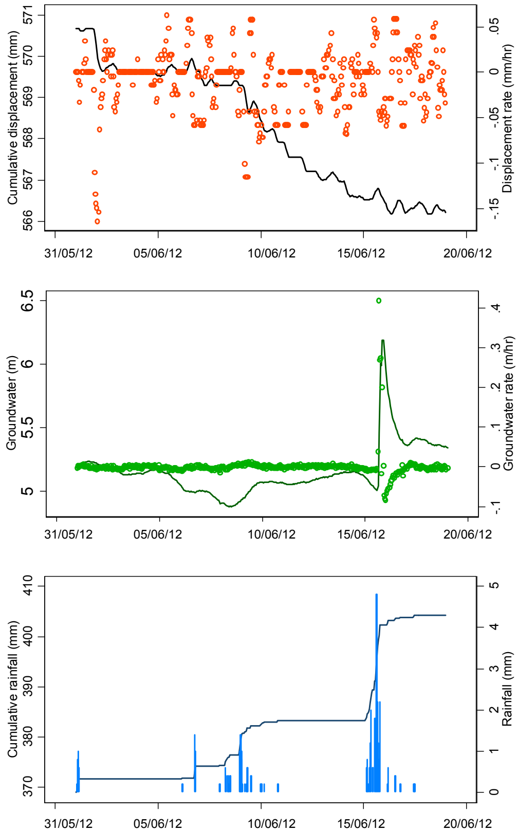
Figure A.10 Monitoring results at the Upgang Landslide (Period 10). No movement between 01 st and 19 th June 2012 shows about -4 mm in cumulative displacement with a maximum displacement rate of 0.06mm/hr. Groundwater fluctuated between 4.88 and 6.19m with a high groundwater rate of 0.42 m/hr. The total rainfall was 47mm with a maximum rate of 4.8mm/hr during a 35-hour wet period.
