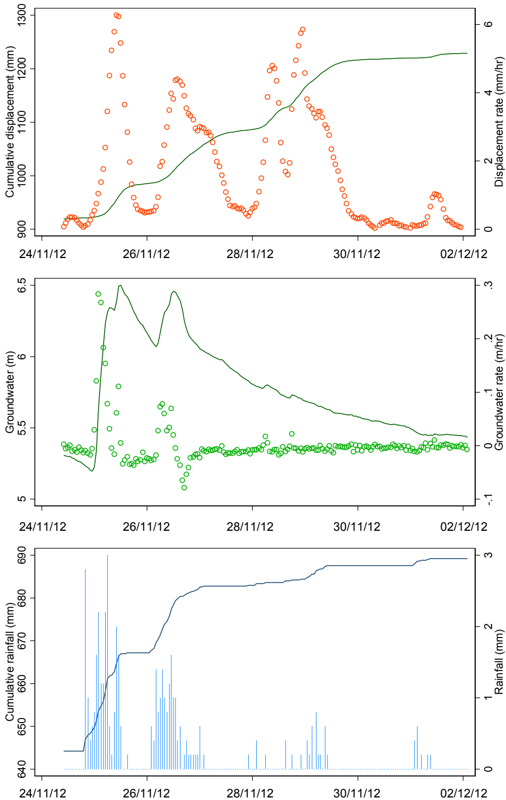
Figure A.19 Monitoring results at the Upgang Landslide (Period No.19). Accelerated movement between 24 th November and 02 nd December 2012 shows about 309.6 mm in cumulative displacement with a maximum displacement rate of 6.272 mm/hr. Groundwater fluctuated between 5.2 and 6.5 m with a high groundwater rate of 0.28 m/hr. The total rainfall was 45 mm with a maximum rate of 3 mm/hr during a 60-hour wet period.
