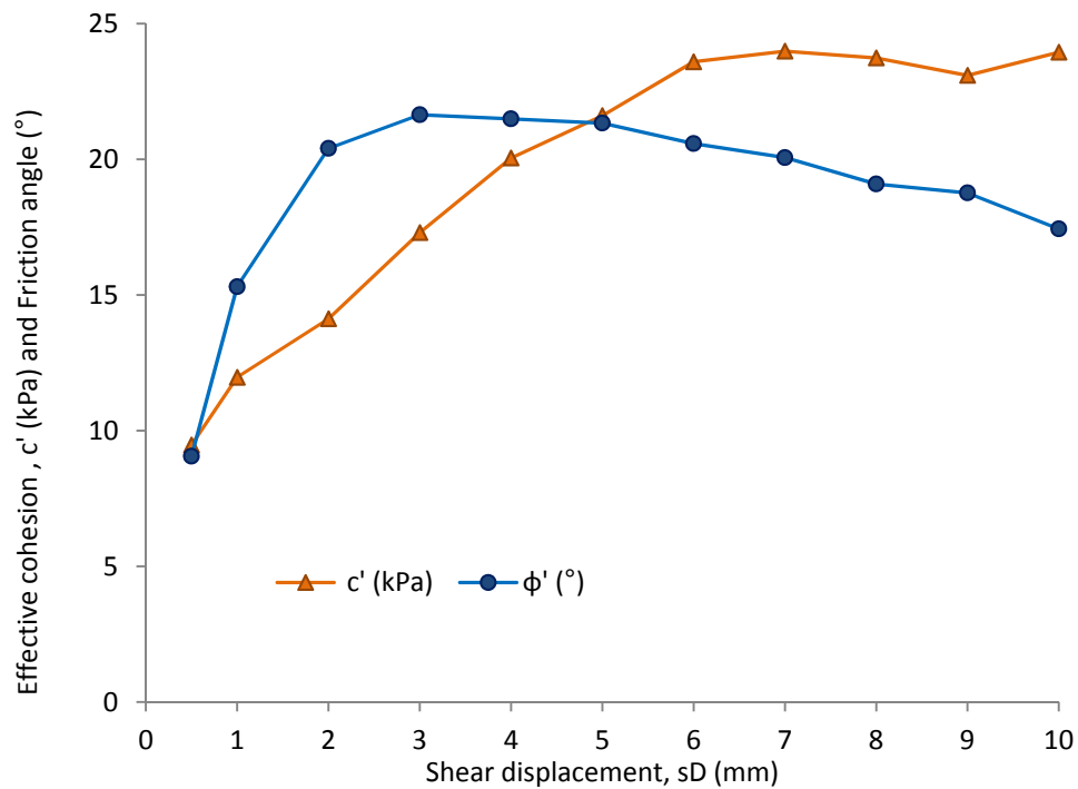
Figure 6.8 Strain development during shearing stage in terms of effective cohesion and frictional angle. Frictional strength increase rapidly at the initial stage of shearing ( \leq 4 mm), followed by decreasing frictional strength toward the end of failure. Conversely, effective cohesion increases dramatically and followed by stabilisation: a) West samples (W02, W03, W04, W05); b) East samples (E02, E03, E04).
