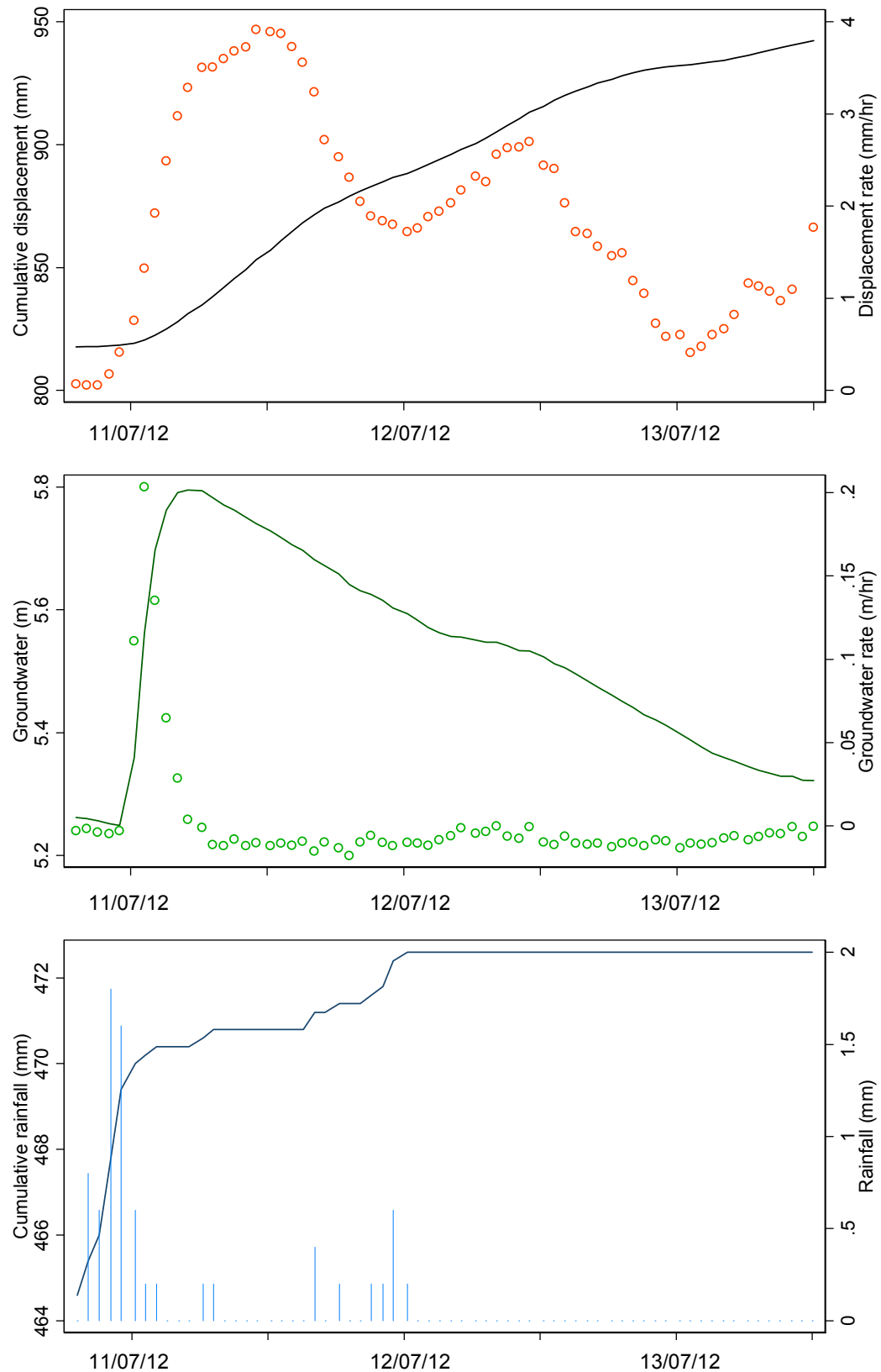
Figure A.15 Monitoring results at the Upgang Landslide (Period No.15). Accelerated movement during 10 th – 13 th July 2012 shows about 124.77 mm in cumulative displacement with a maximum displacement rate of 3.91 mm/hr. Groundwater fluctuated between 5.25 and 5.80 m with a high groundwater rate of 0.20 m/hr. The total rainfall was 10.2 mm with a maximum rate of 1.8 mm/hr during a 15-hour wet period.
