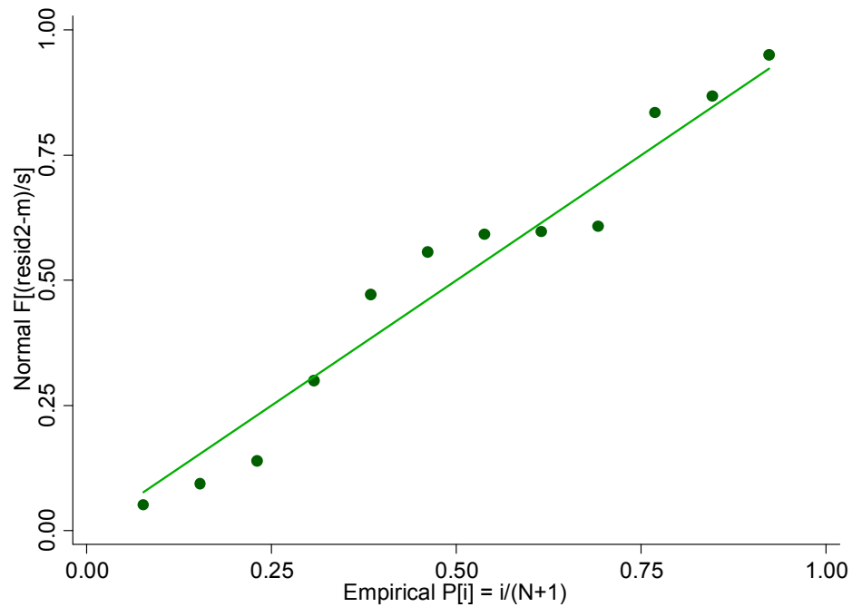
Figure 7.4 Plot of the residuals against the predicted values present a random pattern, so the model is reasonable (a). The normalized probability plot shows distribution of displacement rate nearer to the centre of the distribution (b).
