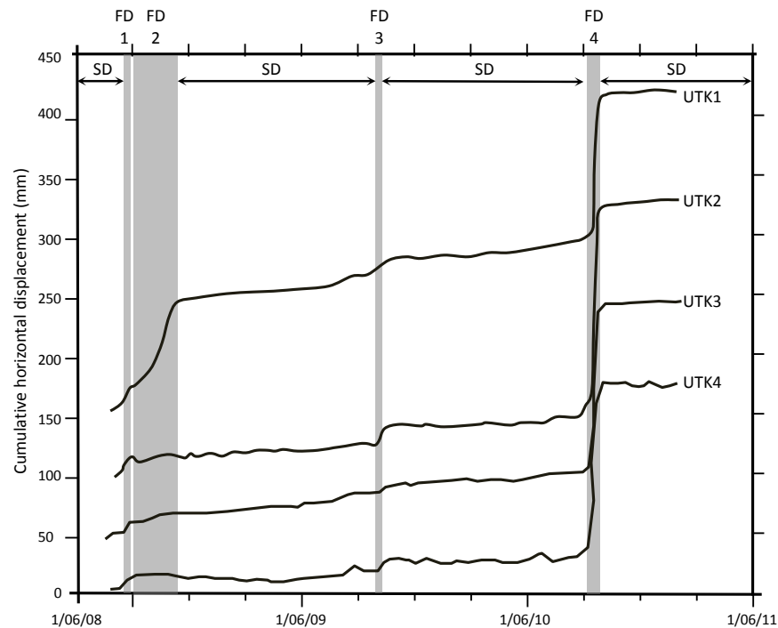
Figure 2.4 Daily filtered cumulative horizontal displacement of cGPS stations located on the Utiku landslide, plotted along their main displacement bearings: FD-fast displacement periods, SD-slow displacement periods. Note: the cumulative displacement cGPS time all originate at zero and have been offset from zero for presentation purpose (redrawn from Massey et al., 2013).
