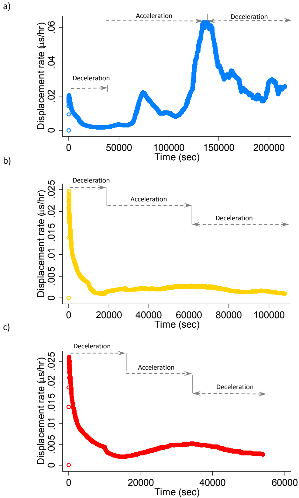
Figure 6.22 Plots of displacement rate over time under reinflation rates of 0.5 (a), 1(b), and 2(c) kPa / hr. Decelerations are found at the initial stage of increasing PWP, followed by accelerations. However, the movements show deceleration toward the end of the reinflation stage.
