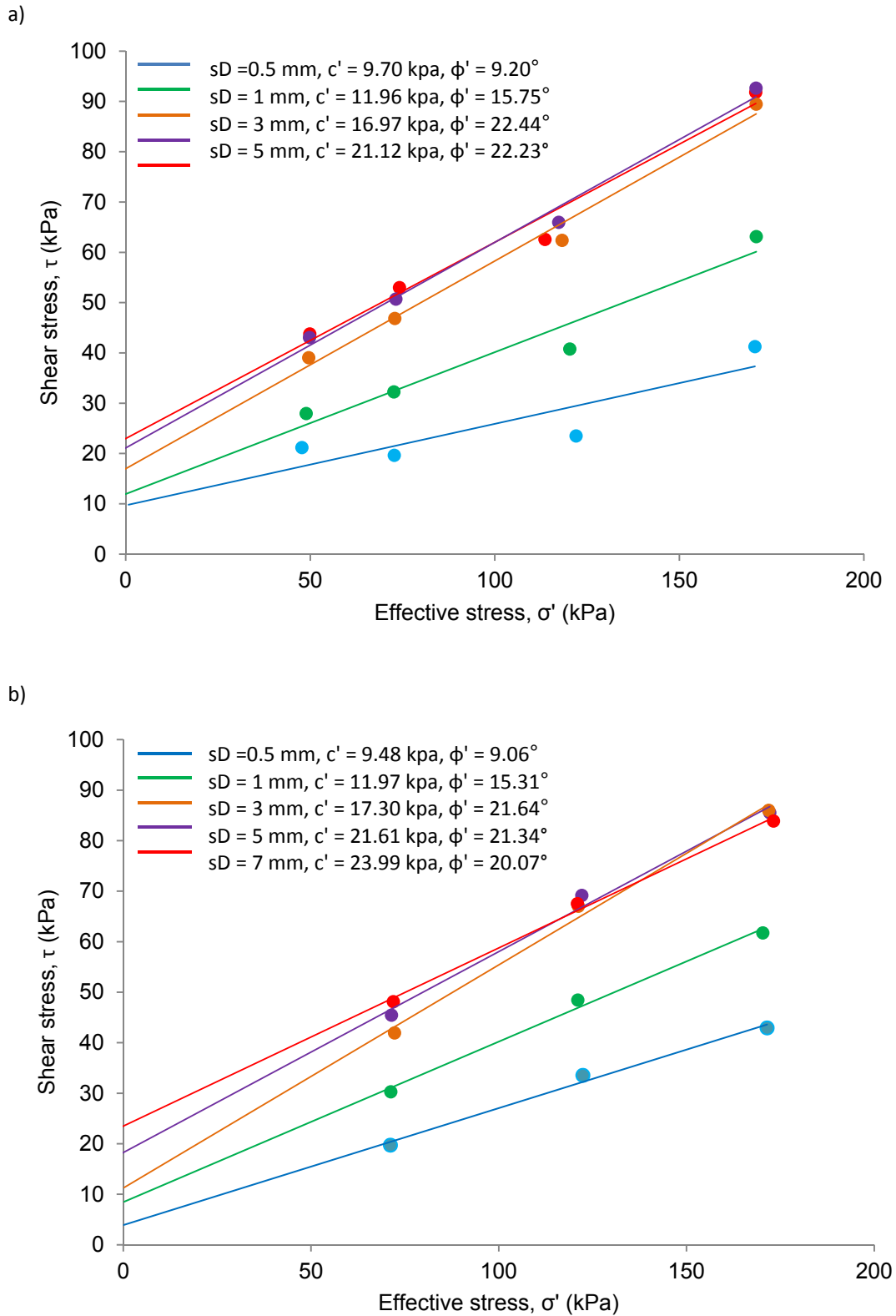
Figure 6.9 Strain development during shearing stage revealed by failure envelopes at equal strains. West sample (a) and East sample illustrated the largely similar constant slopes of \tau_{\max} - \sigma' at 3-7 mm shear displacements.
