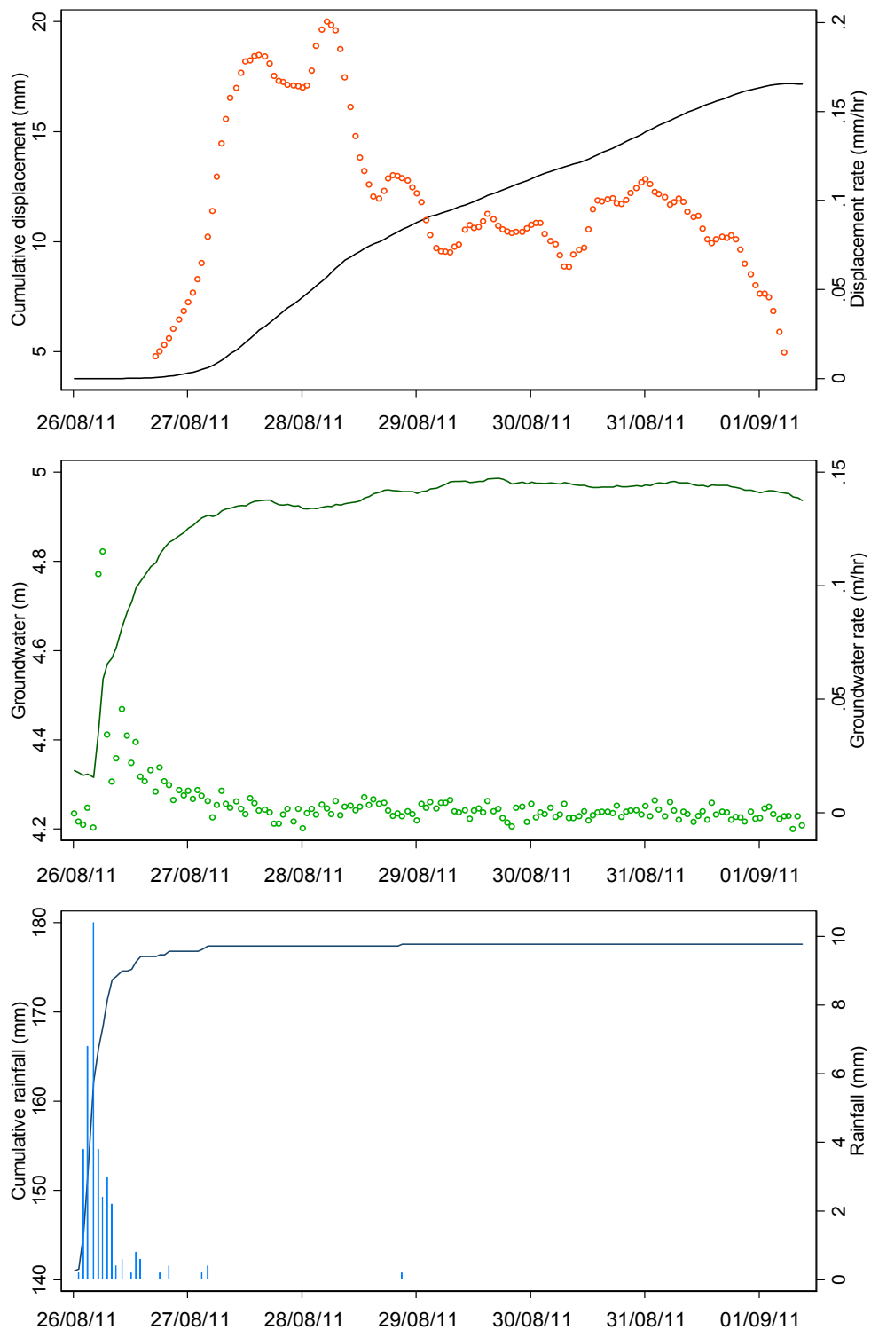
Figure A.2 Monitoring results at the Upgang Landslide (Period 2). Accelerated movement between 26 th August and 01 st September 2011 shows about 13.40 mm in cumulative displacement with a maximum displacement rate of 0.2 mm/hr. Groundwater fluctuated between 4.32 and 4.99 m with a moderate groundwater rate of 0.1 m/hr. The total rainfall was 36.60mm with a maximum rate of 10.40 mm/hr during a 18-hour wet period.
