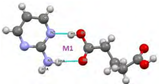
Fig. 1.10 Example of a graph set description of hydrogen bonding motif M1. M1 has a graph set of R_2^2(8) .
