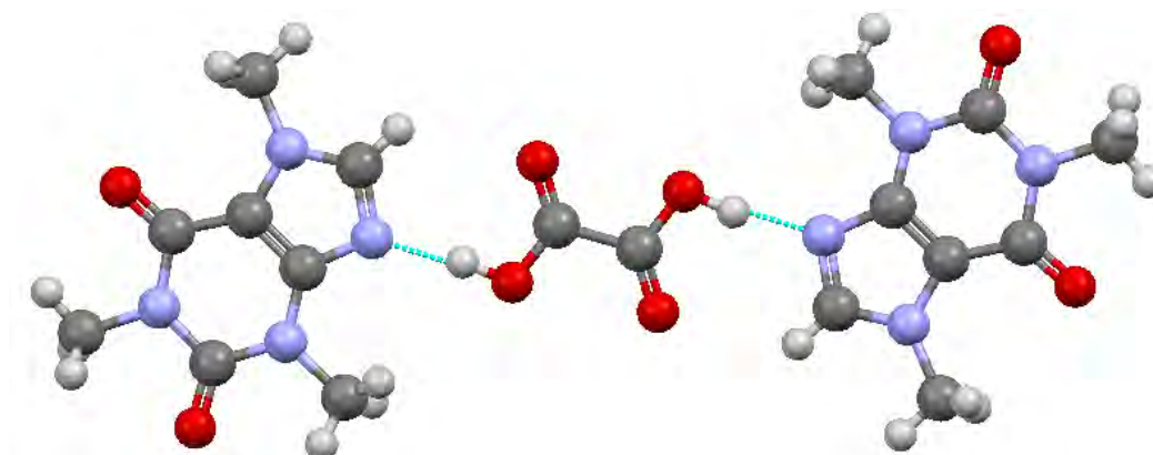
Fig. 5.27 Building motif of caffeine-oxalic acid cocrystal visualised using Mercury.
