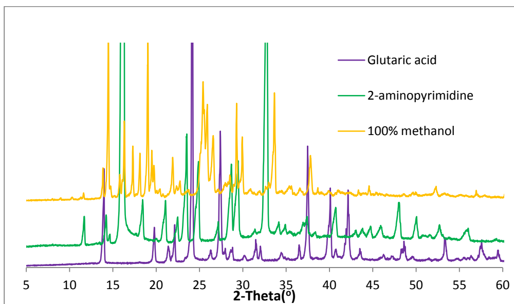
Fig. 6.75 A comparison of 2-aminopyrimidine –glutaric acid (100% methanol) cocrystallisation sample and components pattern.
