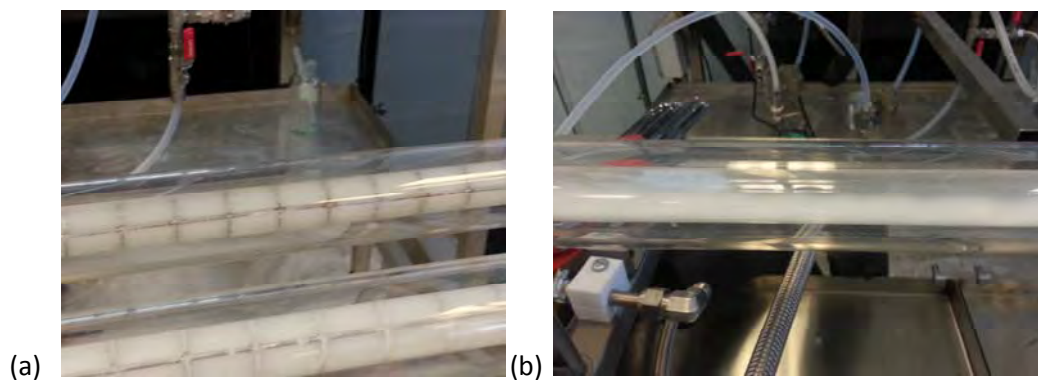
Fig. 2.10 (a) Uniform mixing of slurry in the PPU with baffles. The slurry is uniformly suspended throughout the liquid. (b). Non-uniform mixing of slurry in PPU without baffles. Note the slurry just sits at the bottom of the unit and is not suspended.
