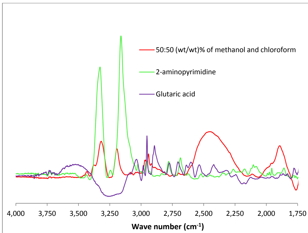
Fig. 6.95 FTIR comparison between 1750 cm -1 and 4000 cm -1 region for 2-aminopyrimidine-glutaric acid (methanol/chloroform) sample.
