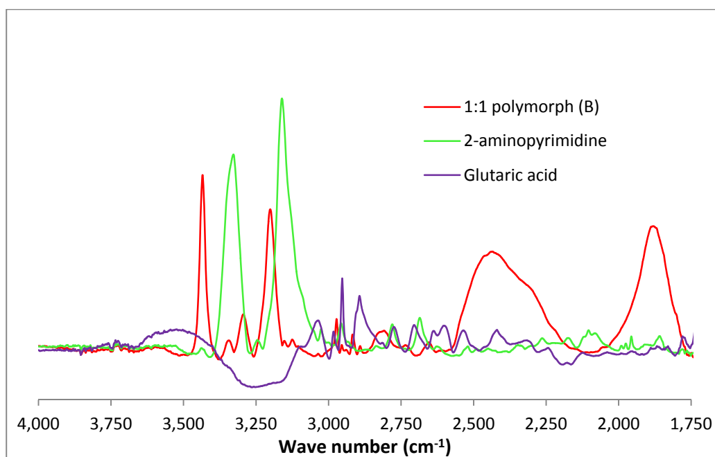
Fig. 6.24 FTIR comparison between 1750 \text{cm}^{-1} and 4000 \text{cm}^{-1} region for B and its cocrystal components.
