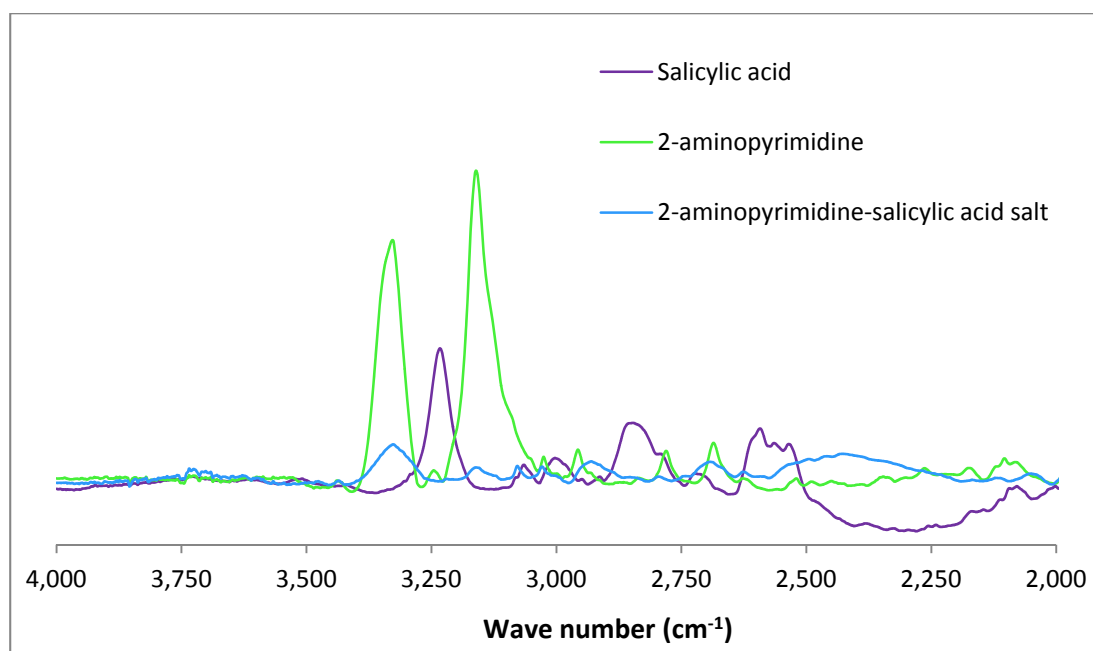
Fig. 5.25 Comparing FTIR spectra for 2-aminopyrimidine-salicylic acid salt between 2000-4000 \text{cm}^{-1} region.
