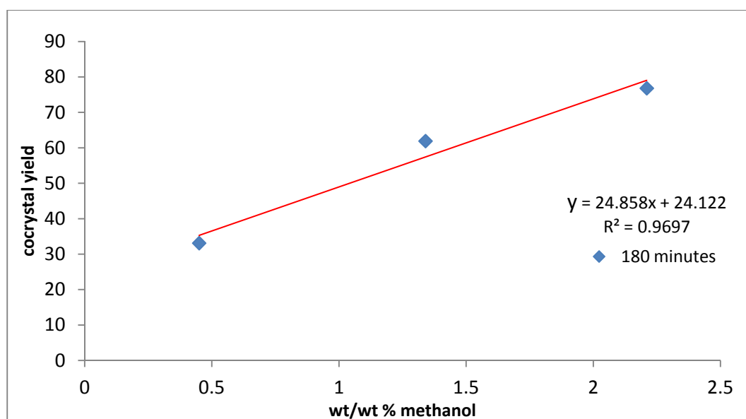
Fig. 4.13 Scatter plot of cocrystal yield against the different ratios of methanol for samples taken after 180 minutes SVC cocrystallisation of caffeine and oxalic acid.
