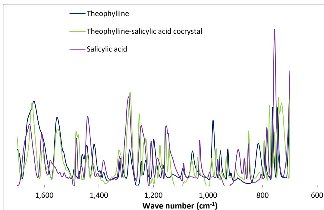
Fig. 5.43 Theophylline-salicylic acid cocrystallisation FTIR spectra comparison between 600 – 1,700 cm -1 region.
