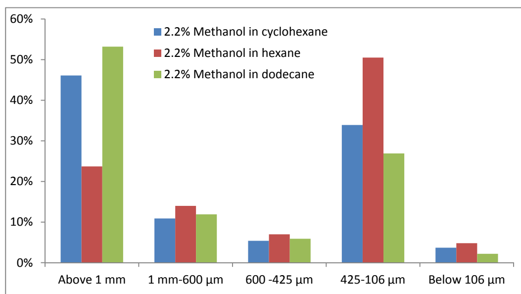
Fig. 4.31 Histogram of particle size distribution for different anti-solvent of caffeine-oxalic acid SVC cocrystallisation experiments.
