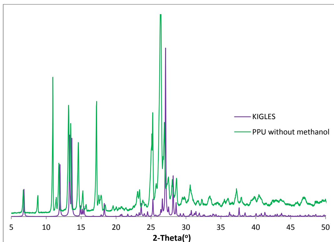
Fig. 5.41 A comparison of PPU cocrystallisation of theophylline-salicylic acid cocrystal without methanol and reference (KIGLES).
