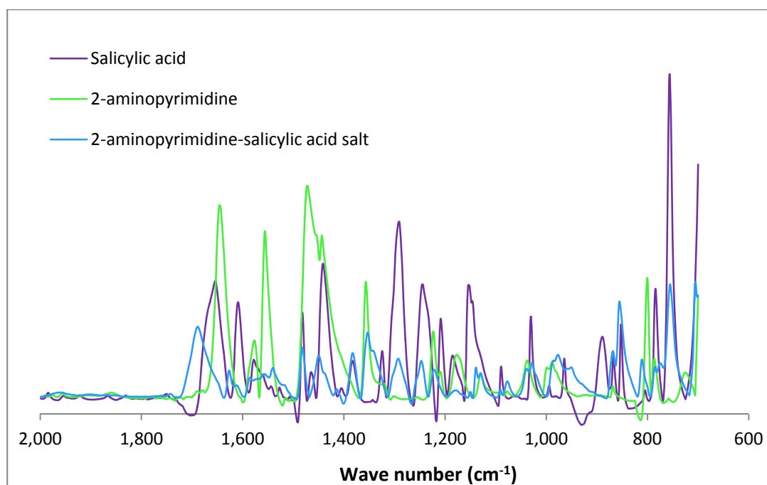
Fig. 5.24 Comparing FTIR spectra for 2-aminopyrimidine-salicylic acid salt between 600 – 2000 \text{cm}^{-1} region.
