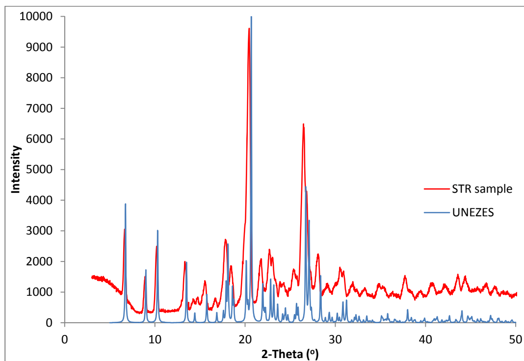
Fig. 5.14 Comparing PXRD pattern for carbamazepine-nicotinamide cocrystal from STR experiment with reference (UNEZES).
