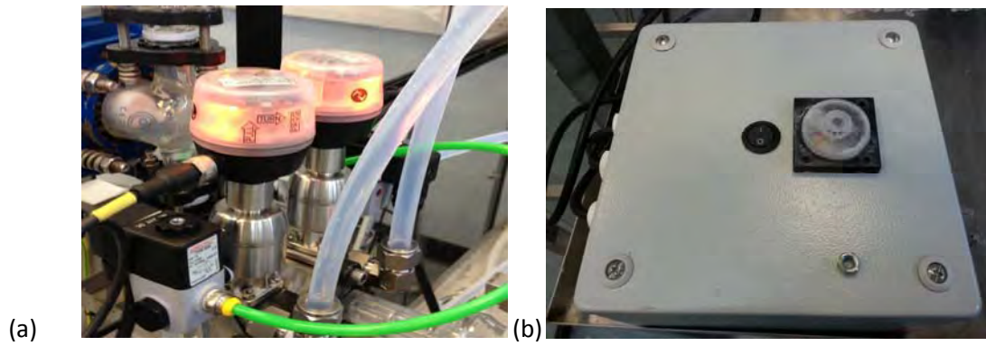
Fig. 2.8 (a) Pneumatic valves for simultaneous slurry dousing from both holding vessels. The two green tubes are the air-lines used for controlling closing and opening of each valve. The red light indicates the valves are shut, which changes to green when the valves are open. (b) Pneumatic valve control box with two dials. The inner dial controls the time delay between valve openings and the outer dial controls how long the valves are opened.
