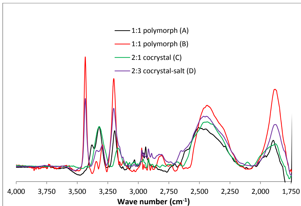
Fig. 6.46. FTIR comparison between 1750 \text{cm}^{-1} and 4000 \text{cm}^{-1} region.
