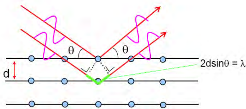
Fig. 2.12 Illustration of Bragg's law 1 .
