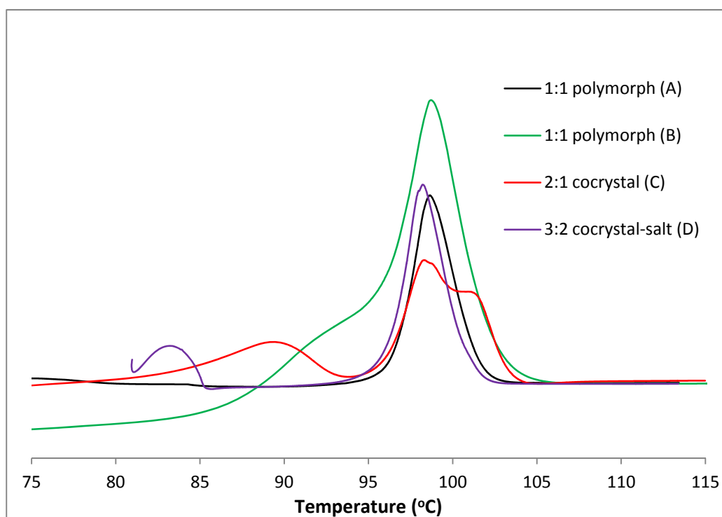
Fig. 6.47 DSC thermogram of all 2-aminopyrimidine-glutaric acid cocrystals.
