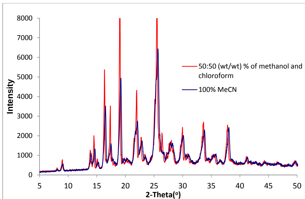
Fig. 6.93 Comparing PXRD of 2-aminopyrimidine-glutaric acid cocrystal PXRD samples from 50:50 methanol /chloroform and sample from 100% acetonitrile.
