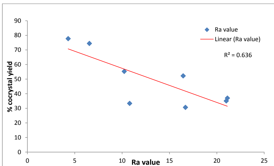
Fig. 4.20 Plot of Ra values against cocrystal yield.
