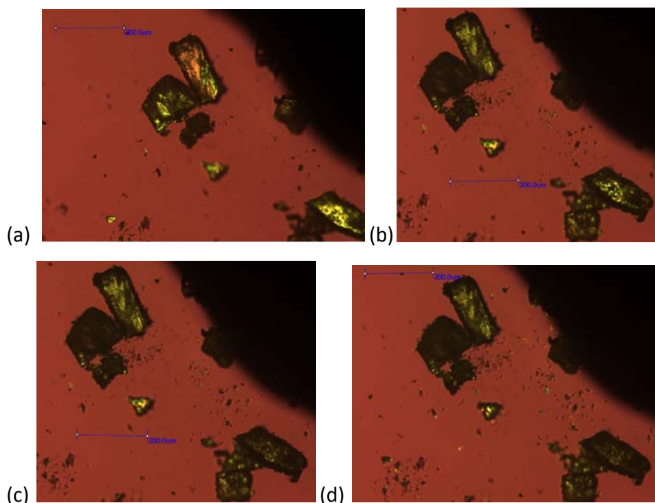
Fig. 6.53 Microscope images of 1:1 polymorph ( A ) of 2-aminopyrimidine-glutaric acid cocrystal. (a) at 25°C, (b) at 73.2°C, (c) at 73.8°C and (d) at 79°C. Pictures show crystals of A , at the top and bottom of the picture goes from bright to a dark crystals as temperature is increased. A transformation at elevated temperature does not go through a melt stage.
