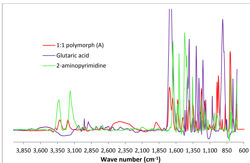
Fig. 6.15 Comparing FTIR spectra for A with glutaric acid and 2-aminopyrimidine.
