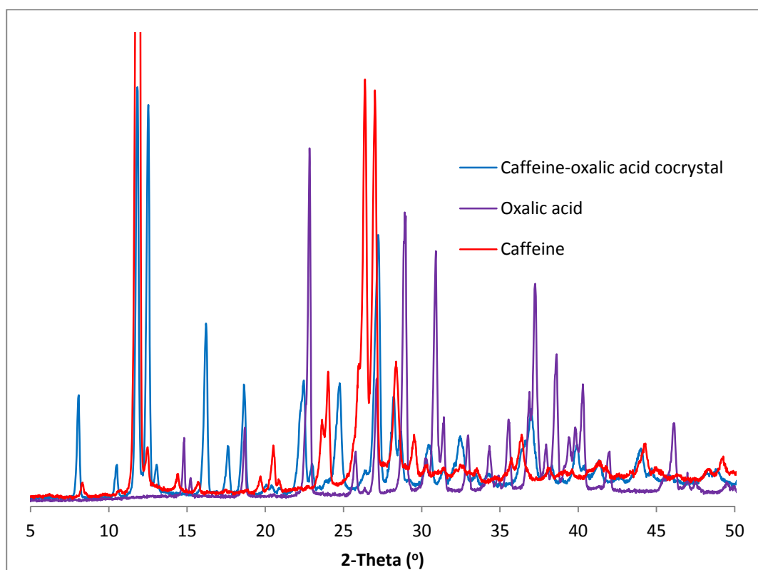
Fig. 3.18 Comparison of PXRD pattern of caffeine, oxalic acid and caffeine-oxalic cocrystal.
