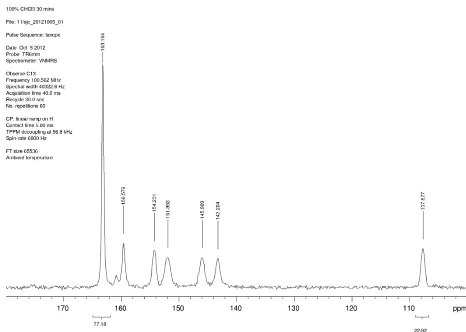
Fig. 3.31 ^{13}\text{C} CP/MAS spectra of the caffeine-oxalic acid cocrystal precision test sample
