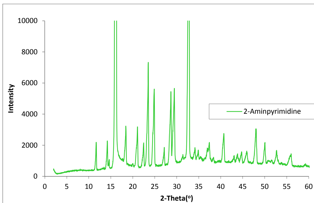
Fig. 6.3 PXRD pattern for commercial sample of 2-aminopyrimidine.
