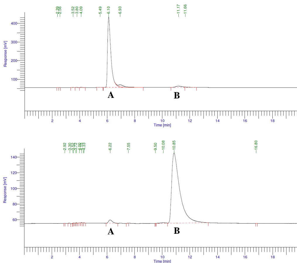
Figure 4.11: Chiral HPLC traces of ( R )- and ( S )-[Eu.L 34 ] (bottom and top respectively) run on a CHIRALPAK-ID column (MeOH, 1 mL min -1 , λ = 268 nm, 290 K).
