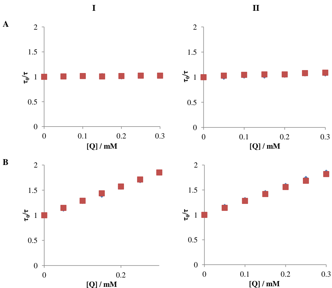
Figure 4.19: Comparison of the variation in emission lifetime as a function of [\text{Co.L}^{38}] (I) and [(R)\text{-Co.L}^{37}] (II) for (R)- (red) and (S)- (blue) [\text{Ln.L}^{34}] (A = \text{Eu}^{3+} ; B = \text{Tb}^{3+} ) (295 K, pH 7.4, 0.1 M HEPES, 0.1 M NaCl, 20 \mu\text{M} complex).
