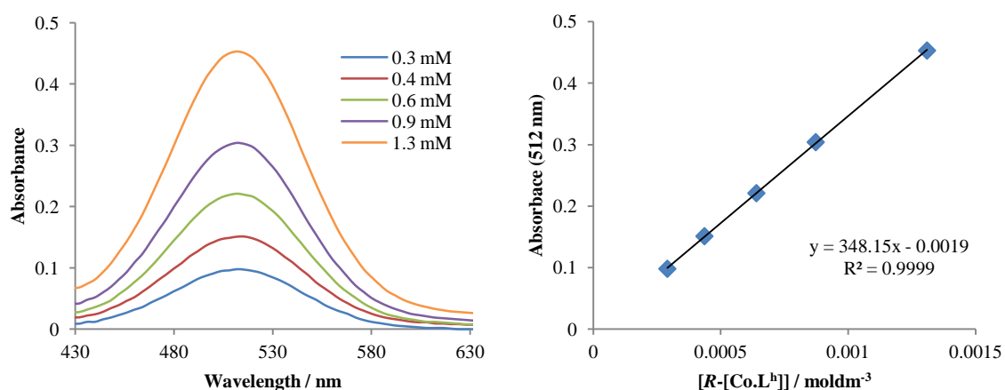
Figure 4.15: Absorption spectra recorded for five aqueous solutions of (R) -[Co.L 37 ] at differing concentrations (left) shown alongside a plot of the absorbance at 512 nm versus complex concentration.
