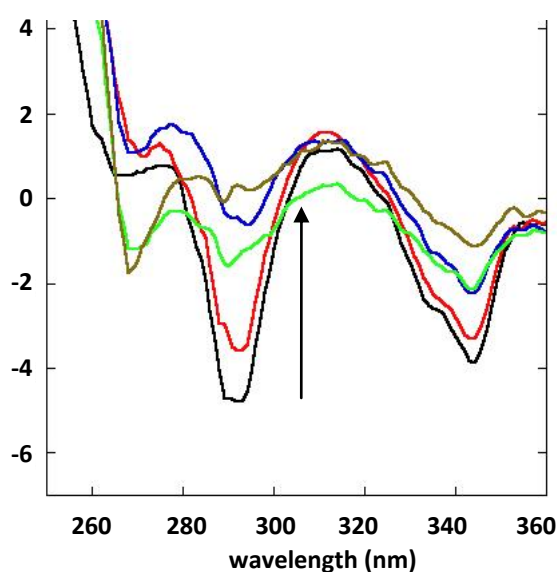
Figure 2.15: Variation in the induced ECD spectrum of [\text{Eu.L}^{22}(\text{OH}_2)]^+ (21 \mu\text{M} ) in the presence of 1 equivalent of \alpha_1 -AGP upon addition of CPZ (up to 1.25 equivalents).
