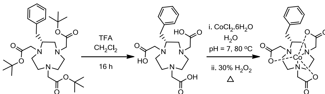
Scheme 4.7: Synthetic pathway for the preparation of (R) - [\text{Co.L}^{37}] . The overall yield of complex was 16%.
