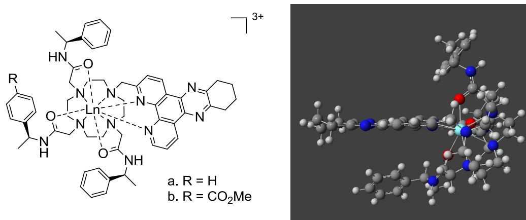
Figure 4.1: DFT calculated structure of (SSS)\text{-}\Delta\text{-}[\text{Y.L}^{20b}]^{3+} , the lower face of the sensitising moiety can be seen to be blocked by a proximate phenyl ring. 136
