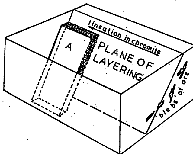
Diagram 2. To show the general relationships of the structures seen in the chromiferous dunite serpentinites of the Saddle Islands, Darvel Bay. The axis of lineation in the Tabular deposits is horizontal; and the Irregular deposits may lie at any angle in the massive dunite serpentinite.
