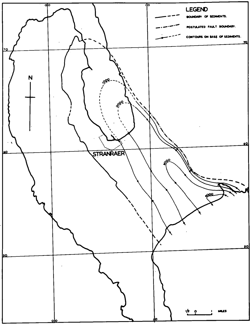
FIGURE 7 APPROXIMATE DEPTH CONTOURS OF STRANRAER SEDIMENTARY BASIN CALCULATED FOR A DENSITY CONTRAST OF 0.4 GM/CM 3 .
