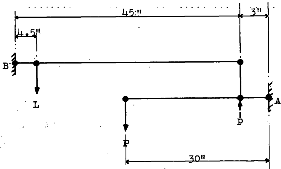
FIG.7.1. WORKING PRINCIPLE OF CREEP MACHINE
