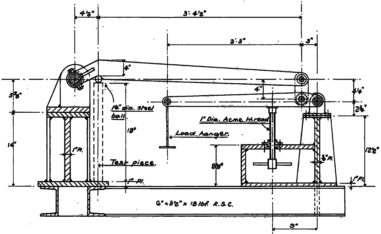
Typical Section Through Creep Machine Frame
