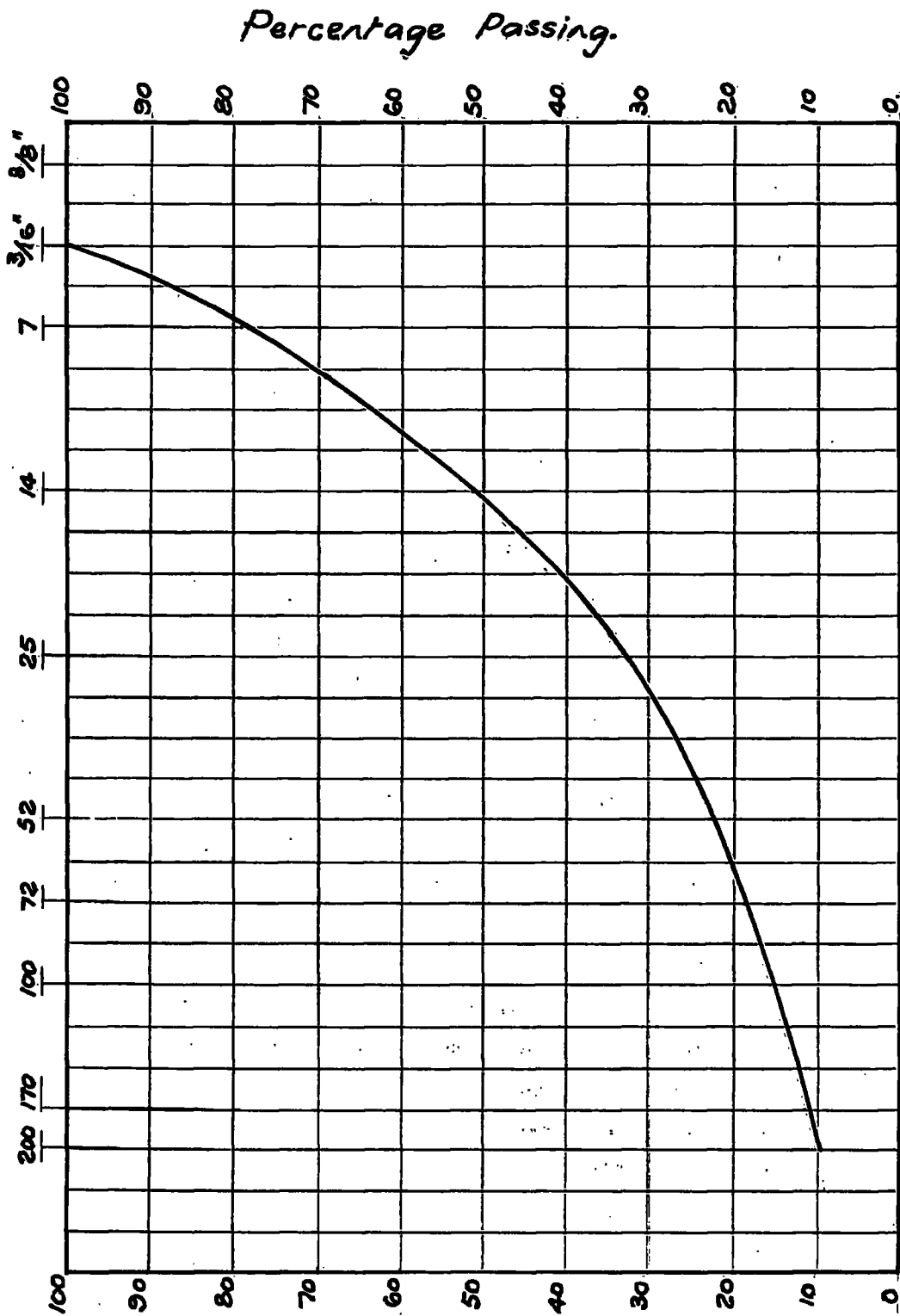
Fig. 3.15. "All-in" Grading of 3/16" aggregate.
