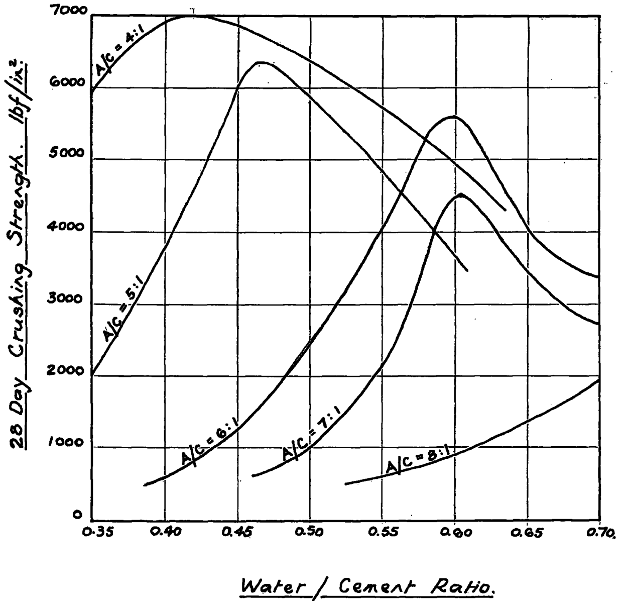
Fig. 3.18. Water / Cement v Crushing Strength for varying aggregate / cement ratios.
