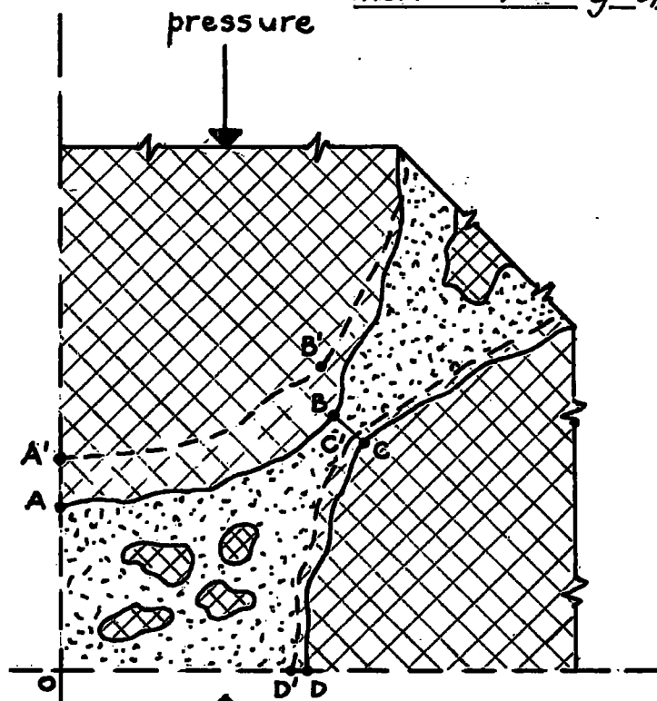
Fig. 2.3. Deformation and forces acting on the mortar filling of a void.
