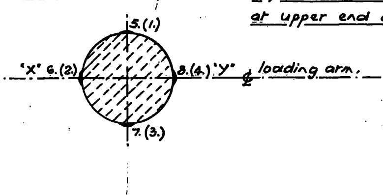
Fig. 7.3. Location of strain gauges. (For strain readings see Table 7.1)
