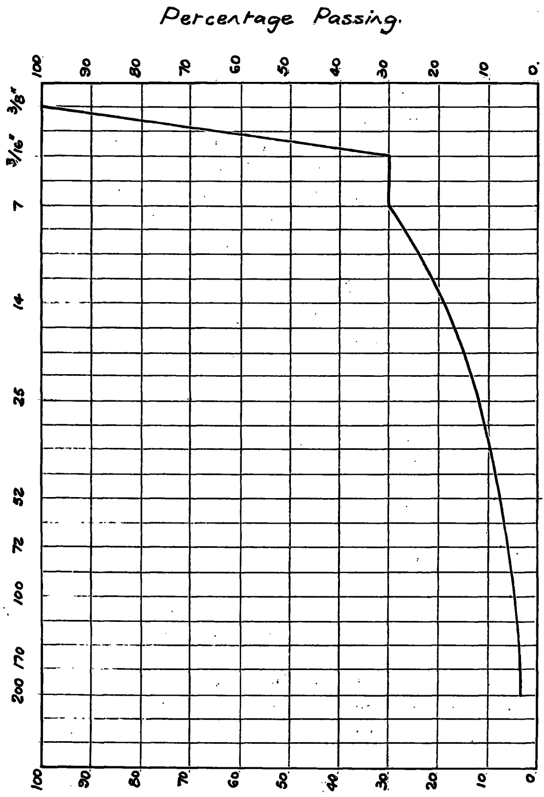
Fig. 3.21. Gap Grading of aggregate for mix "B4"
