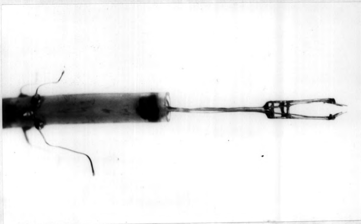
Fig 2.8 The cooling water thermocouples and holder
