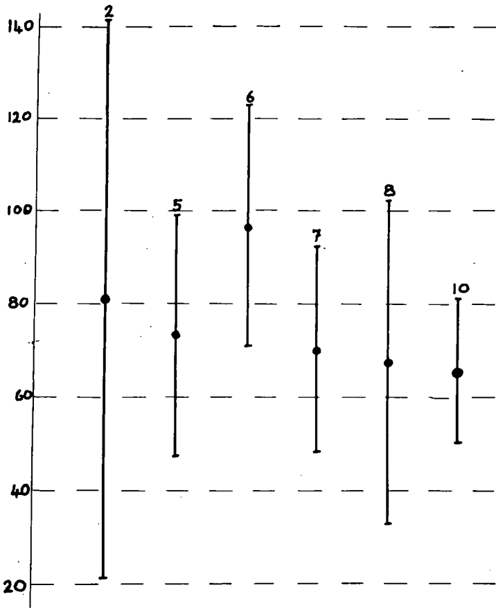
99.7% Confidence interval for a' in equation iv .
