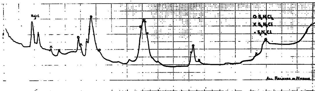
c PRODUCT: S_3N_3Cl_2 + S_3N_3Cl + S_2N_2Cl
