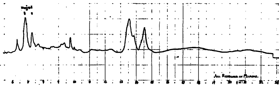
c. EXPERIMENT B. RESIDUE FROM ORANGE AND YELLOW EXTRACTS
