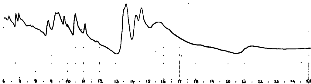
a. EXPERIMENT B. COLOURLESS LEAFLET CRYSTALS
