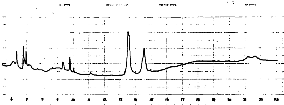
b. EXPERIMENT B. Ph 2 S 2 FROM COLOURLESS EXTRACT
