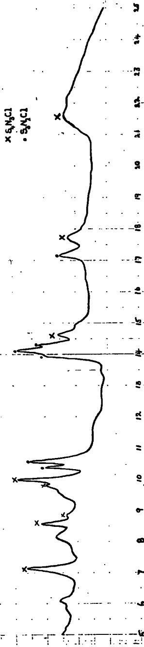
REAGENT: DIMETHYLFORMAMIDE b
