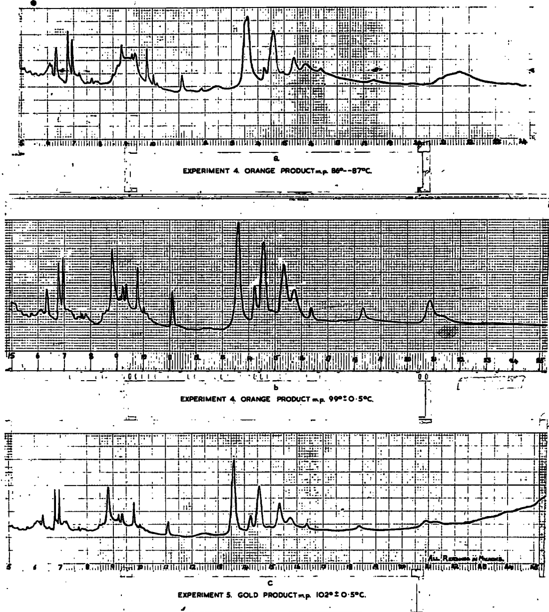
FIG. SP 10. IR. SPECTRA OF PRODUCTS FROM THE REACTION S.N. + PhMgBr
