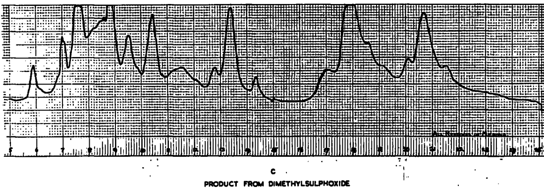
FIG SP 3 I.R. SPECTRA OF PRODUCTS OBTAINED IN THE SOLVENT EXTRACTION OF S, N, Cl
