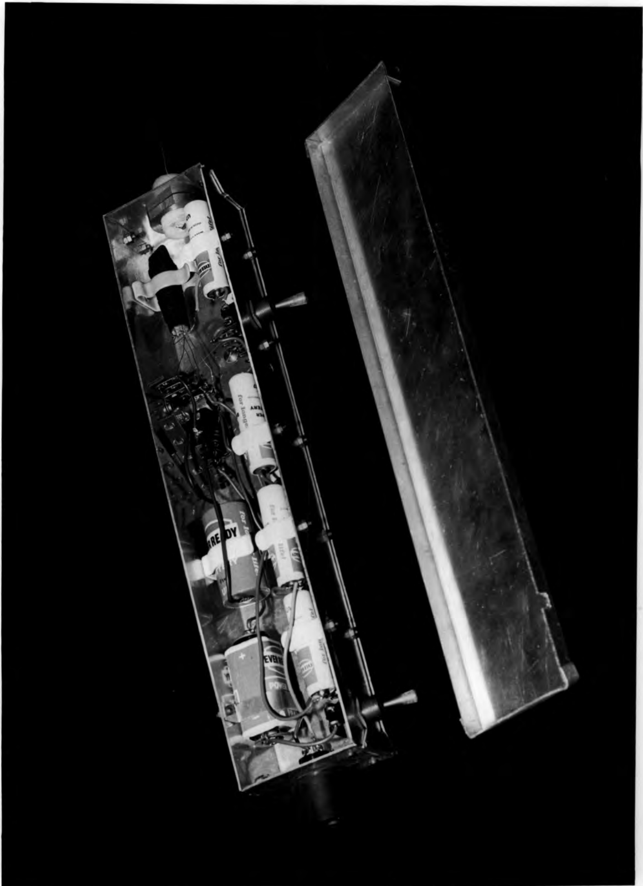
Plate 6 The Passive Probe Head Unit
