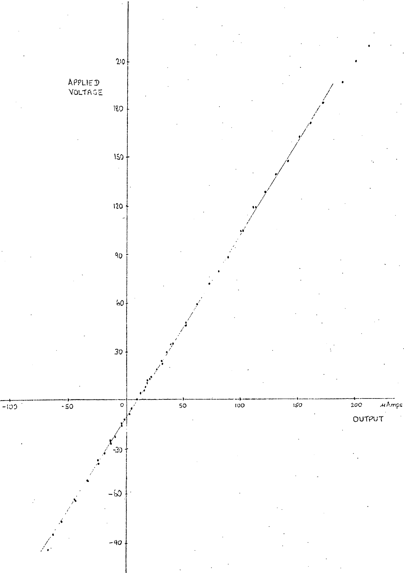
Fig. 12. Calibration Curve of Passive Probe
