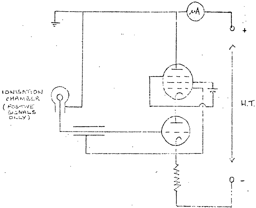
Farmer's Circuit Diagram
