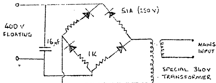
400V POWER SUPPLY
