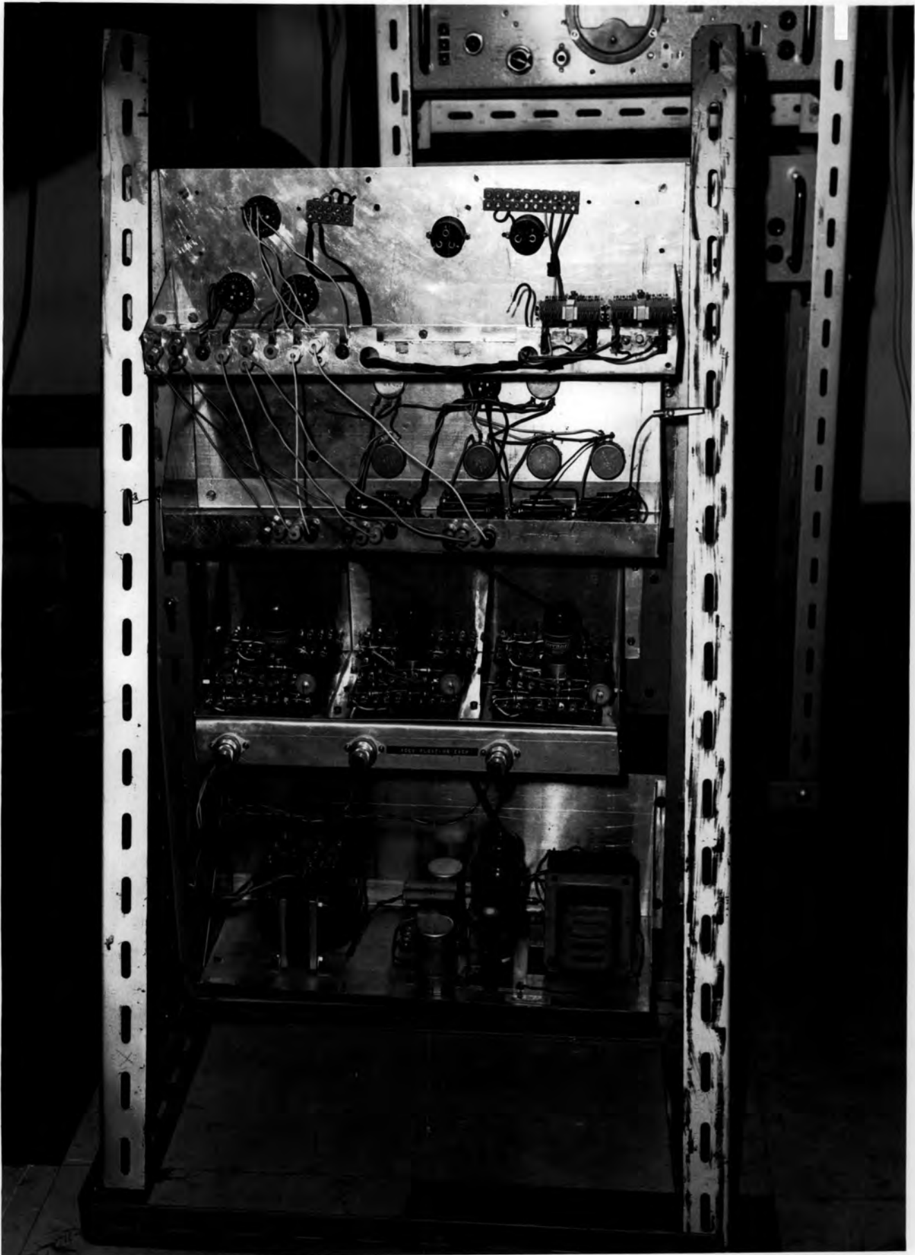
Plate 7b The Passive Probe Ancillary Electronics
