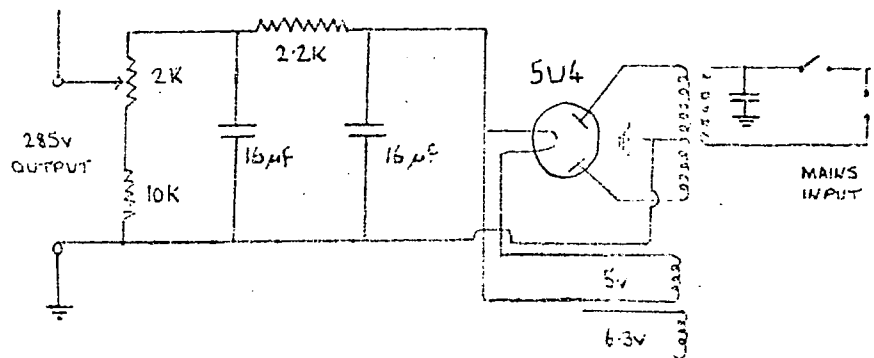
285V POWER PACK
