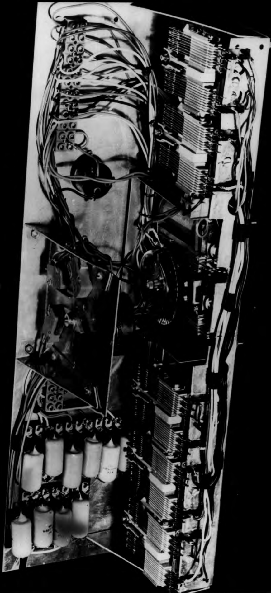
Plate 3 The Timing Mechanism
