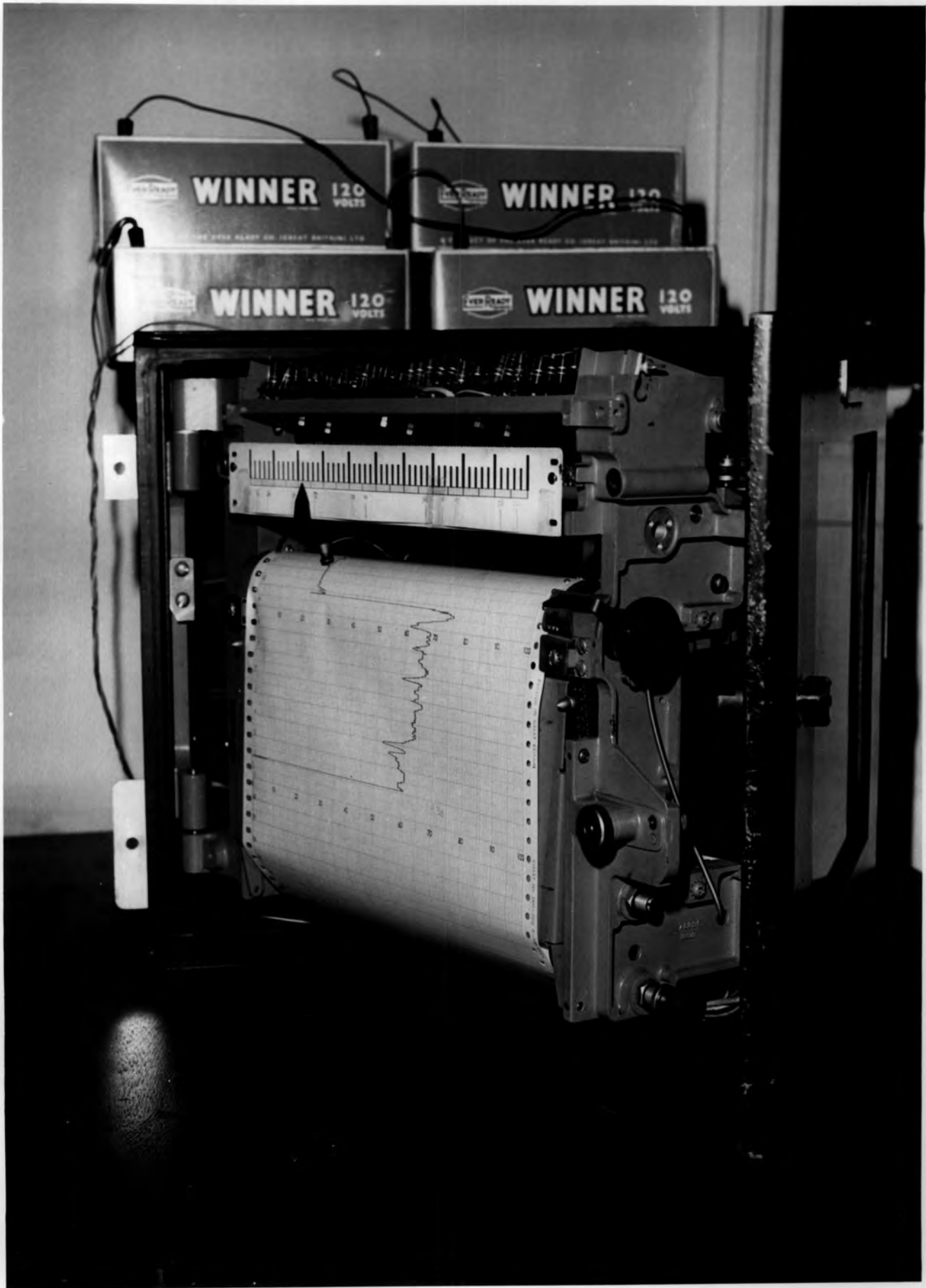
Plate 4 The Potential Balancing Servo Mechanism
